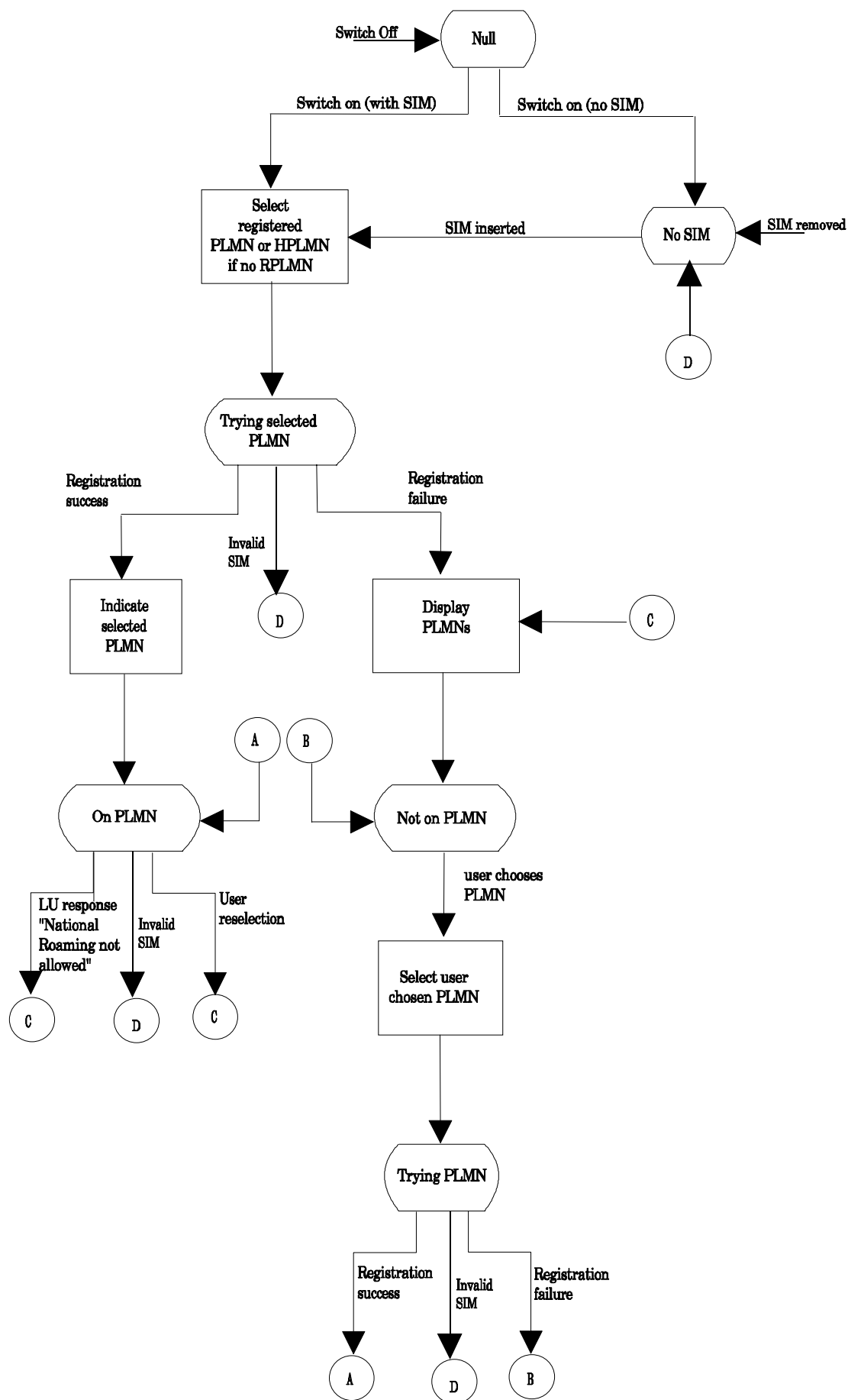
Figure 2b: PLMN Selection State Diagram (Manual Mode)
