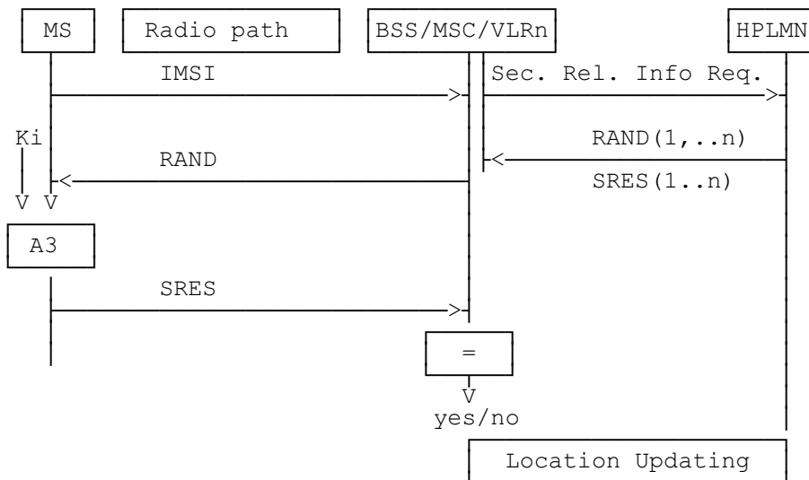
Figure 3.5: Authentication at location updating in a new VLR, using IMSI
