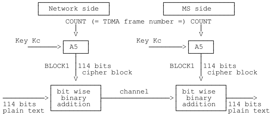
Figure C.2: Deciphering on the MS side
