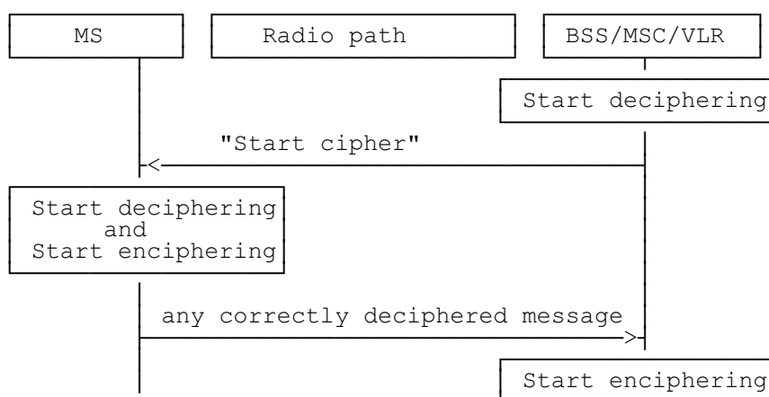
Figure 4.2: Starting of the enciphering and deciphering processes
