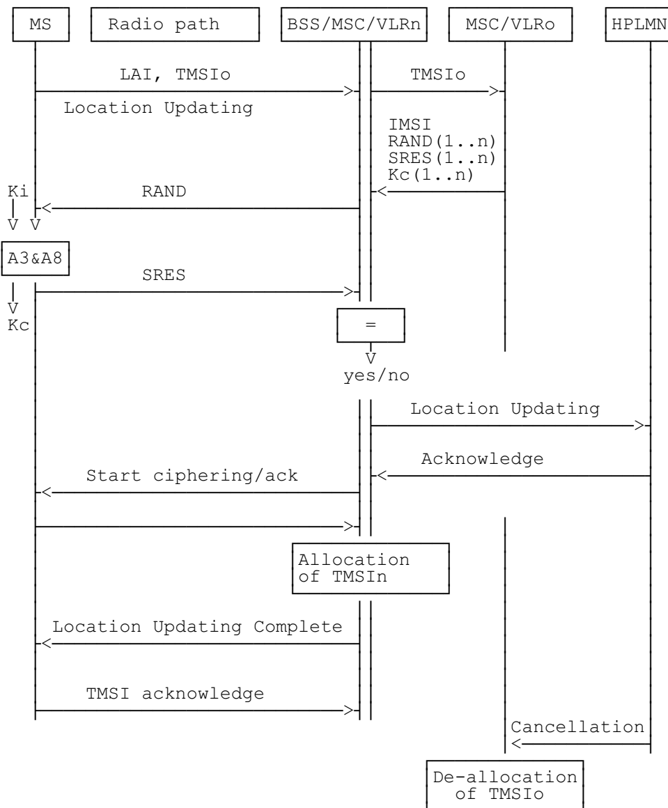
Figure 5.1: Normal location updating procedure
