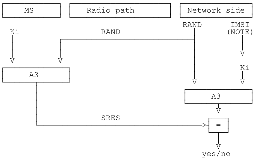
Figure 3.1: The authentication procedure
