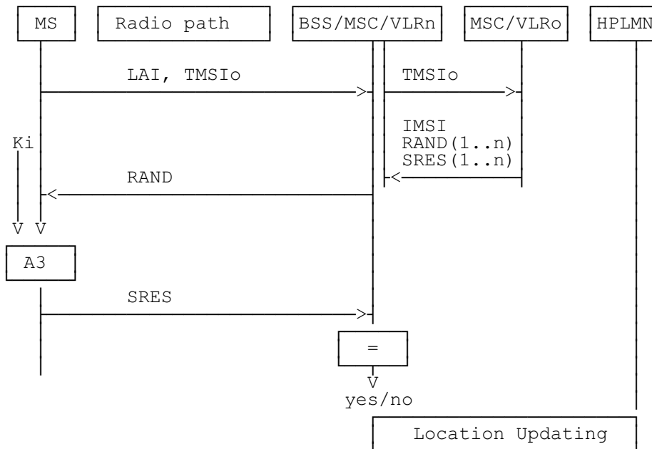
Figure 3.4: Authentication at location updating in a new VLR, using TMSI
