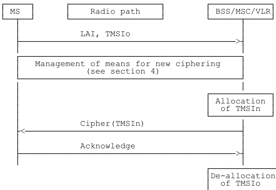
Figure 2.1: Location updating in the same MSC area
