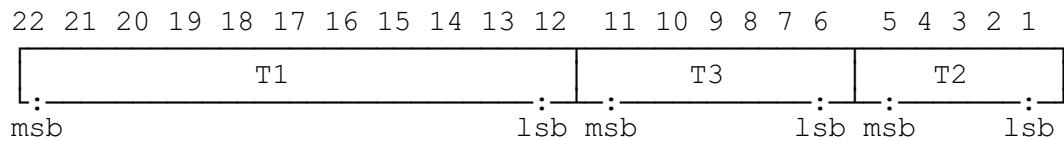
Figure C.1: The coding of COUNT
