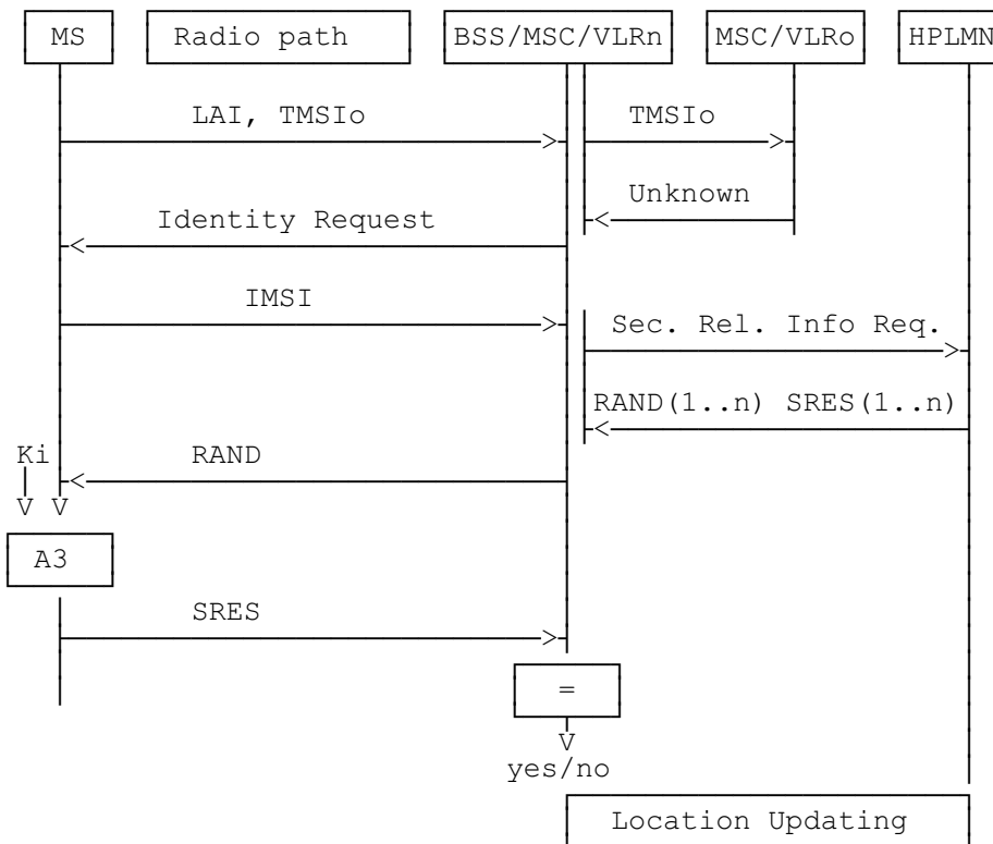
Figure 3.6: Authentication at location updating in a new VLR, using TMSI, TMSI unknown in 'old' VLR
