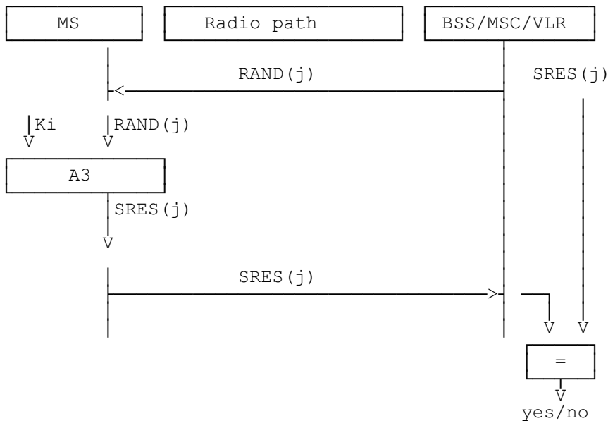
Figure 3.3: General authentication procedure
