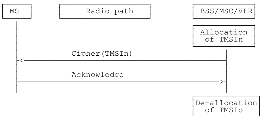
Figure 2.5: Reallocation of a new TMSI
