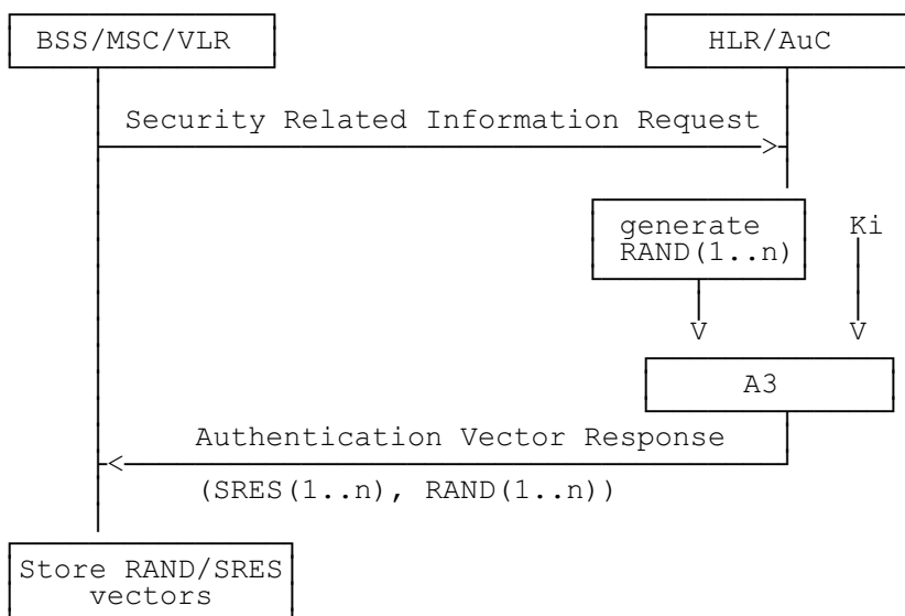
Figure 3.2: Procedure for updating the vectors RAND/SRES
