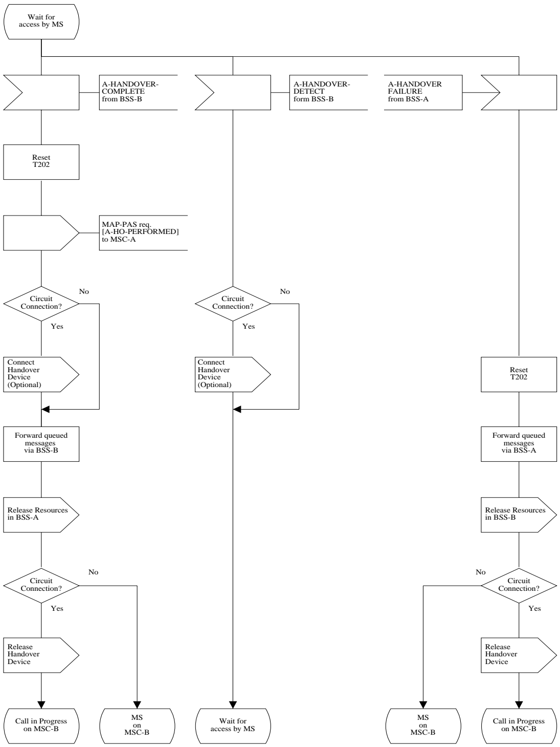
Figure 14 (Sheet 9 of 18): Handover control procedure in MSC-B
