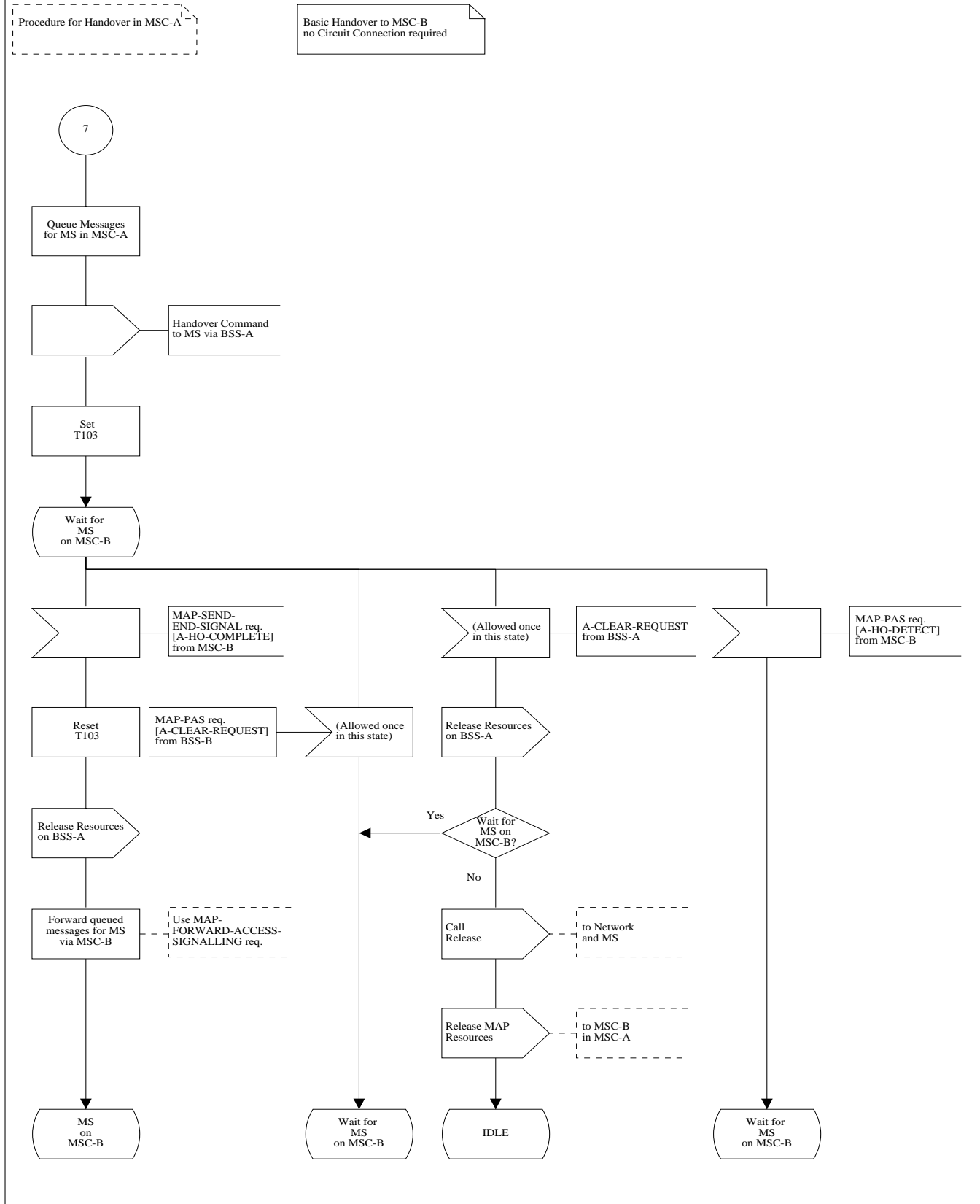
Figure 13 (Sheet 19 of 26): Handover control procedure in MSC-A
