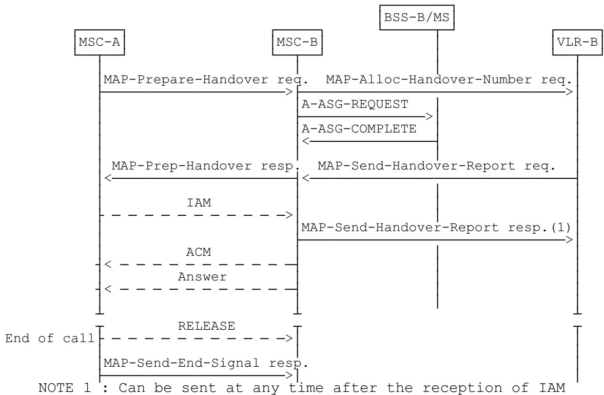
Figure 11: Successful circuit-switched call establishment after a Basic Handover without circuit connection
