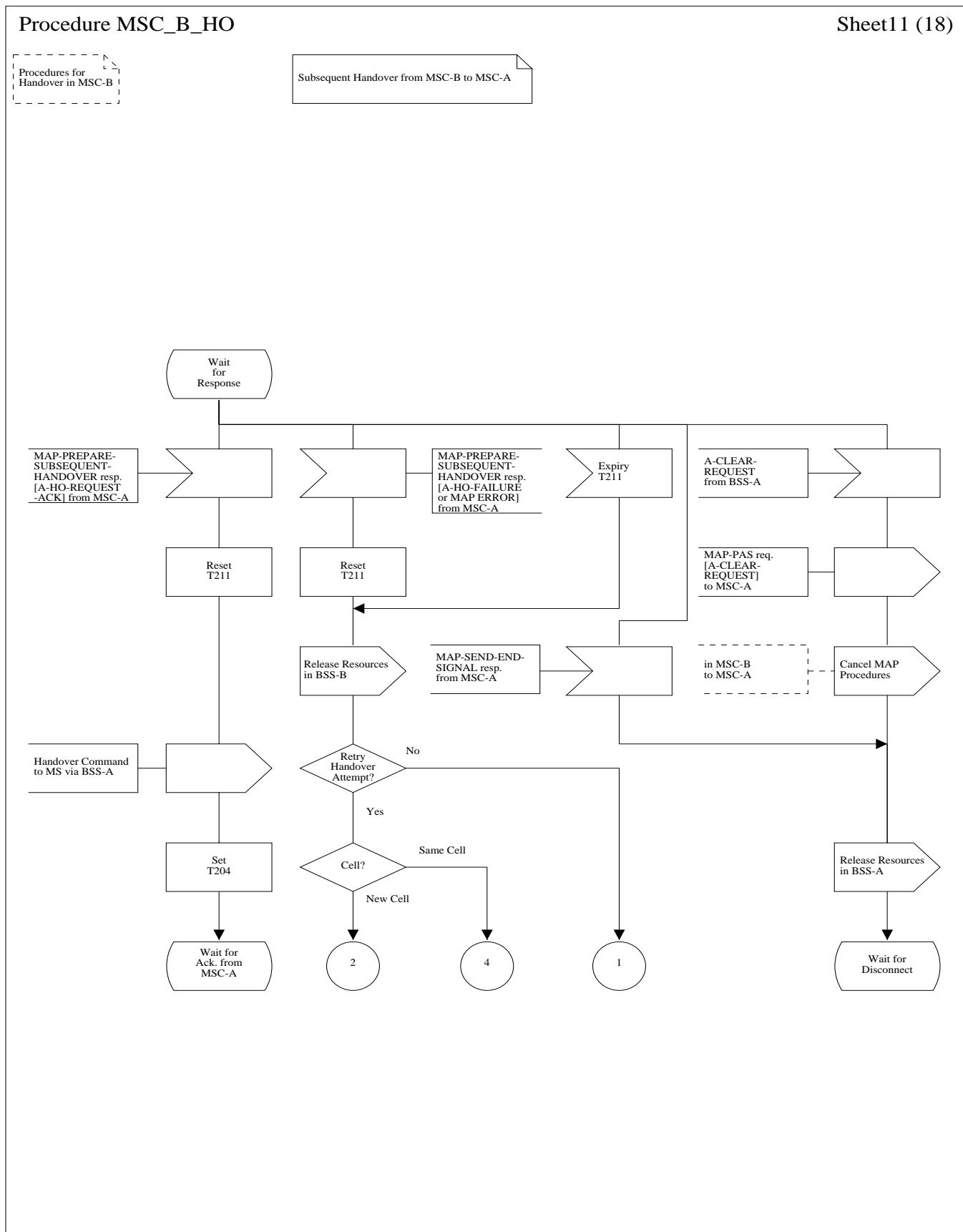
Figure 14 (Sheet 11 of 18): Handover control procedure in MSC-B
