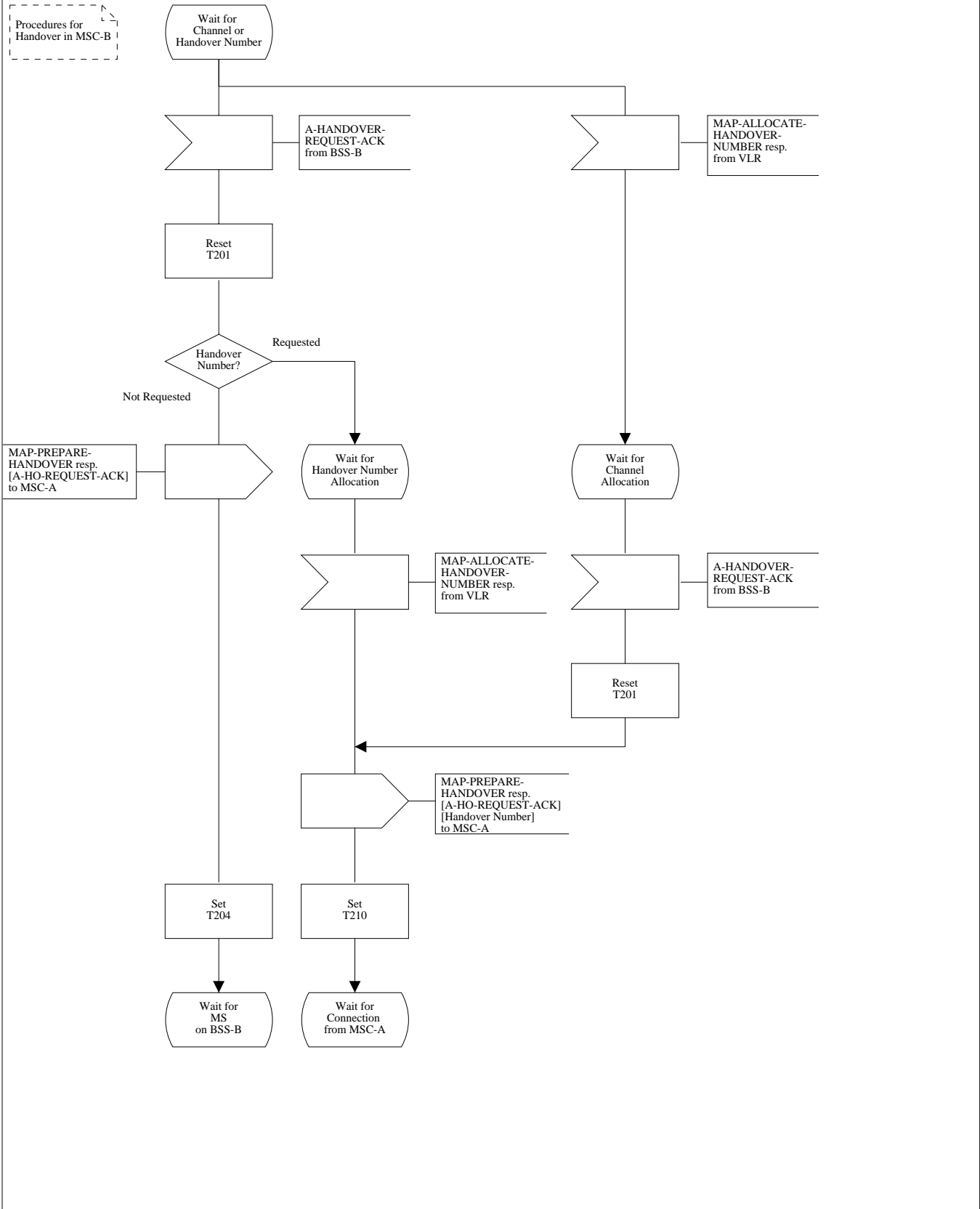
Figure 14 (Sheet 2 of 18): Handover control procedure in MSC-B
