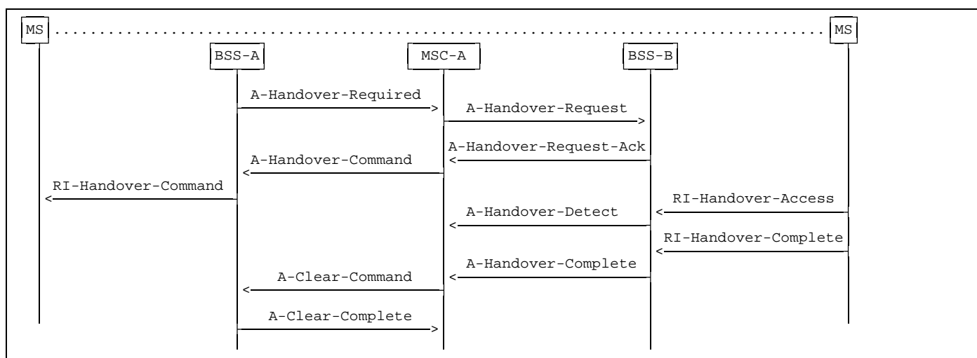
Figure 4: Basic External Intra-MSC Handover Procedure
