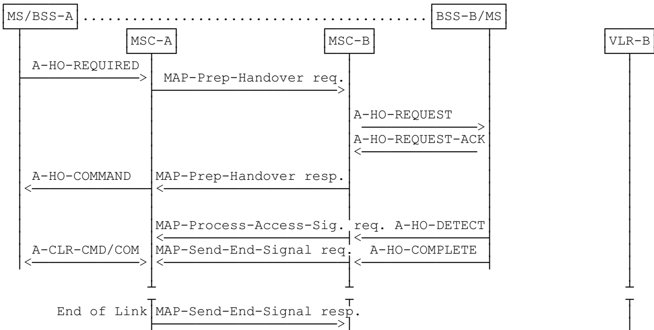
Figure 6: Basic Handover Procedure without circuit connection
