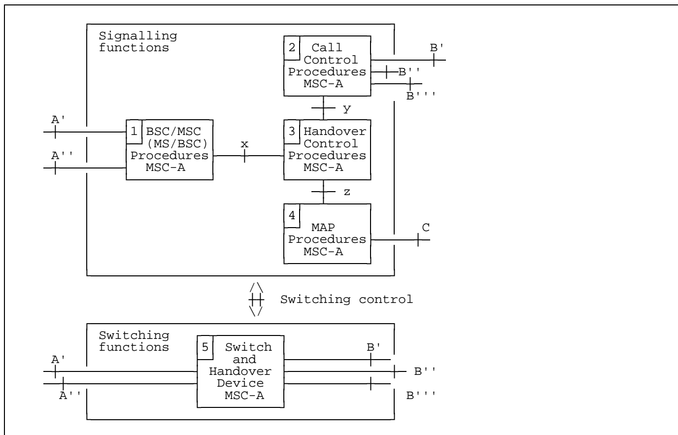
Figure 1: Functional composition of the controlling MSC (MSC-A) for supporting handover
