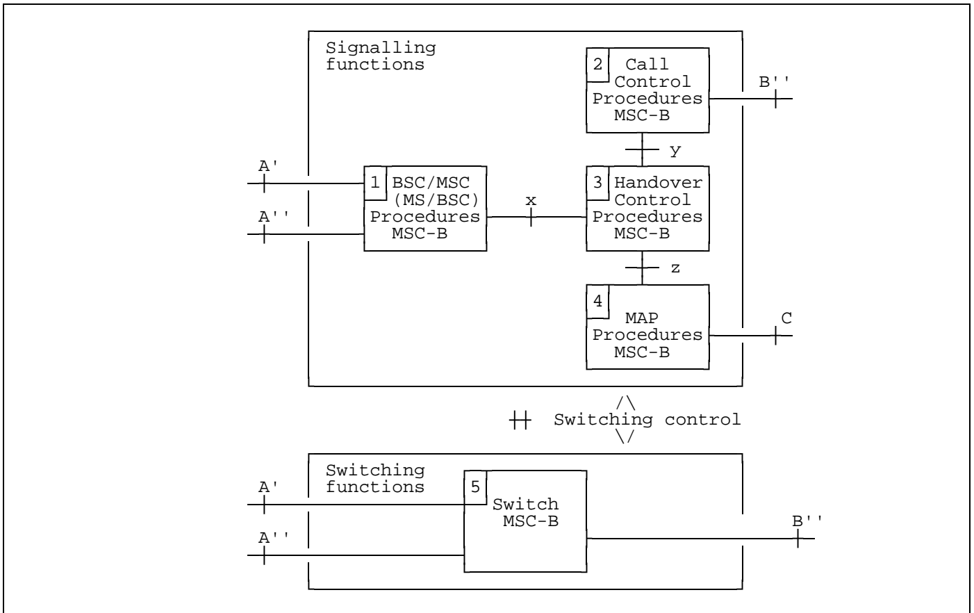
Figure 3: Functional composition of MSC-B for supporting handover
