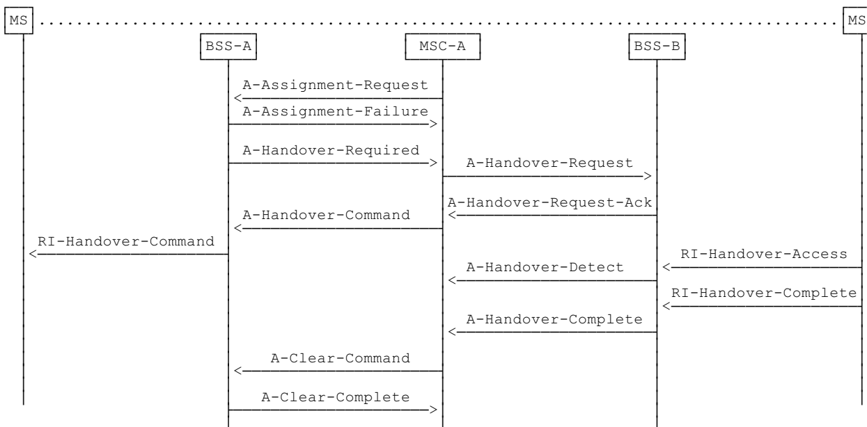
Figure 12: Example of a Directed Retry Intra-MSC Handover Procedure
