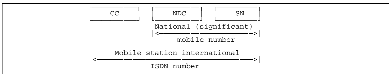
Figure 2: Number Structure of MSISDN
