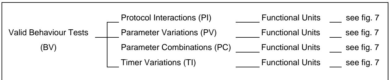
Figure 3: Valid Behaviour Test Group Structure
