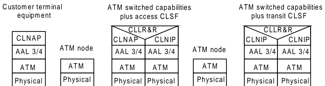
Figure 3: General protocol structure for provision of CBDS in B-ISDN
