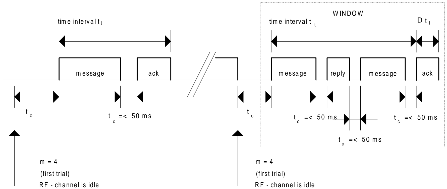
Figure 1: Access protocol sharing data/data
