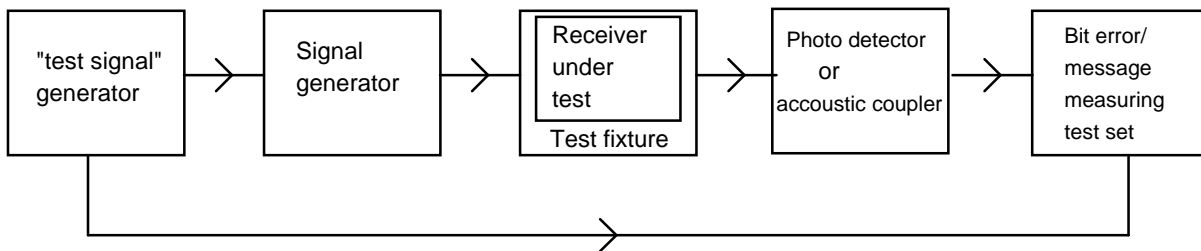
Figure 8: Measurement arrangement for equipment with an integral antenna
