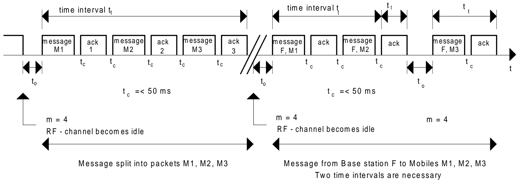
Figure 3: Access protocol sharing data/data
