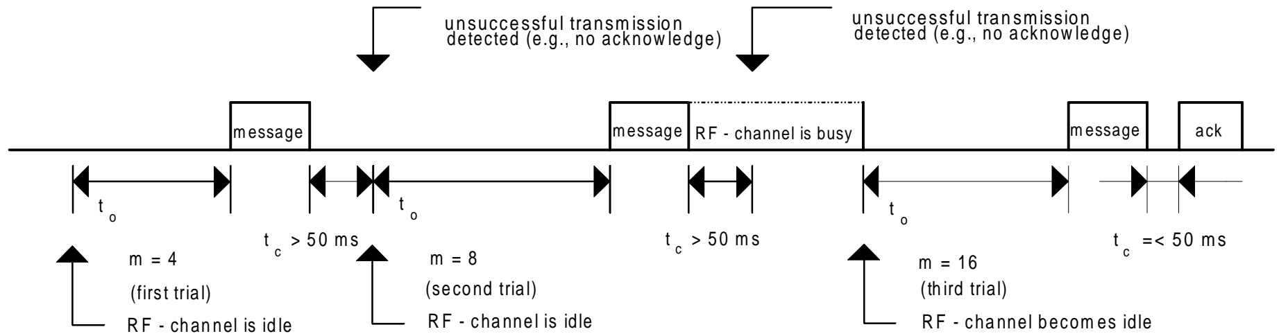
Figure 2: Access protocol: unsuccessful transmission
