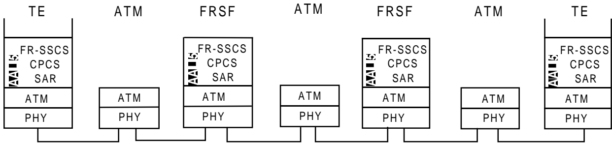
Figure 2b: Protocol stack of FRBS provided by FRSF outside B-ISDN
