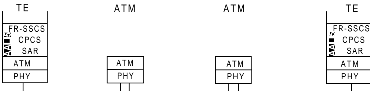
Figure 3b: Protocol stack of frame relay protocol carried by an ATM bearer service
