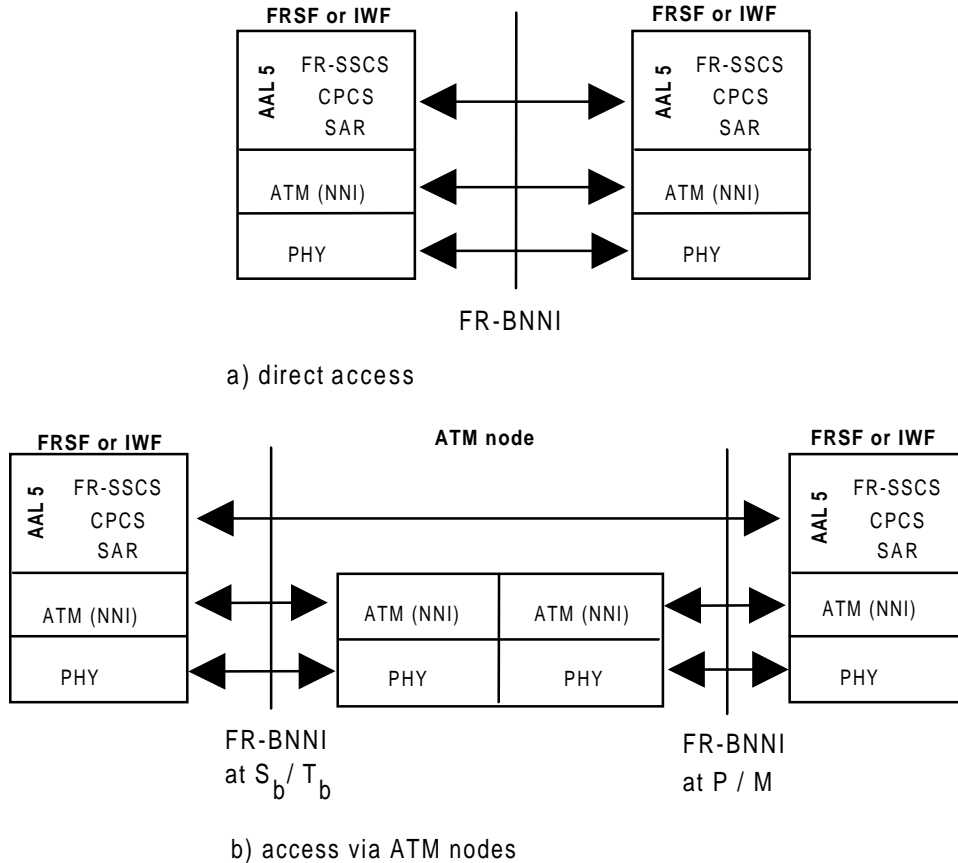
Figure 5: FR-BNNI U-plane protocol reference architecture
