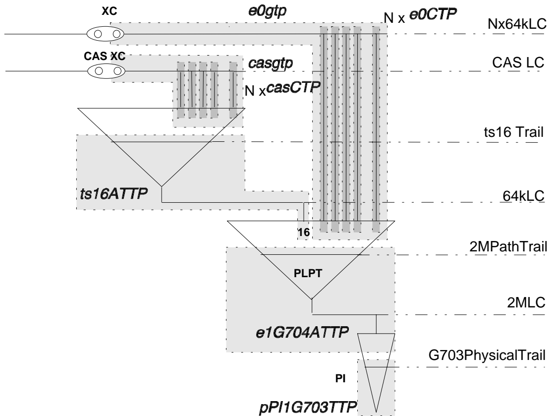
Figure 21: CAS for N x 64 kbit/s link connection on aggregate
