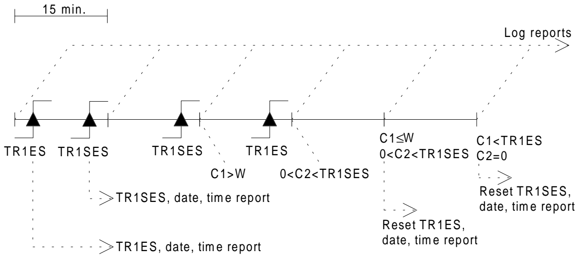
Figure 9: Performance evaluation with hysteresis
