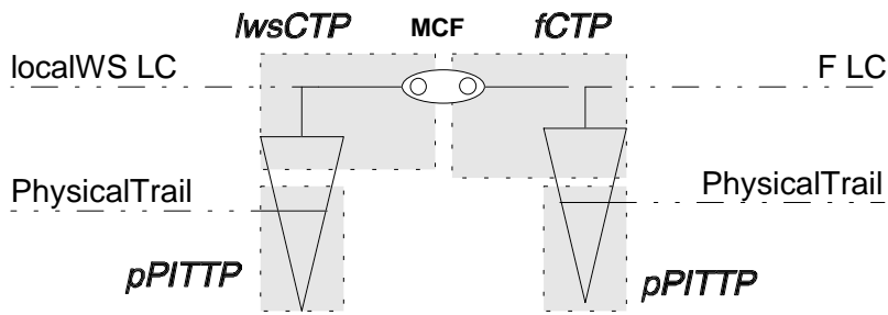
Figure 43: Management relay through F interface
