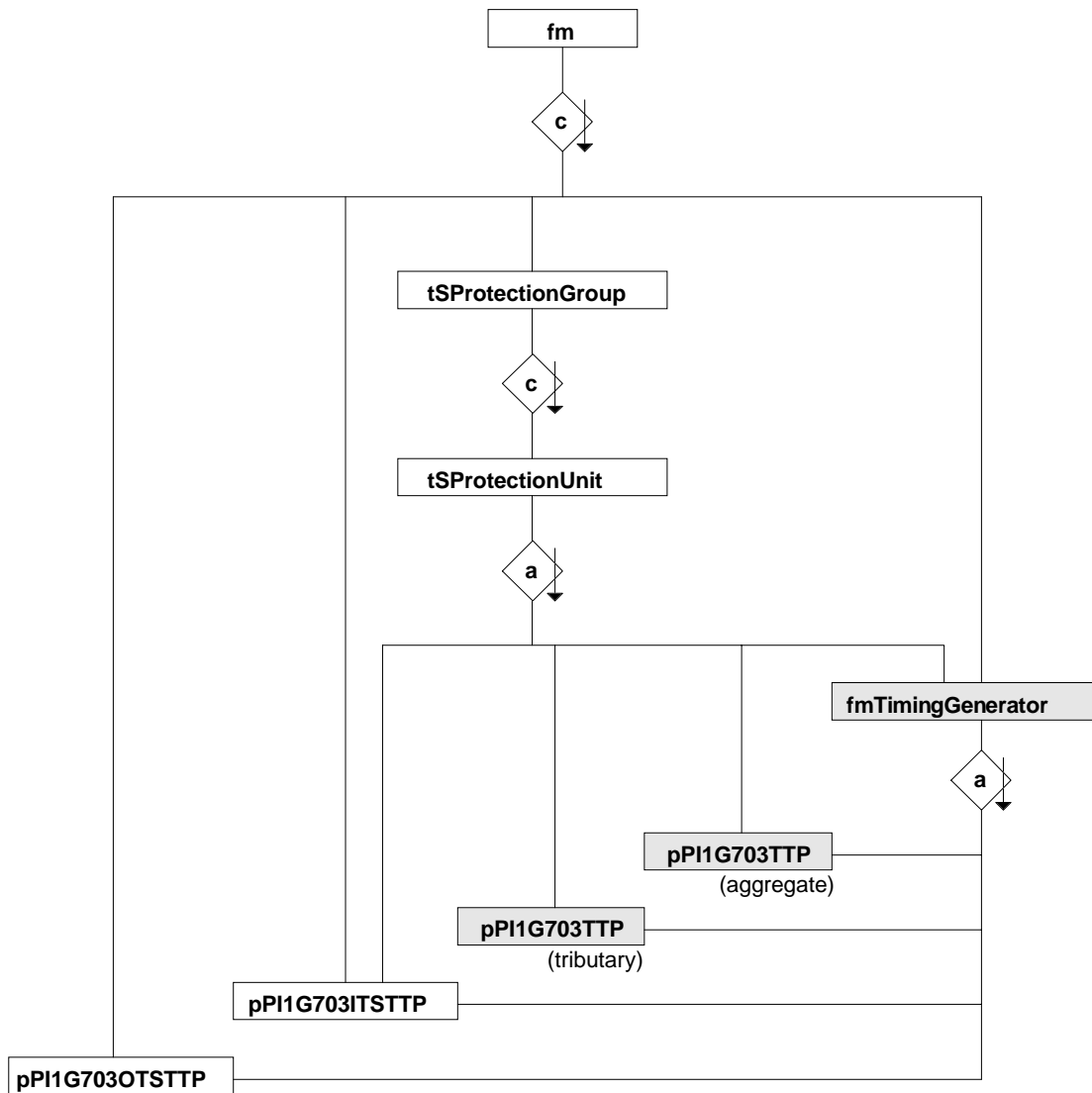
Figure 53: Entity relationship diagram. Synchronization
