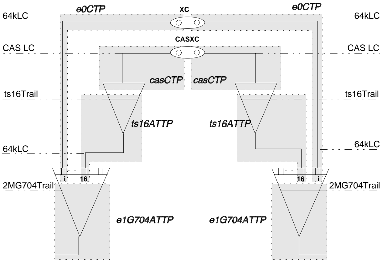
Figure 20: CAS cross-connection between CCITT Recommendation G.704 [2] tributary and aggregate
