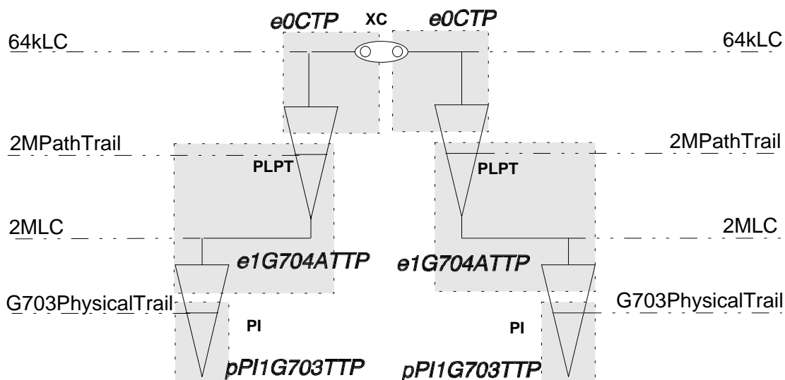
Figure 17: 64 kbit/s cross-connection between ITU-T Recommendation G.704 [2] tributary and aggregate
