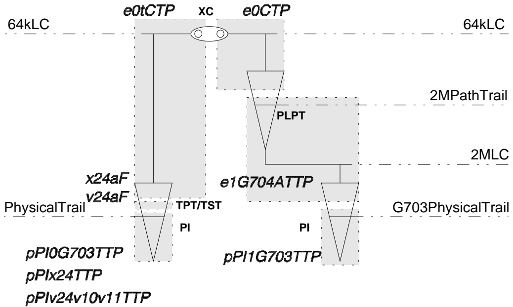
Figure 15: 64 kbit/s cross-connection between tributary and aggregate
