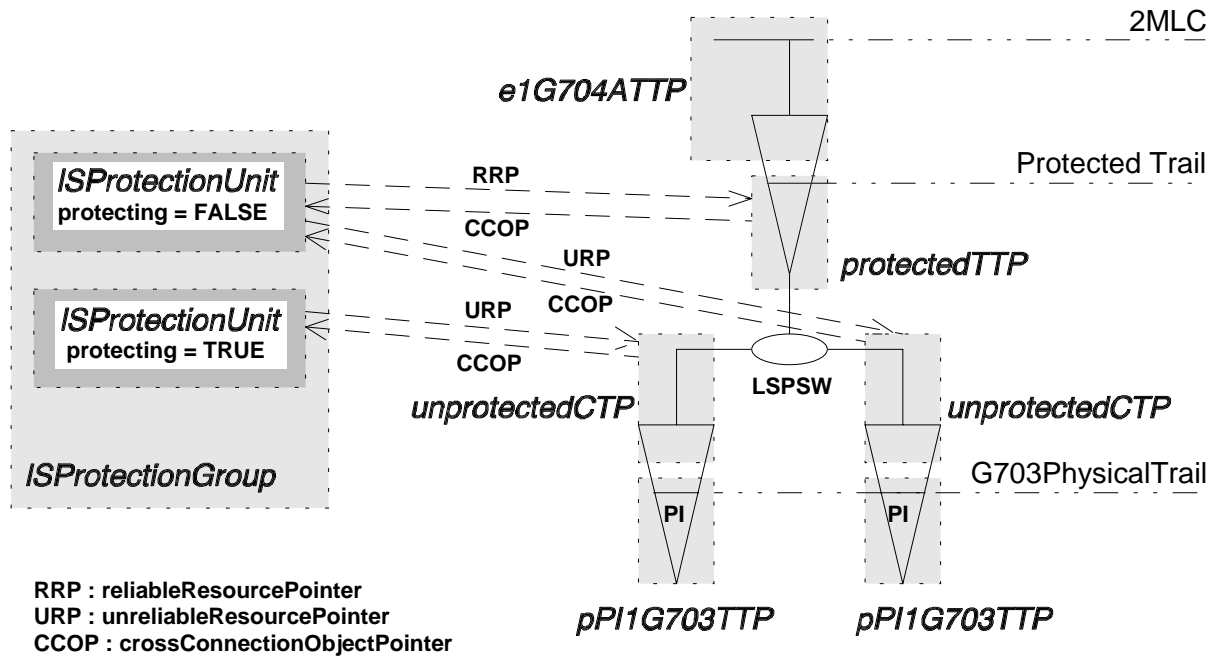
Figure 22: Lower order section protection switch (1+1)
