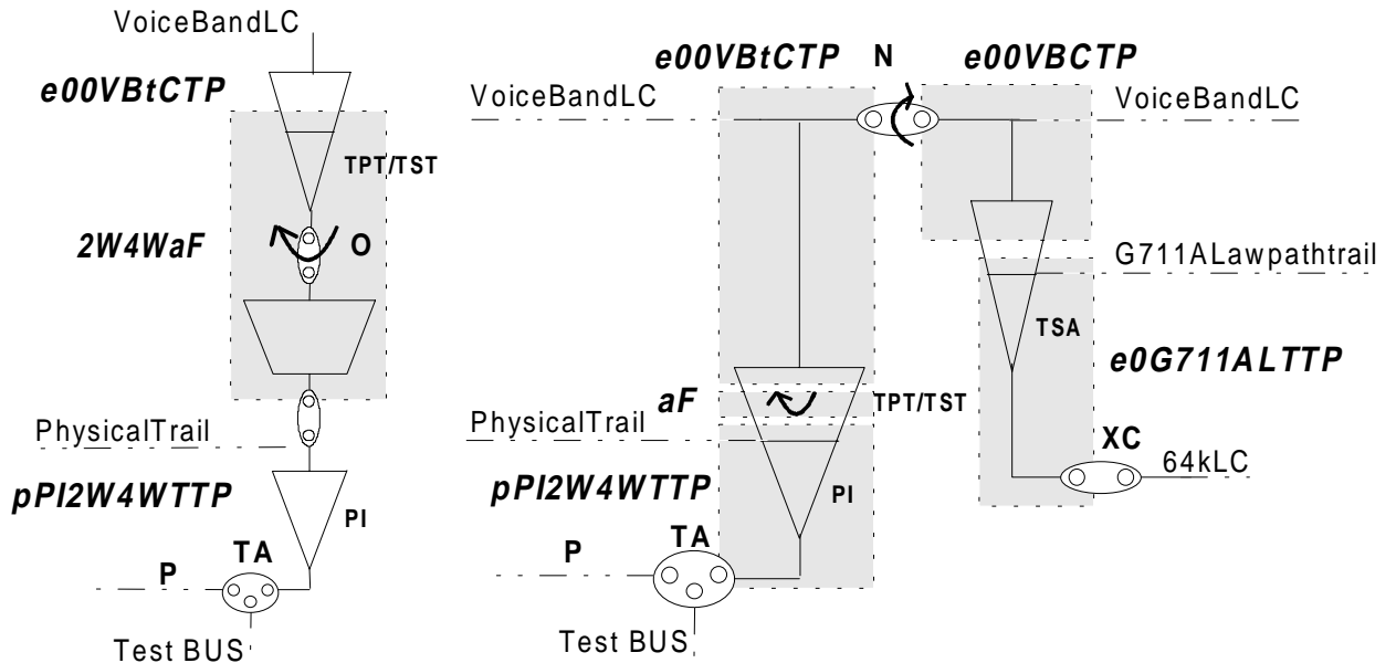
Functional model detailed break-down
