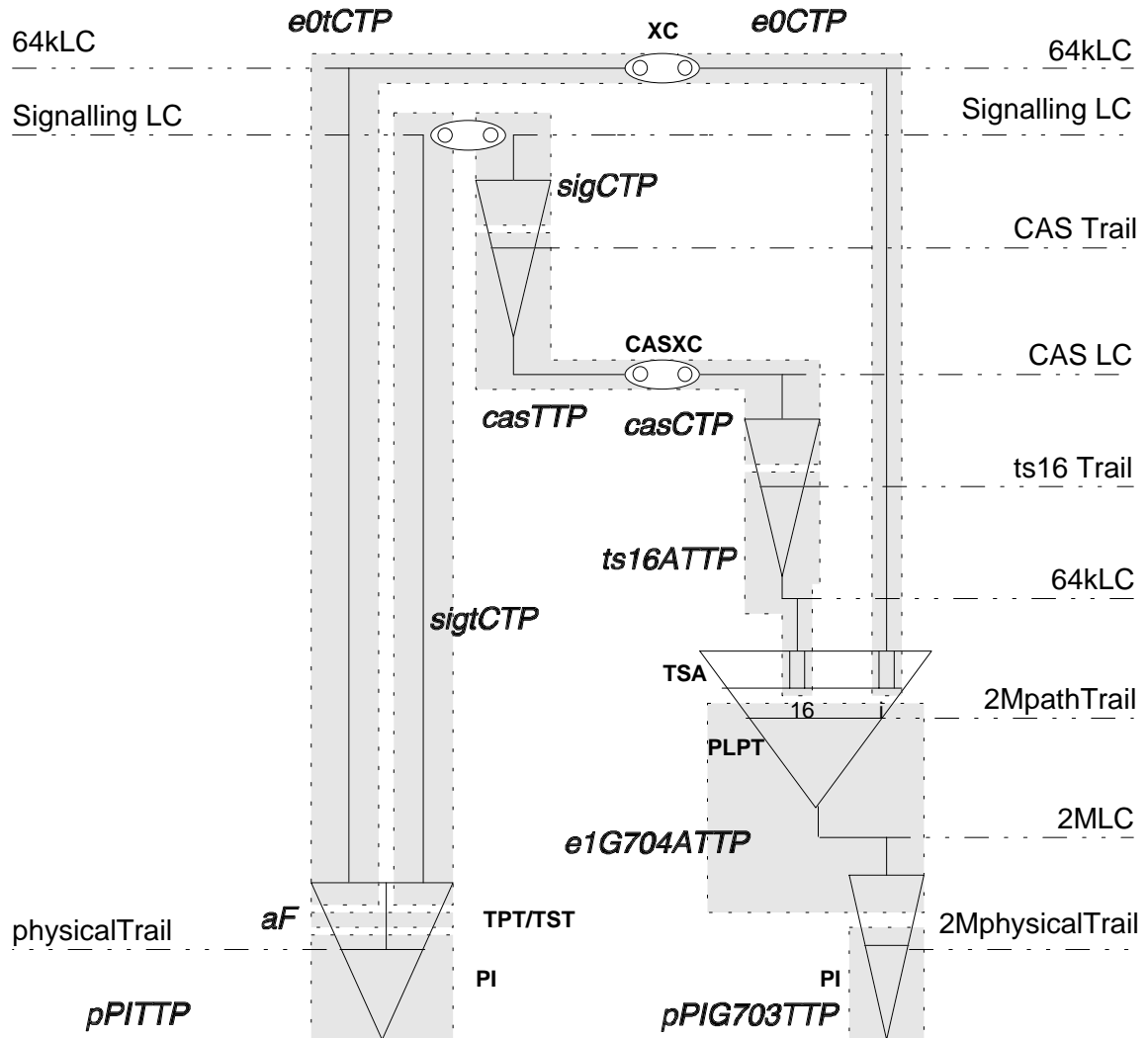
Figure 19: CAS cross-connection between tributary and aggregate
