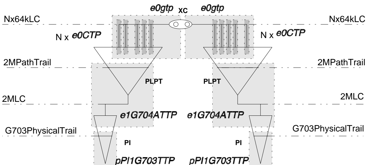
Figure 18: N x 64 kbit/s cross-connection between ITU-T Recommendation G.704 [2] tributary and aggregate
