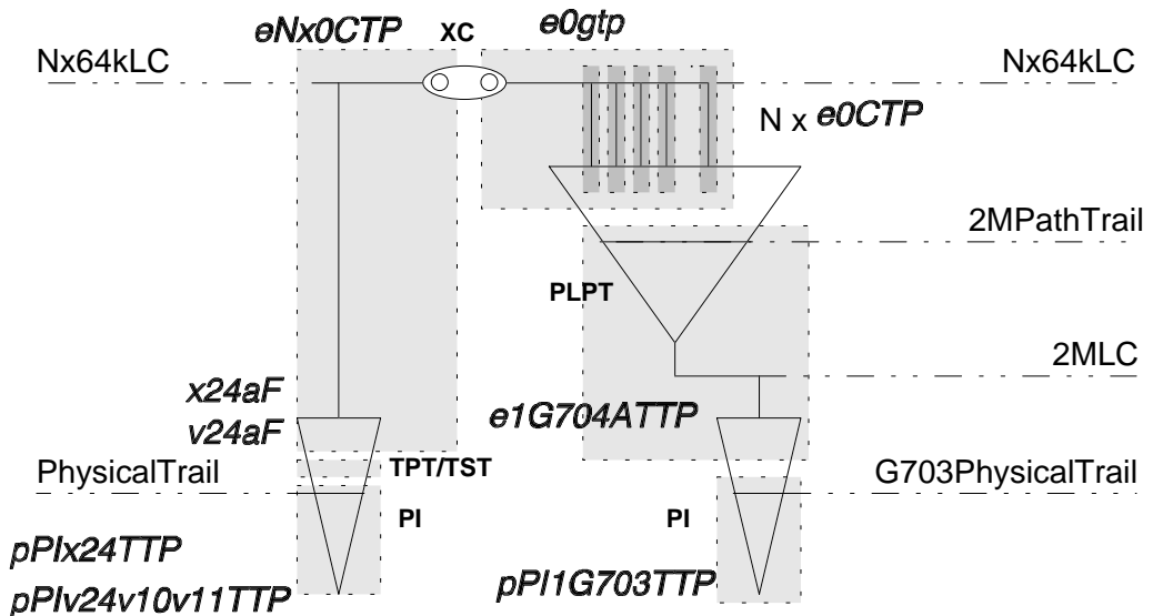
Figure 16: N x 64 kbit/s cross-connection between tributary and aggregate
