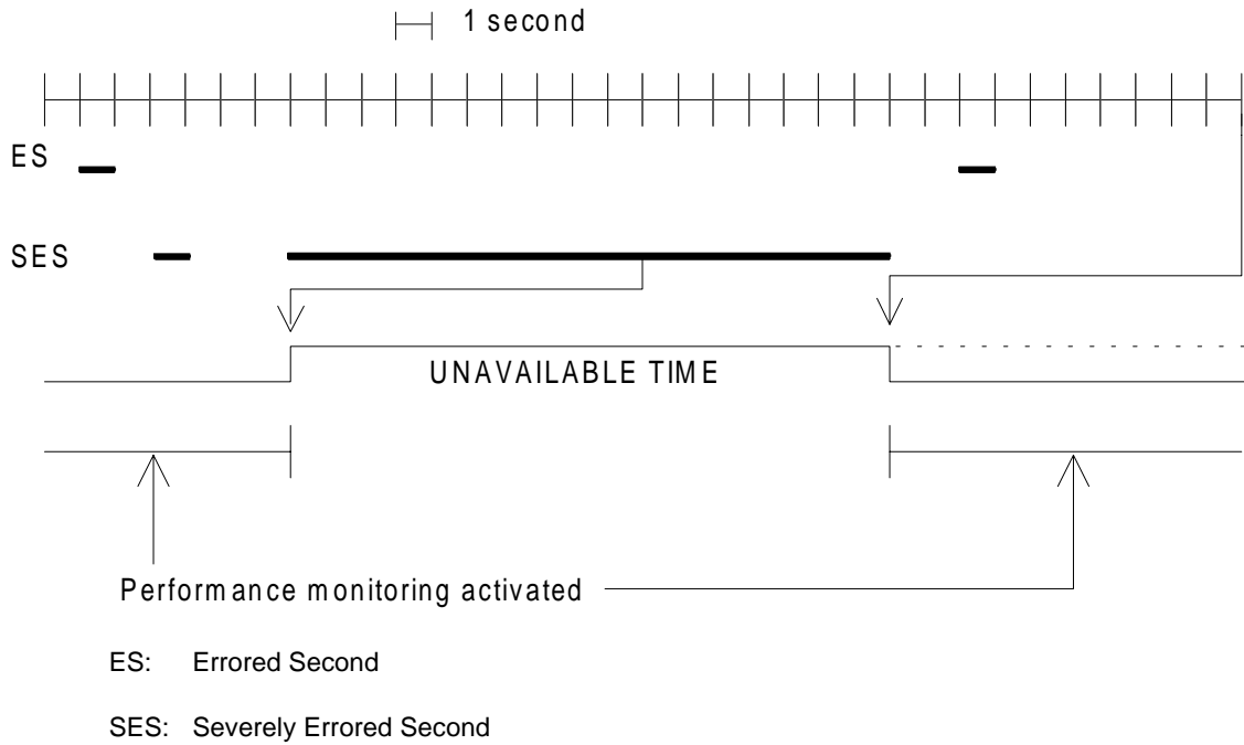
Figure 5: Definition of unavailable time
