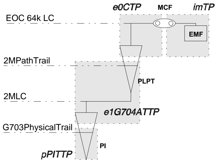
Figure 40: Management through 64 kbit/s EOC
