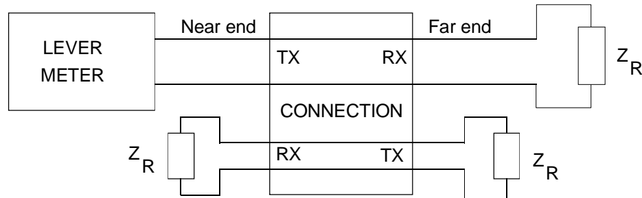
Figure A.10: Single tone interference
