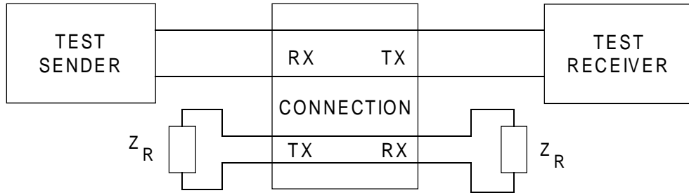
Figure A.4: Group delay distortion
