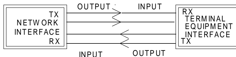
Figure 4: Leased line configuration conventions
