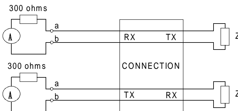
Figure A.15: Power feeding
