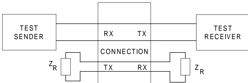
Figure A.7: Impulsive noise
