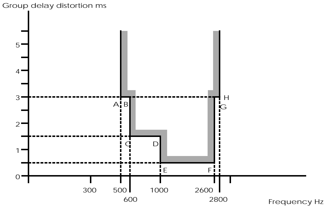
Figure 3: Limits for group delay relative to the minimum measured group delay in the 500 Hz to 2 800 Hz band
