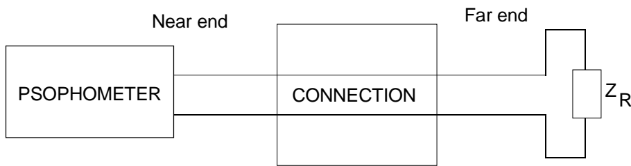
Figure A.7: Random circuit noise
