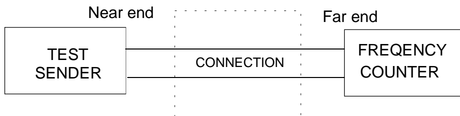
Figure A.12: Frequency error
