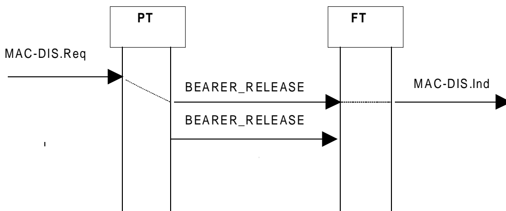
Figure 89: Bearer release
