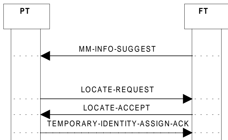
Figure 56: Location update
