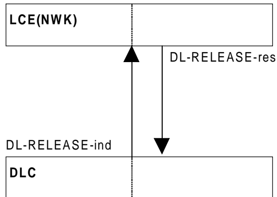
Figure 76: Link release "normal", receiving side
