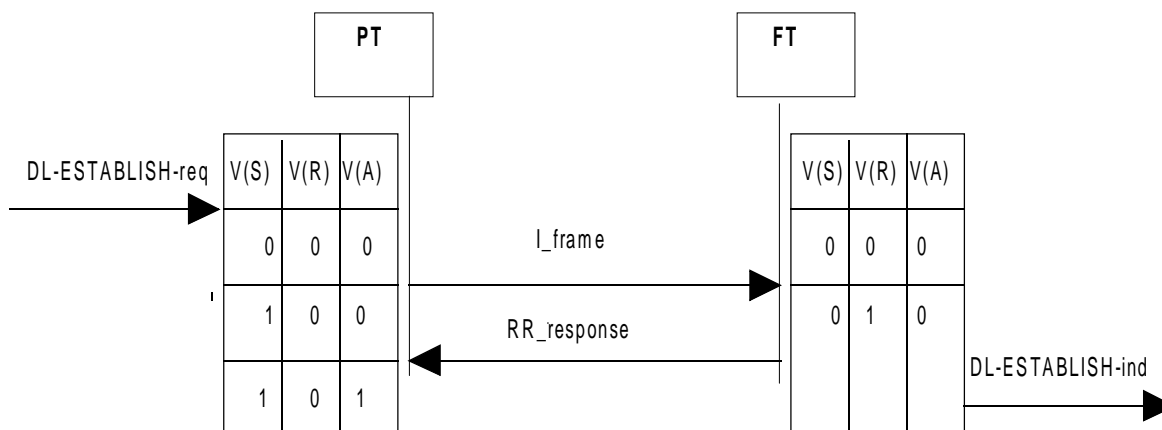
Figure 78: Class A link establishment
