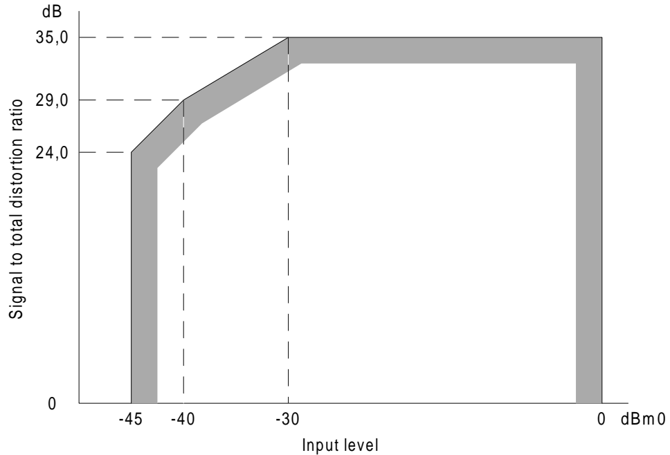
Figure 8: Limits for signal-to-total distortion ratio as a function of input level. Input or output connection. Signalling on separate wires without feeding bridge
