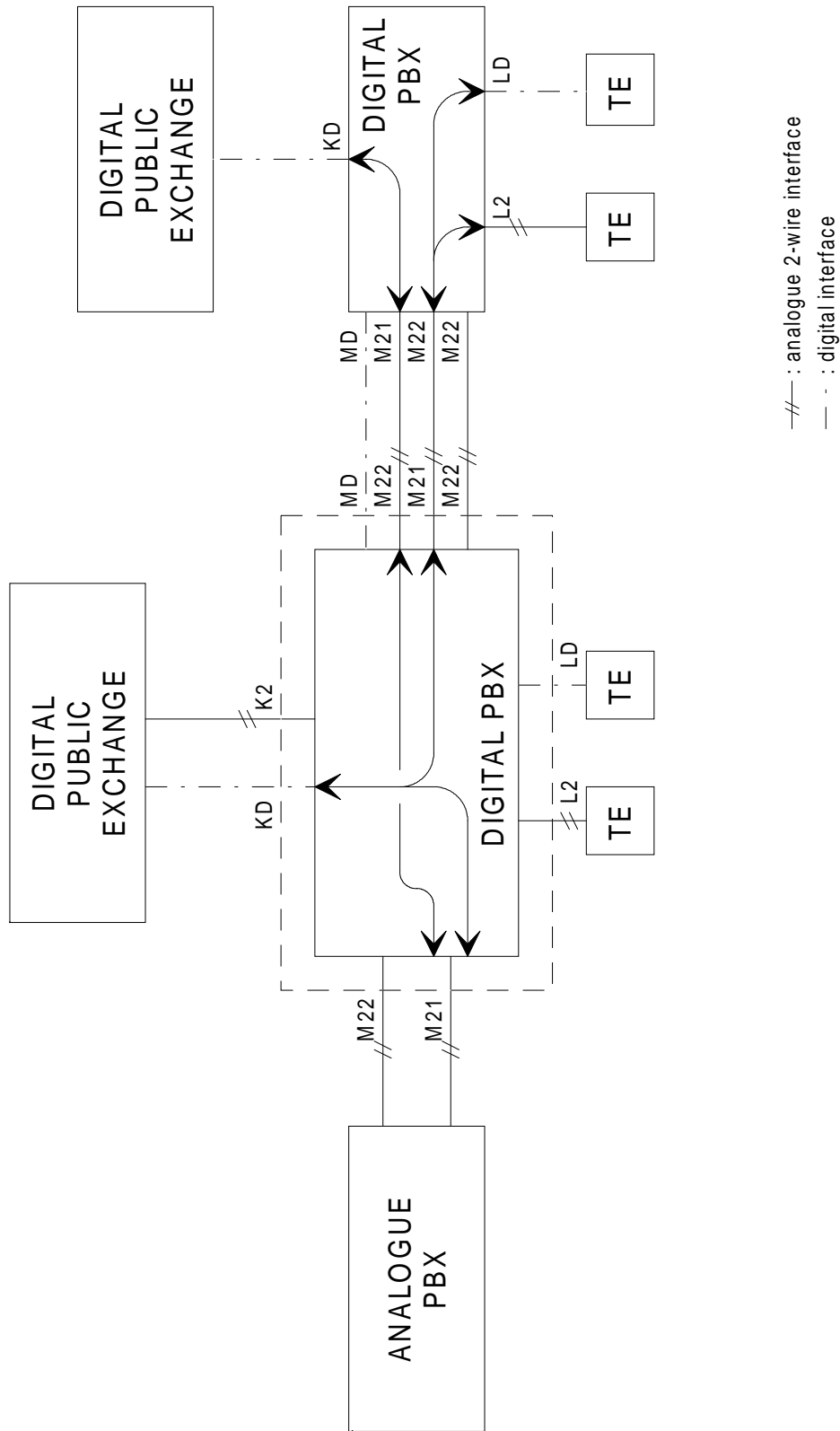
Figure 2: Detailed illustration for access to Public Switched Telephone Network (PSTN) involving M2 interfaces
