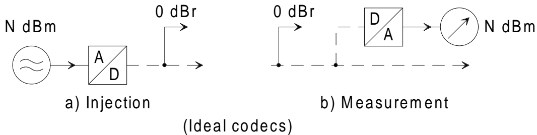
Figure D.3: Interpretation of absolute signal level in a digital path with relative level 0 dBr
