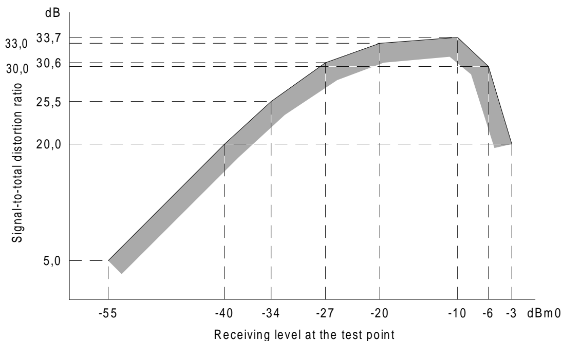
Figure 17: Limits of signal-to-distortion ratio, receiving, method 1
