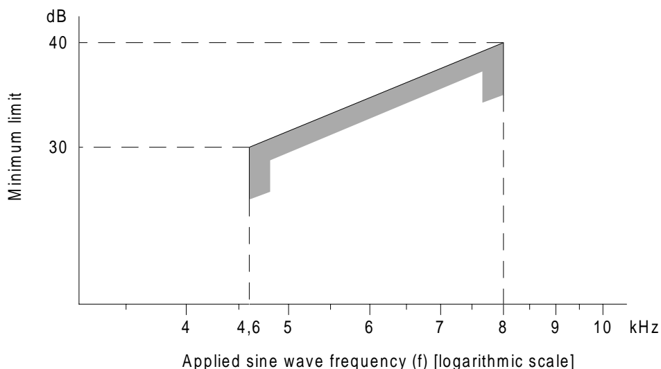
Figure 21: Discrimination levels (sending)
