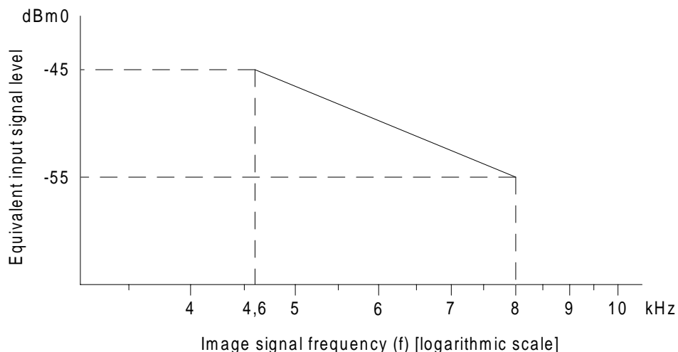
Figure 22: Discrimination levels (receiving)
