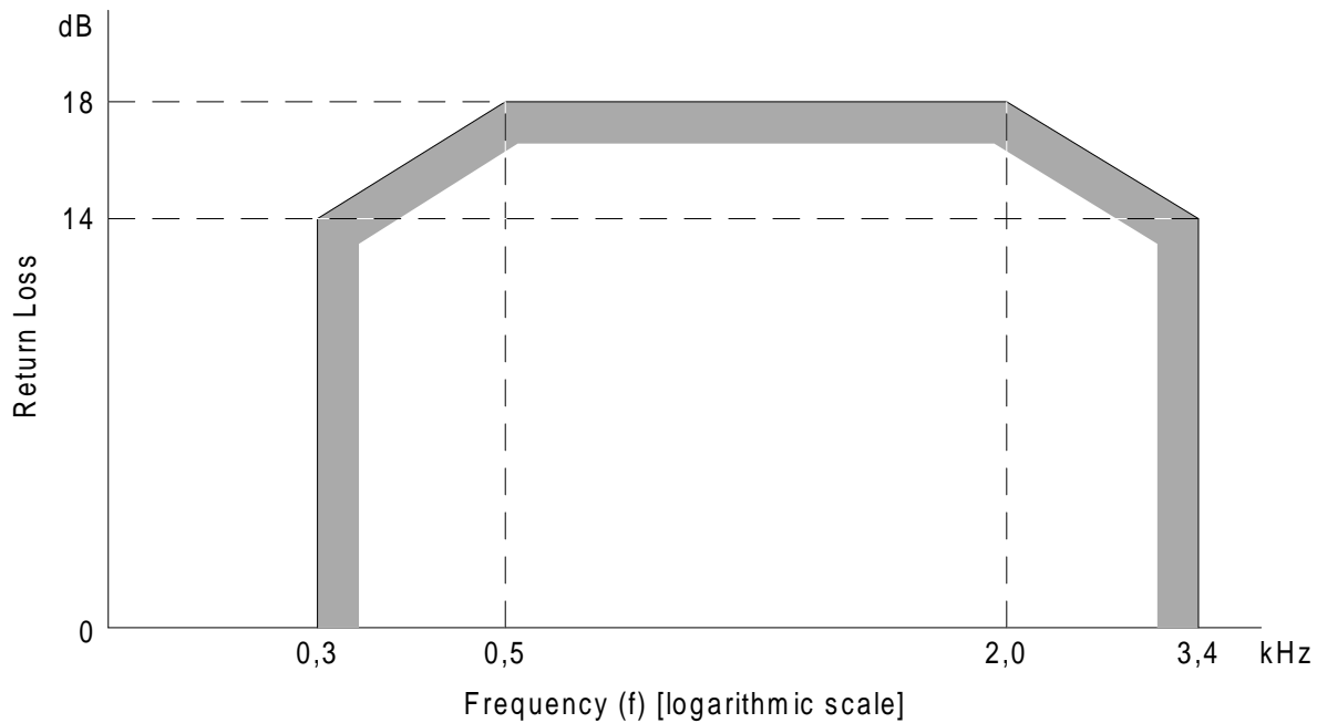
Figure 4: Minimum value of return loss against the nominal PBX impedance
