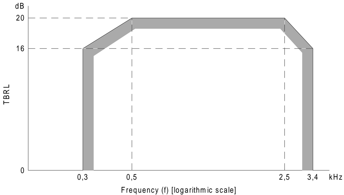
Figure 12: Limits for TBRL
