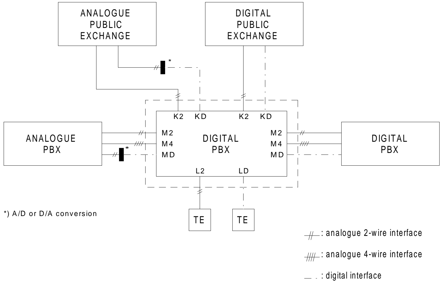
Figure 1: Interfaces of digital PBX's in network interconnections
