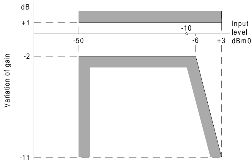
Figure 20: Variation of gain with input level (receiving)
