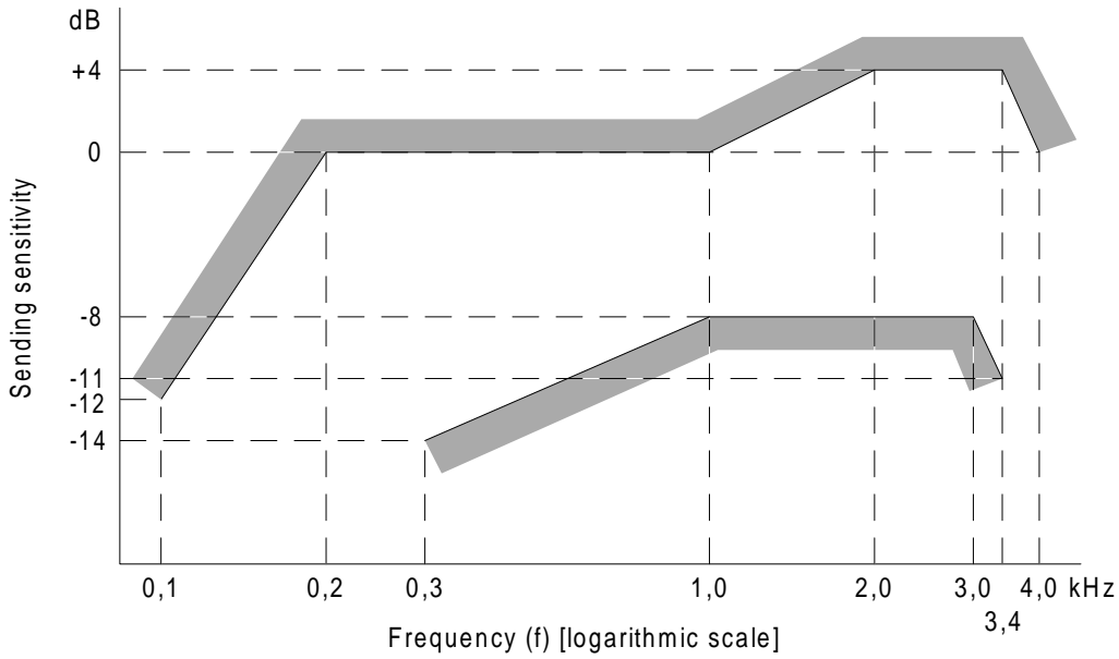
Figure 13: Sending sensitivity/frequency mask
