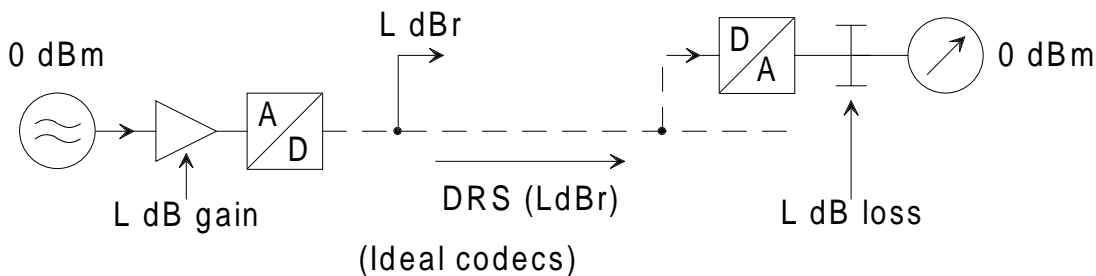
Figure D.4: Interpretation of a 0 dBm0 reference sequence DRS( L dBr) for a digital path with relative level L dBr
