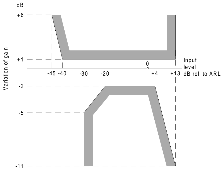
Figure 19: Variation of gain with input level (sending)
