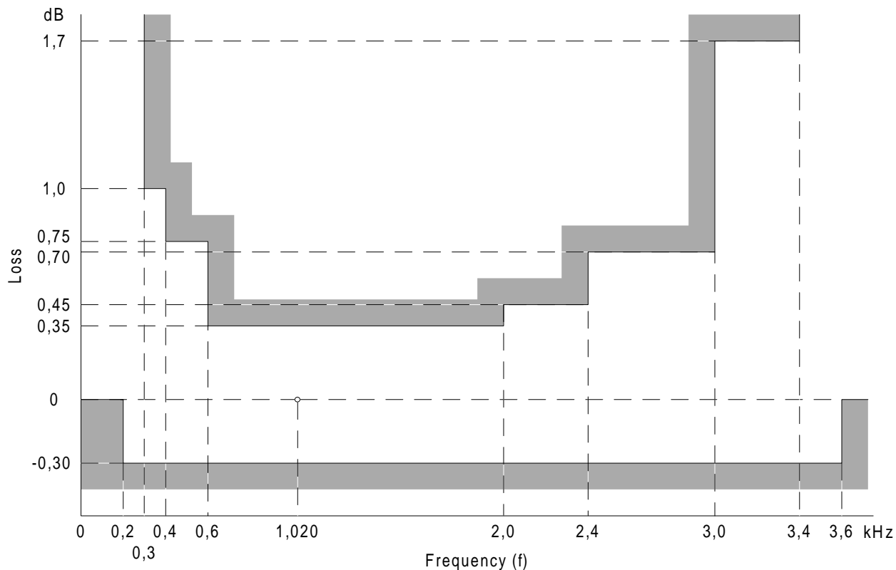
Figure 6: Loss distortion with frequency - input connection
