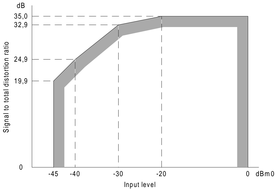
Figure 10: Limits for signal-to-total distortion ratio as a function of input level including analogue noise. Input connection (L i = 0 dBr). Interfaces L2 and M2 with feeding bridges
