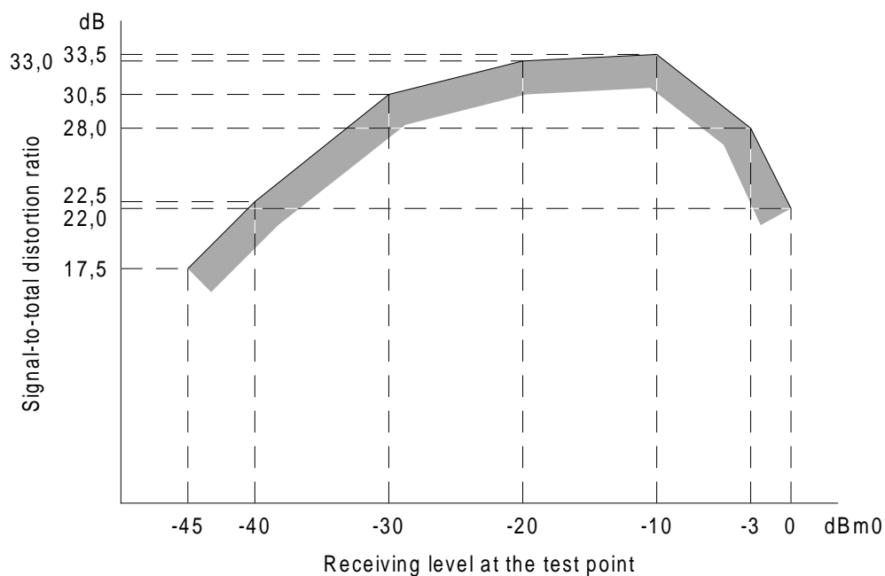
Figure 18: Limits for signal-to-distortion ratio, receiving, method 2
