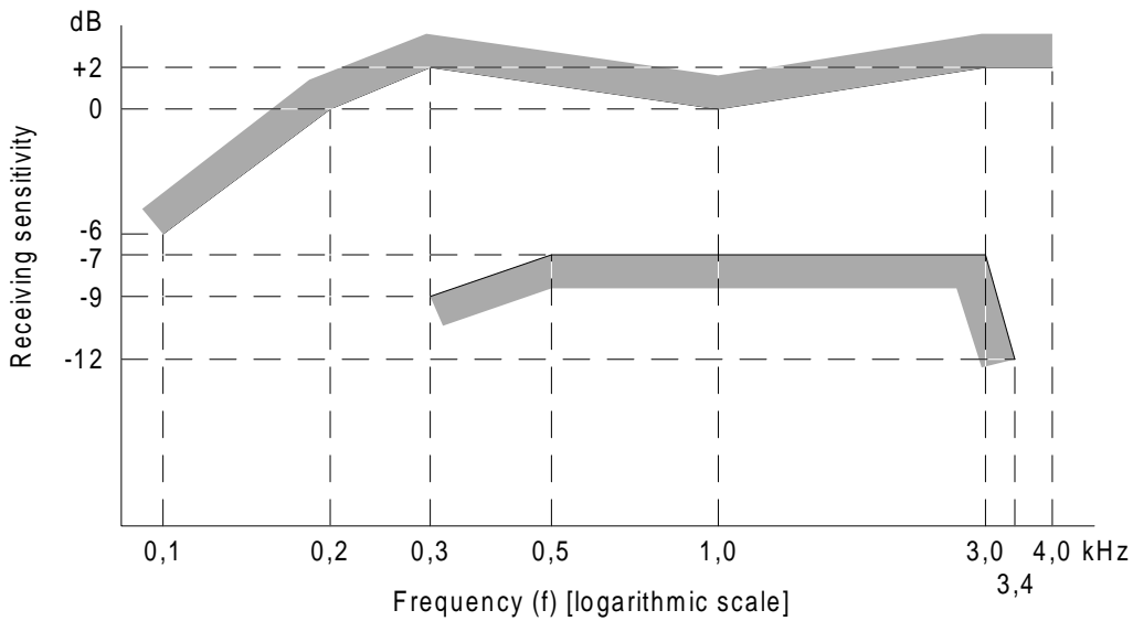
Figure 14: Receiving sensitivity/frequency mask
