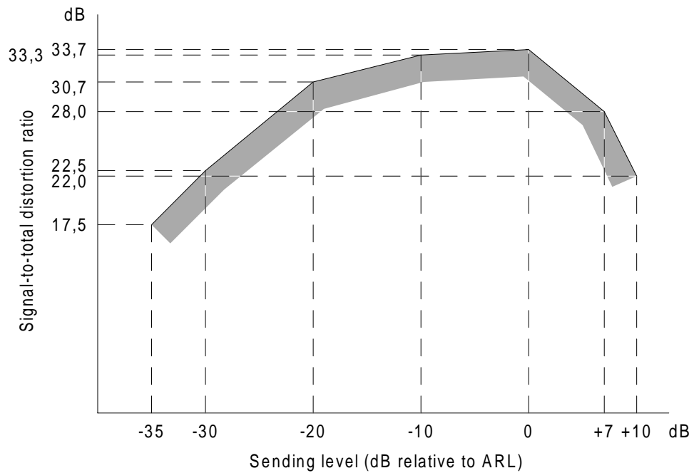
Figure 16: Limits for signal-to-distortion ratio, sending, method 2
