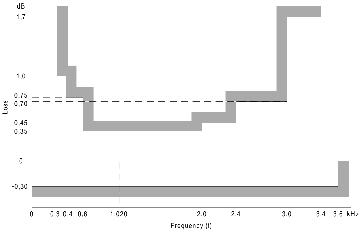
Figure 7: Loss distortion with frequency - output connection
