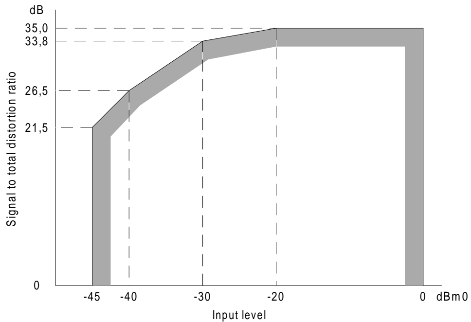
Figure 9: Limits for signal to-total distortion ratio as a function of input level. Input or output connection. Signalling on the speech wires without feeding bridge
