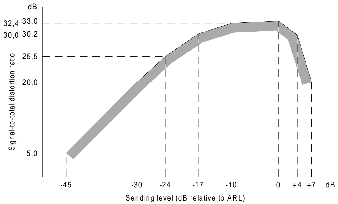
Figure 15: Limits of signal-to-distortion ratio, sending, method 1
