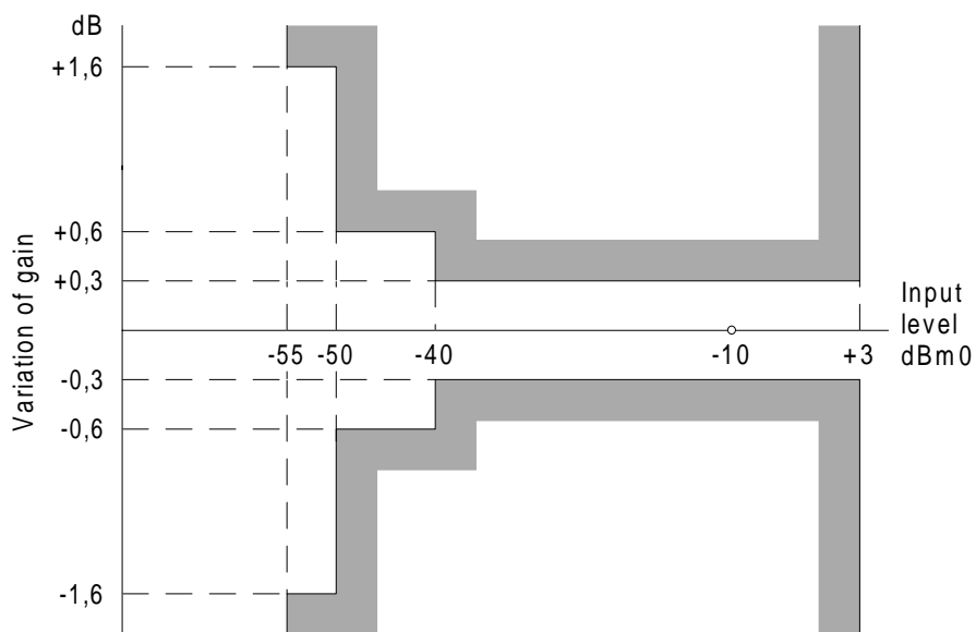
Figure 5: Variation of gain with input level
