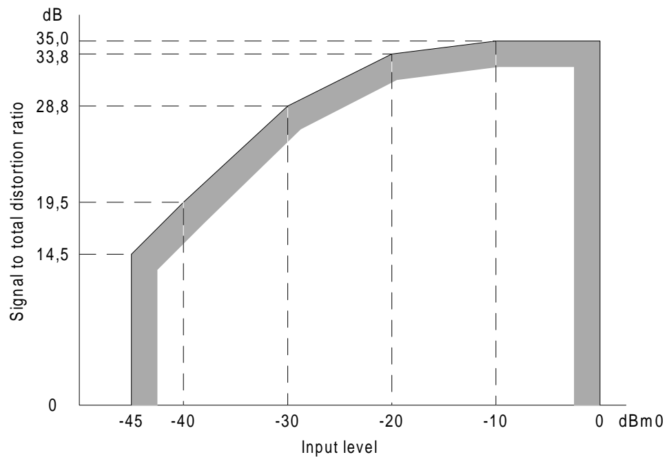
Figure 11: Limits for signal-to-total distortion ratio as a function of input level including analogue noise. Output connection ( L_o = -7 dBr). Interfaces L2 and M2 with feeding bridges
