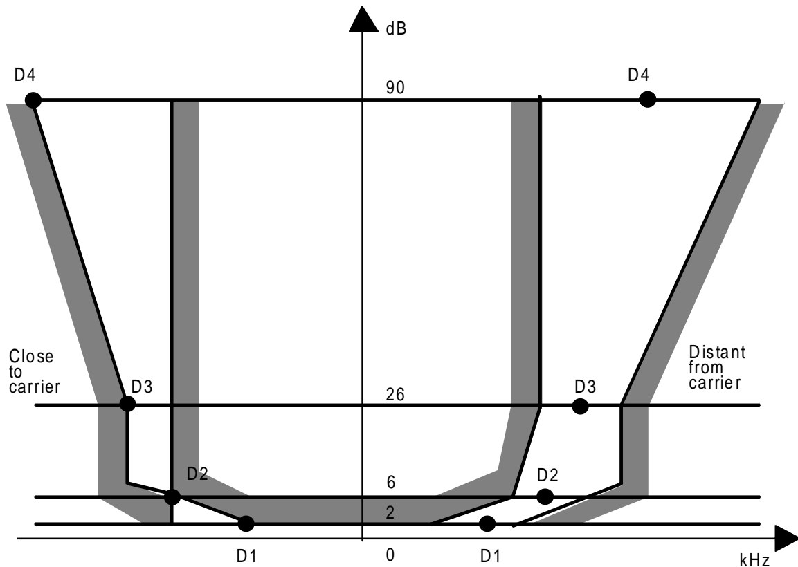
Figure B.1: IF filter characteristic
