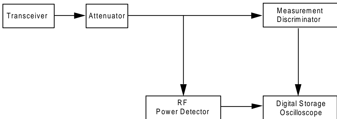
Figure 1: Measurement arrangement
