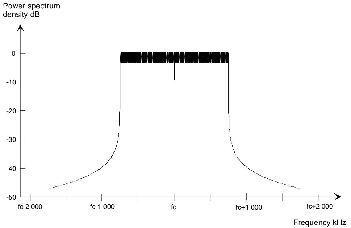
Figure 102: Theoretical DAB transmission signal spectrum for transmission mode I
