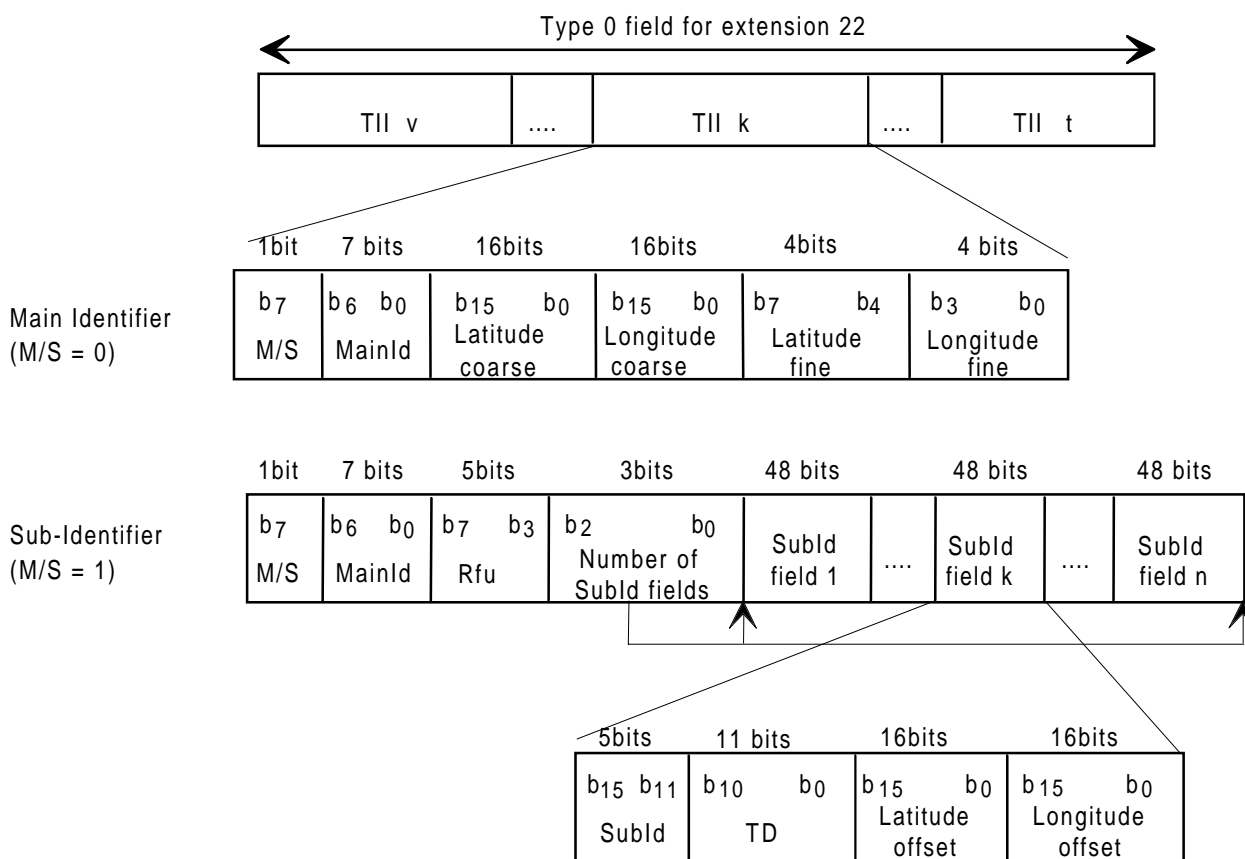
Figure 45: Structure of the Transmitter Identification Information (TII) field
