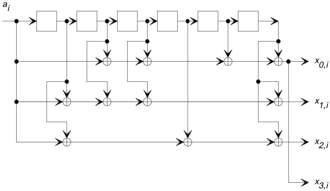
Figure 86: Convolutional encoder
