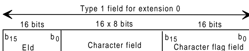
Figure 52: Structure of the ensemble label field
