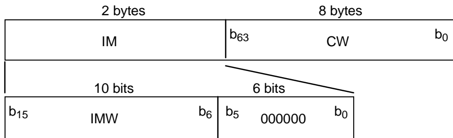
Figure 71: Structure of the IW for Packet mode in configurations 2 and 3
