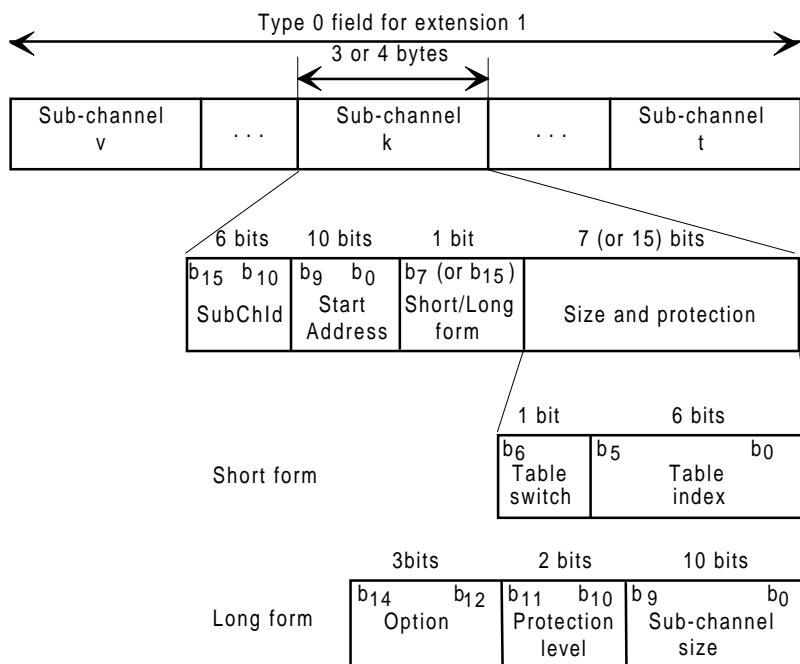
Figure 13: Structure of the sub-channel organization field
