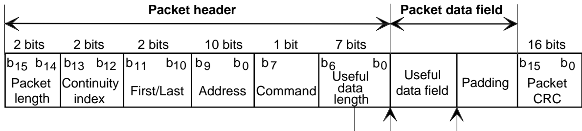
Figure 8: Packet structure
