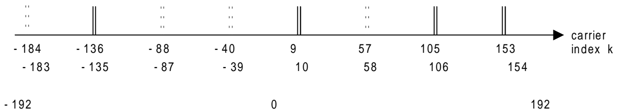
Figure 101: Example of TII signal in transmission mode II
