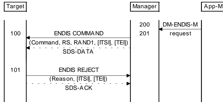
Figure 34: Rejecting a command
