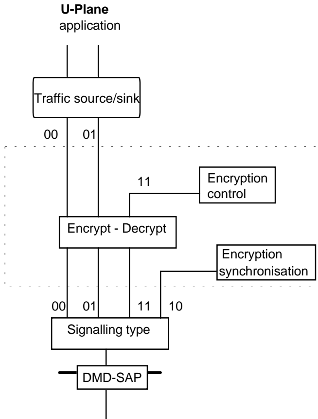
Figure 40: Functional model of the encryption unit
