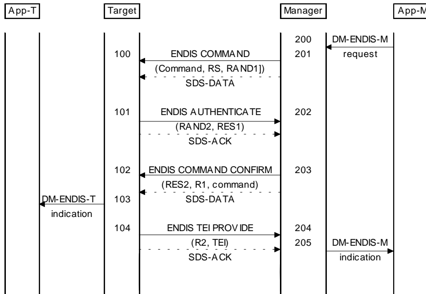
Figure 33: Delivery of TEI
