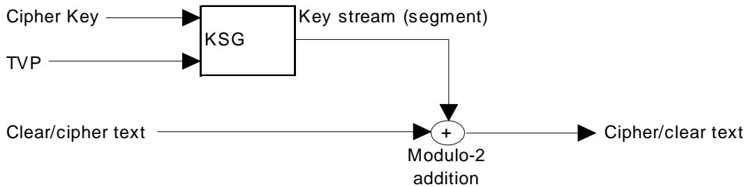
Figure 9: Speech and control information encryption
