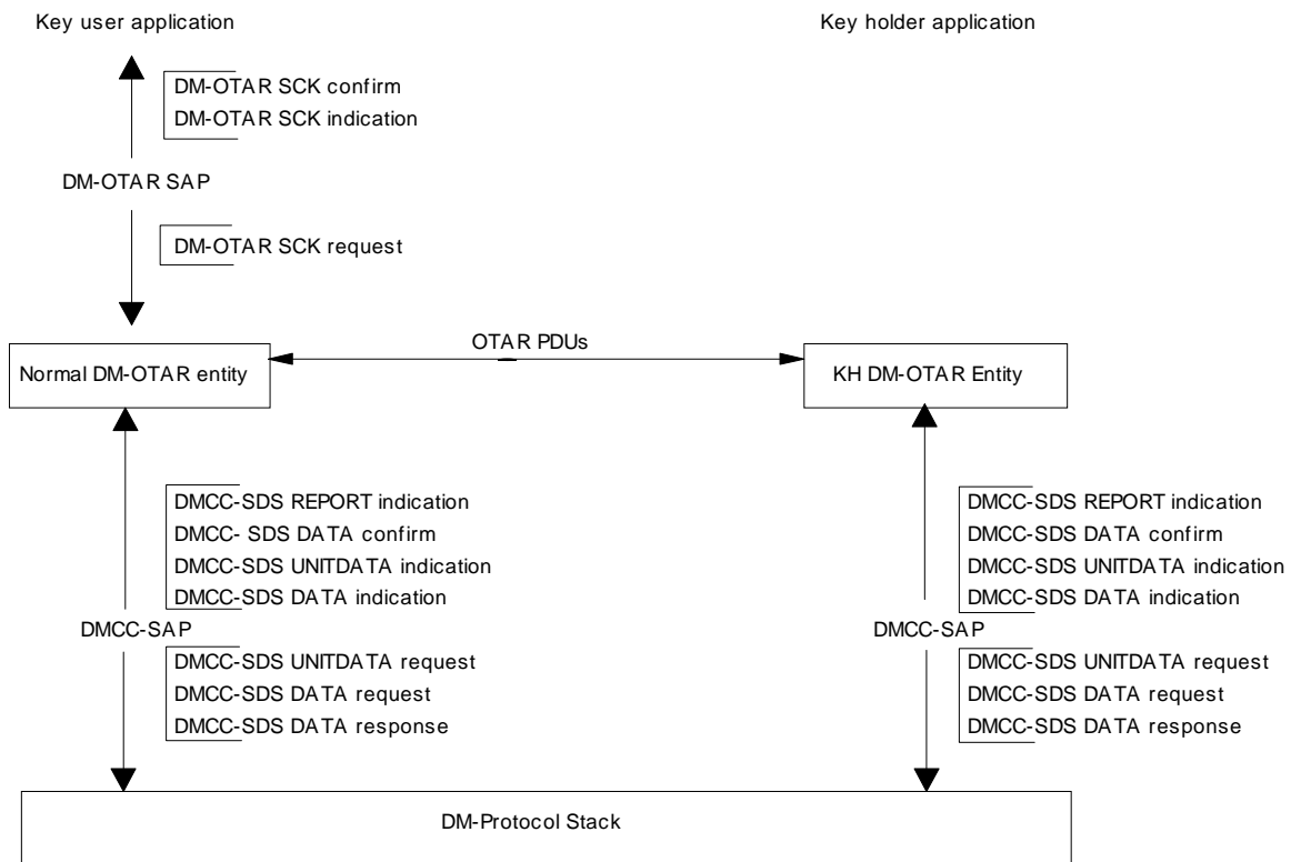
Figure 19: Model for MS to KH protocol
