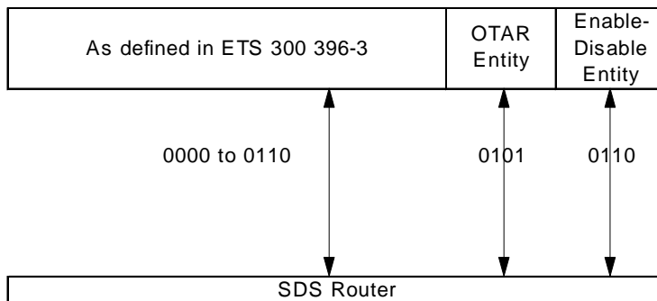
Figure 29: Routing of SDS messages to terminating entities
