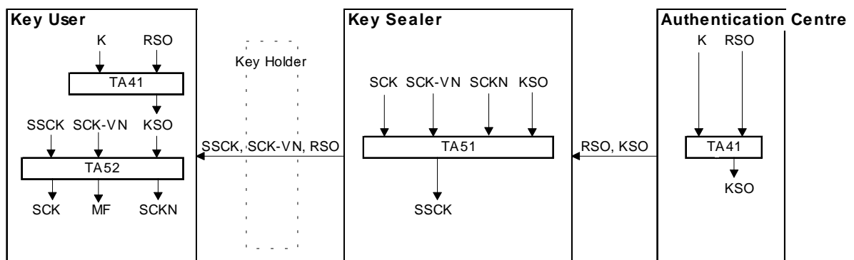
Figure 16: Distribution of SCK by a key sealer
