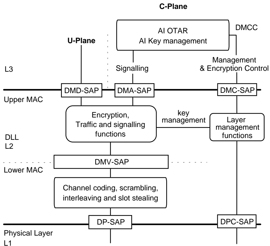
Figure 14: Relationship of security functions to layer functions
