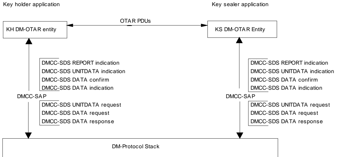
Figure 20: Model for KH to KSL protocol
