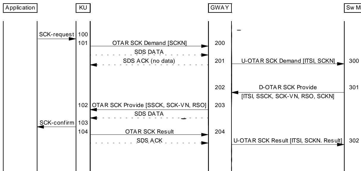
Figure A.1: SCK delivery initiated by MS
