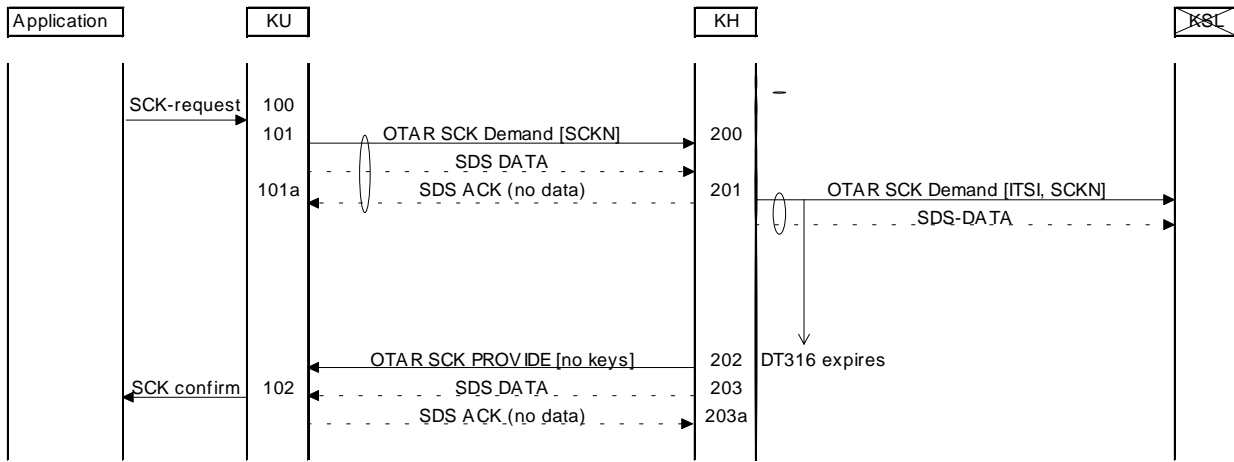
Figure 24: Error scenarios in SCK transfer
