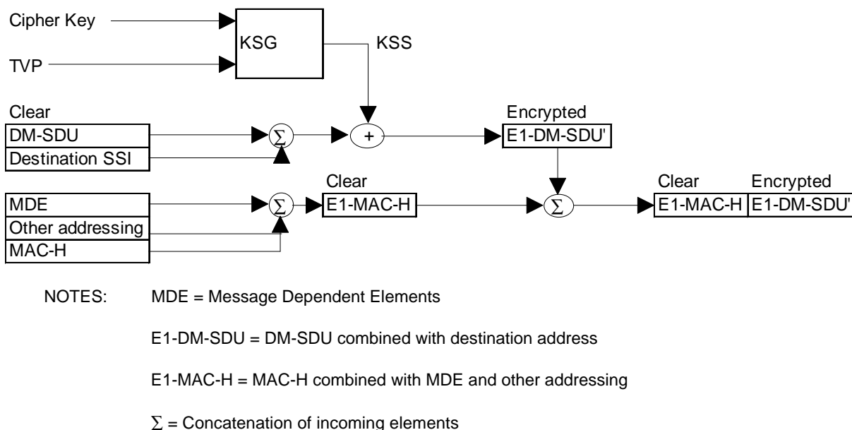
Figure 13: Encryption process as it occurs in TETRA DMO mode 11 2
