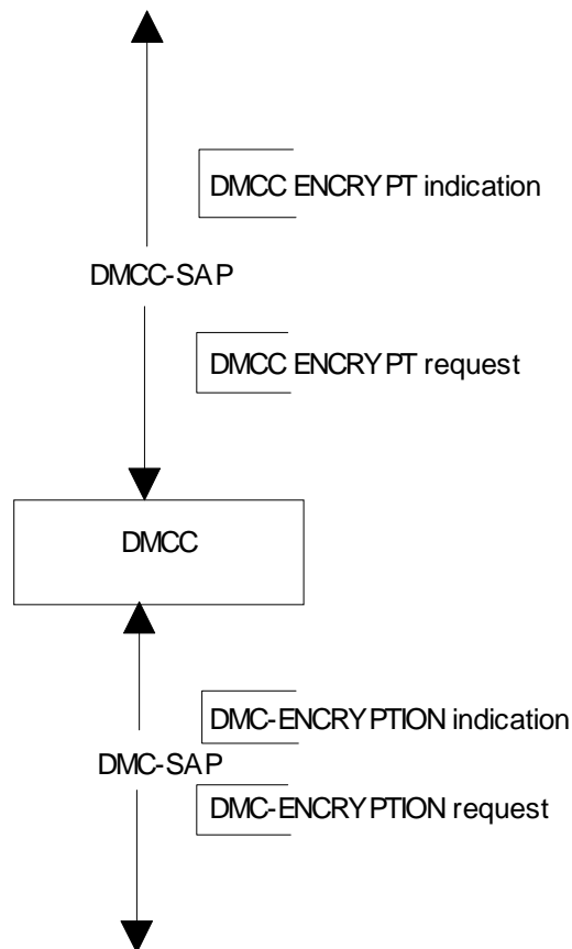
Figure 15: Encryption related services in DMO
