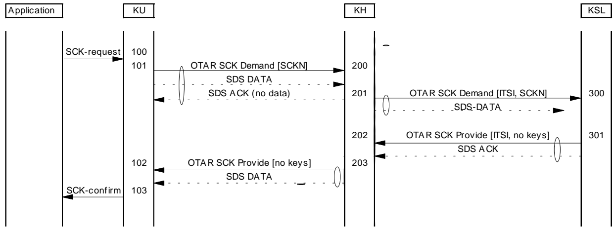
Figure 25: Error scenarios in SCK transfer
