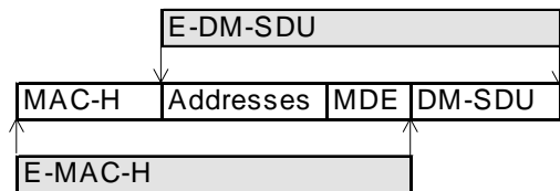
Figure 10: Concatenated structure of TETRA DMO elements
