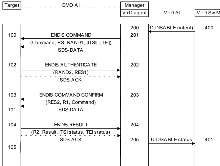
Figure A.2: DM-GWAY acting as V+D agent in secure enable/disable exchange
