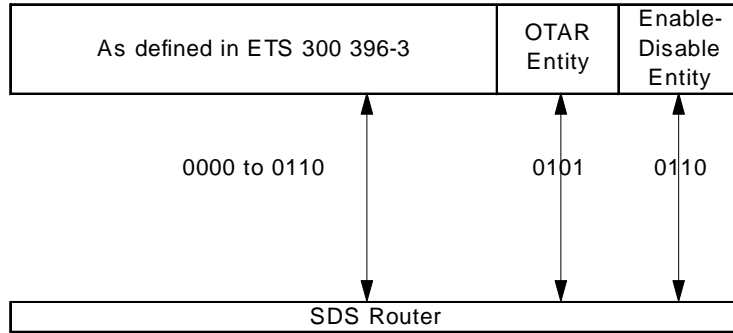
Figure 18: Routing of SDS messages to terminating entities
