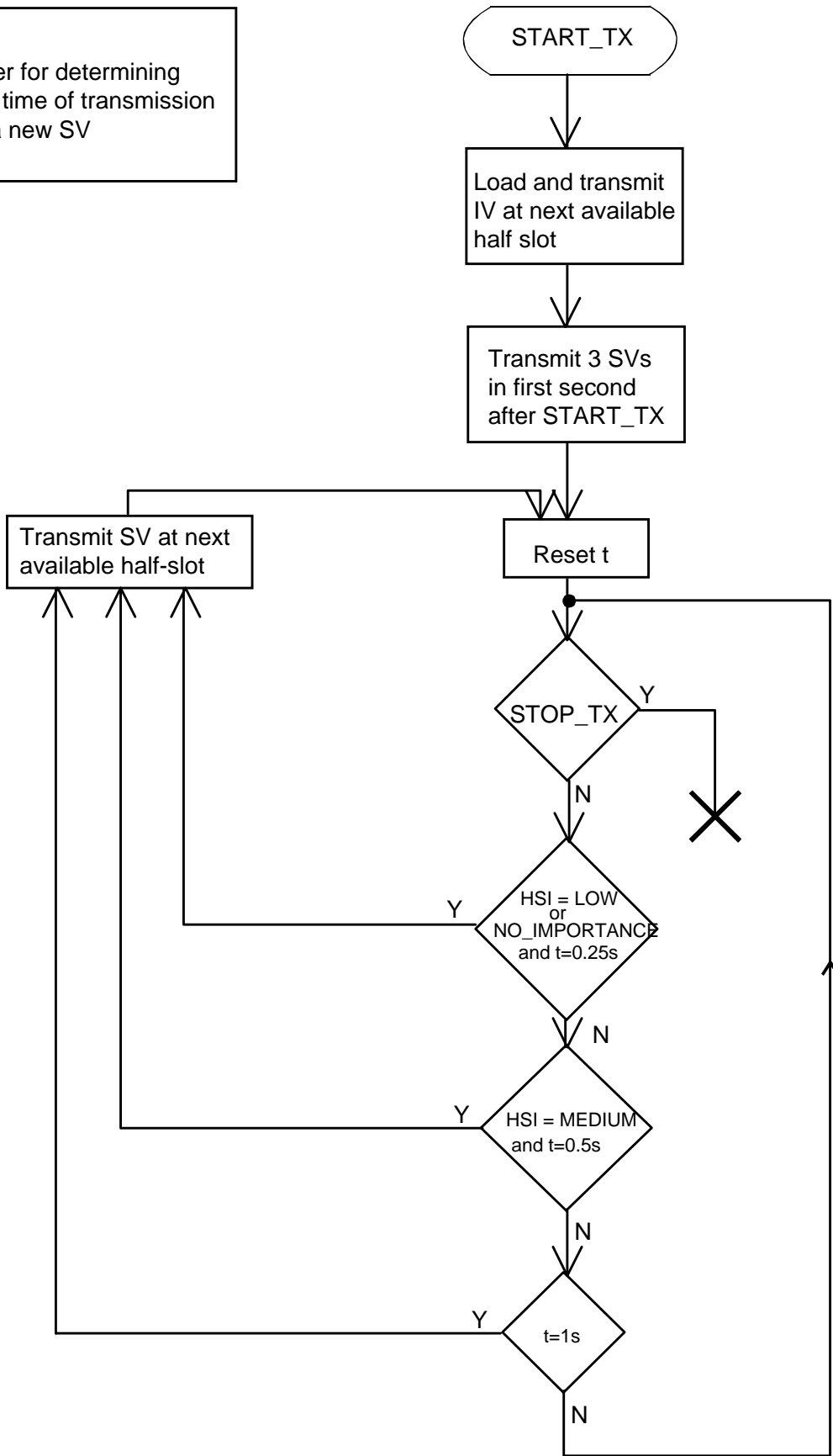
Figure 37: Flow chart of an example transmitter "sync-control" process
