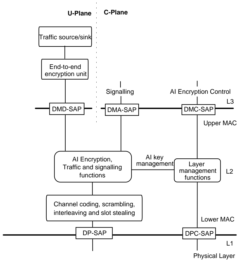
Figure 39: Position of end-to-end encryption unit in MS
