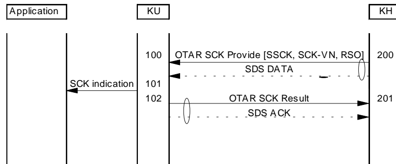
Figure 23: KH distributing SCK unsolicited
