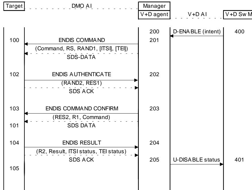
Figure A.3: DM-GWAY acting as V+D agent in secure enable/disable exchange
