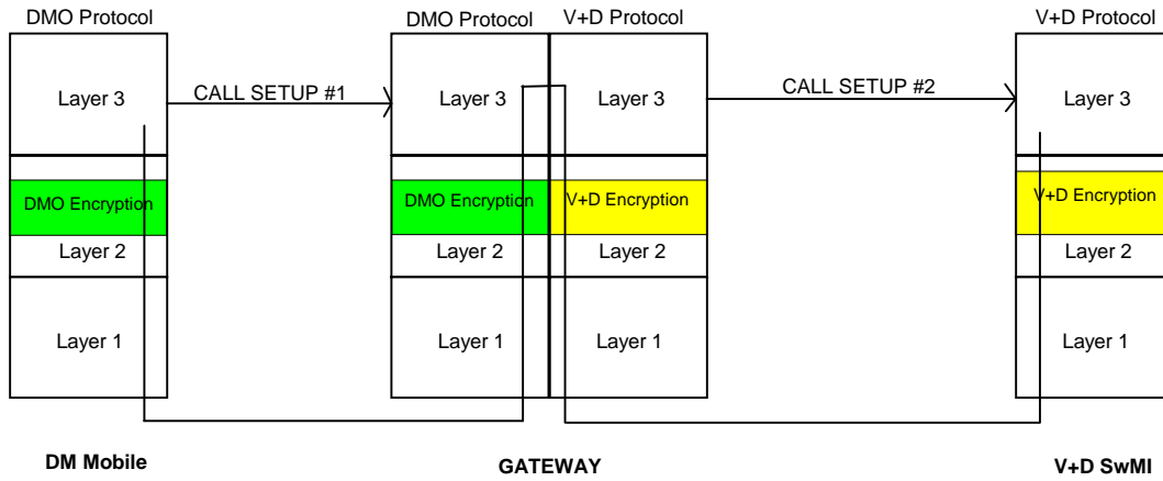
Figure 6: TETRA DMO to TETRA V+D Gateway
