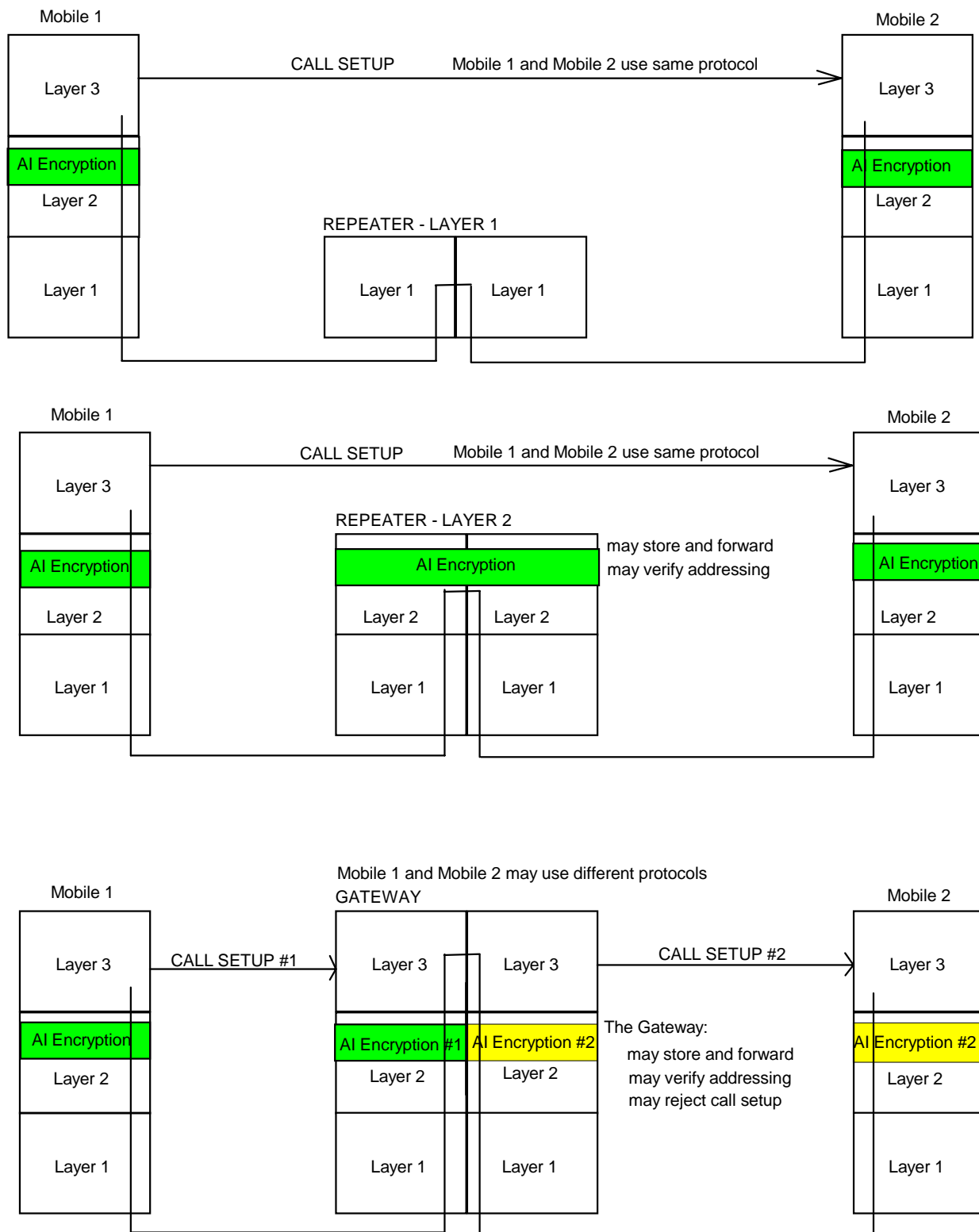
Figure 1: Protocol stacks for multi-hop calls
