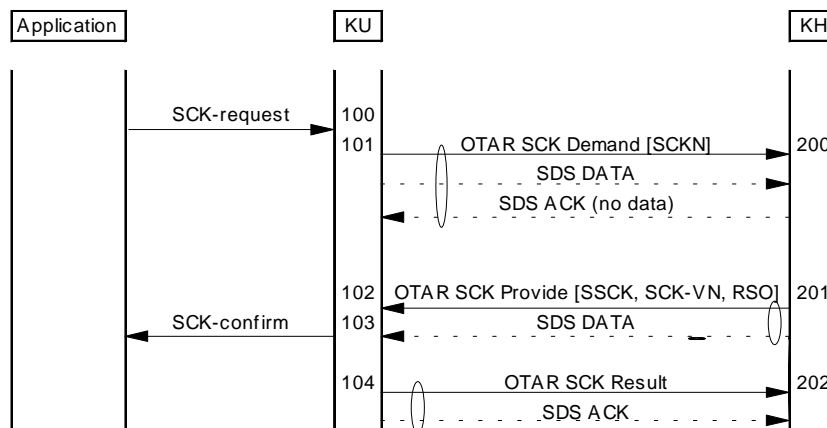
Figure 21: SCK change initiated by KU where KH has key data
