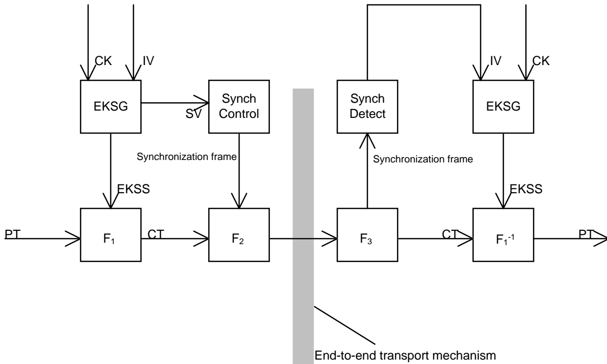
Figure 36: Functional diagram of voice encryption and decryption mechanisms
