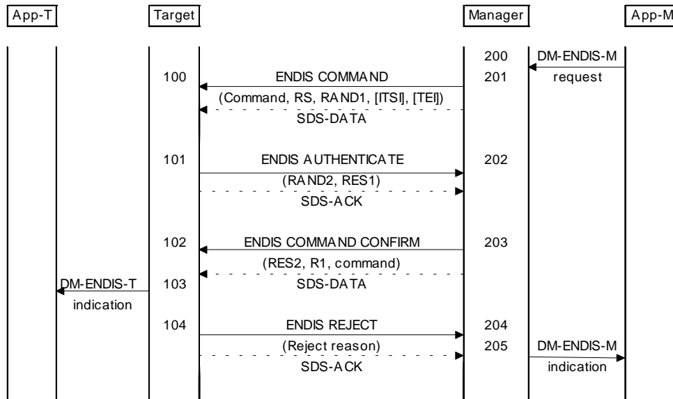
Figure 35: Treating authentication failure during ENDIS exchange
