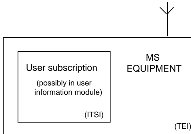
Figure 26: Relationship of TEI and ITSI in DM-MS
