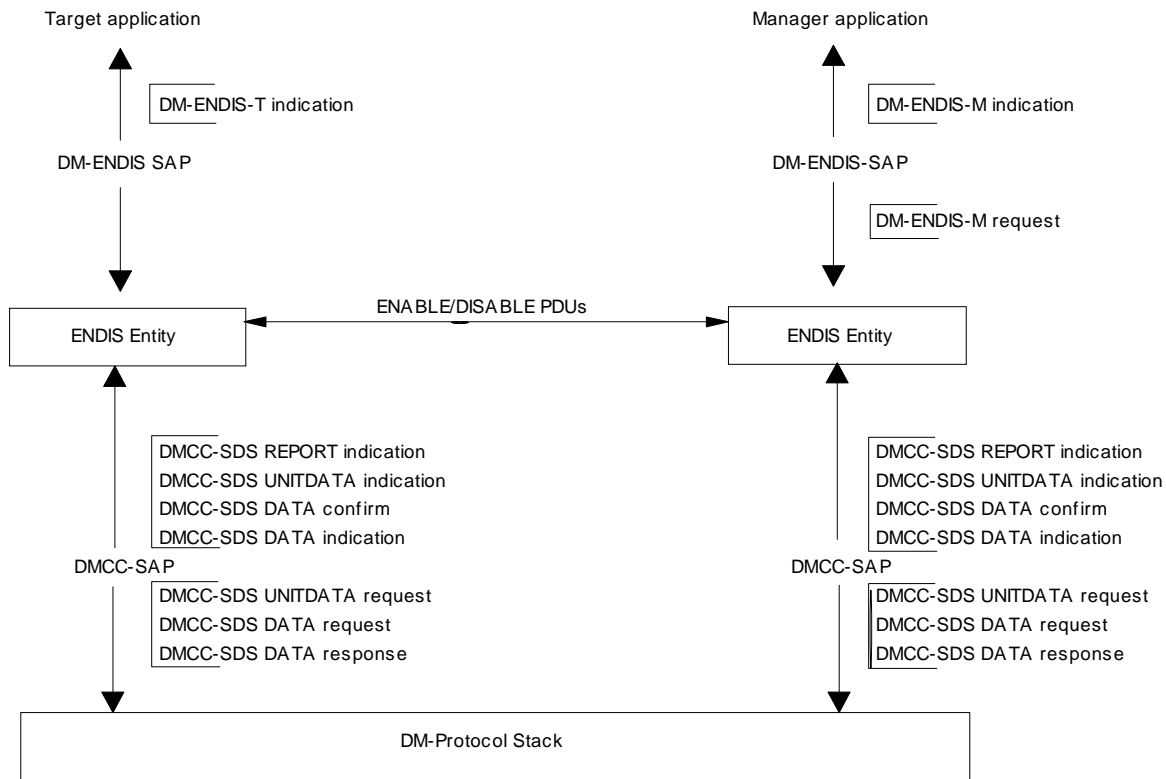
Figure 30: Model for manger to target protocol
