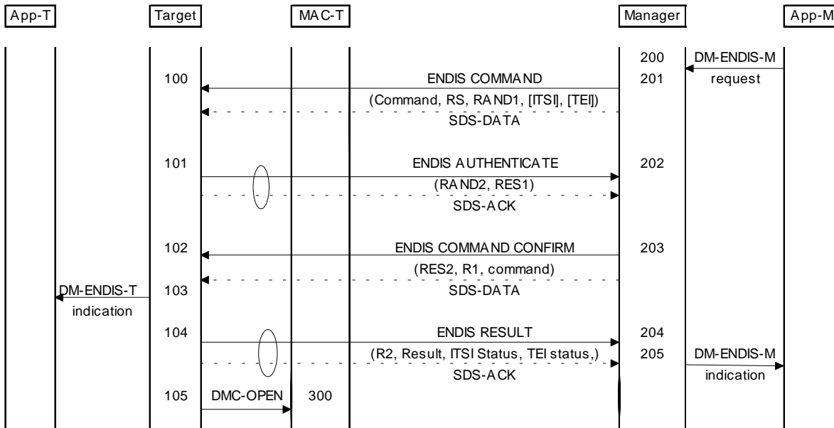
Figure 32: Enabling a target
