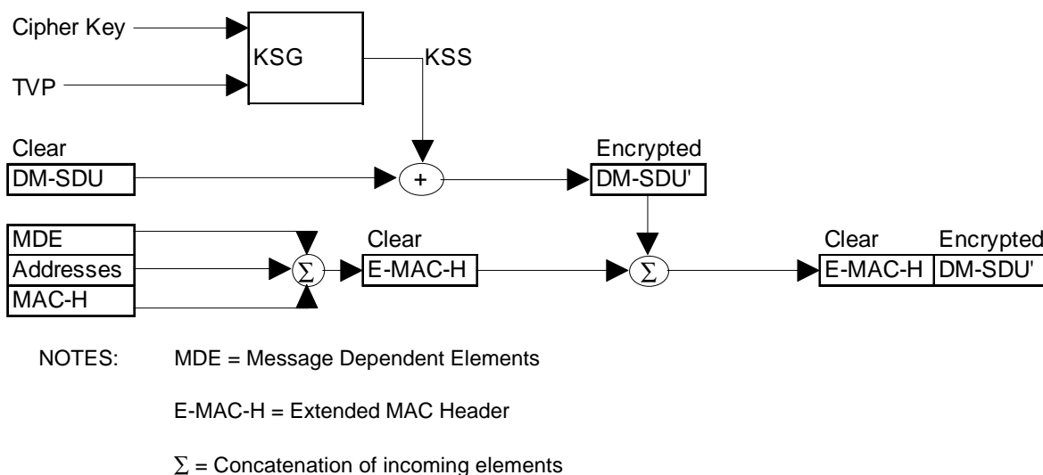
Figure 12: Encryption process as it occurs in TETRA DMO mode 10 2
