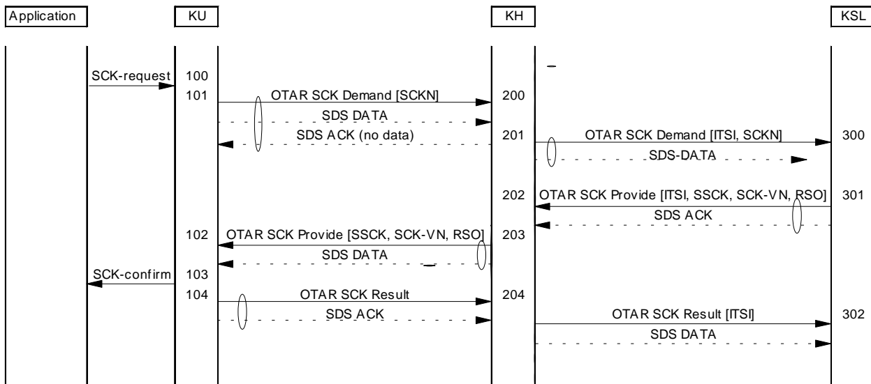
Figure 22: SCK change initiated by KU where KSL has key data
