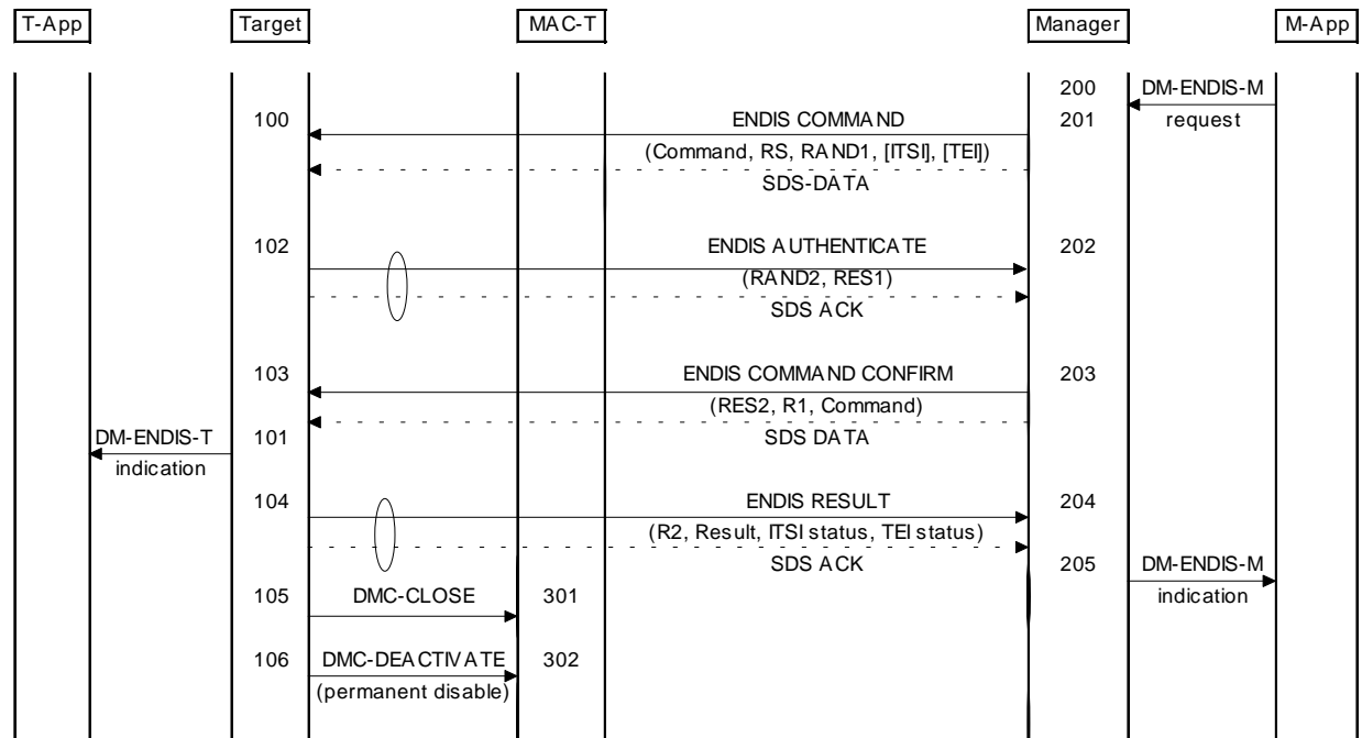
Figure 31: Disabling a target
