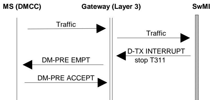
Figure 26: Incoming V+D TX interruption
