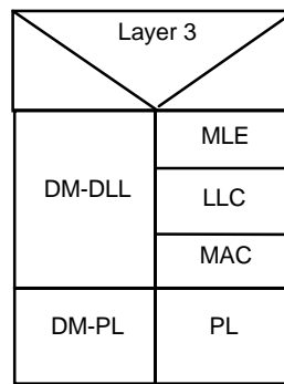
Figure 16: Gateway C-plane protocol stack
