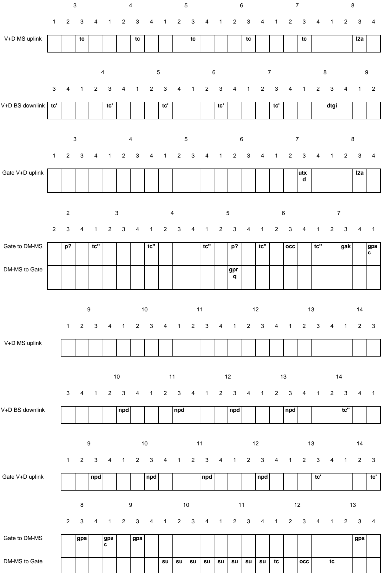
Figure 13: Timing diagram for pre-emption of a call through a DM-GATE
