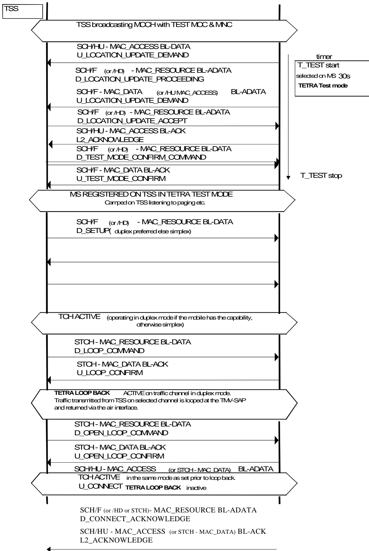
Figure E.3: Outline MSC for TCH loop back
