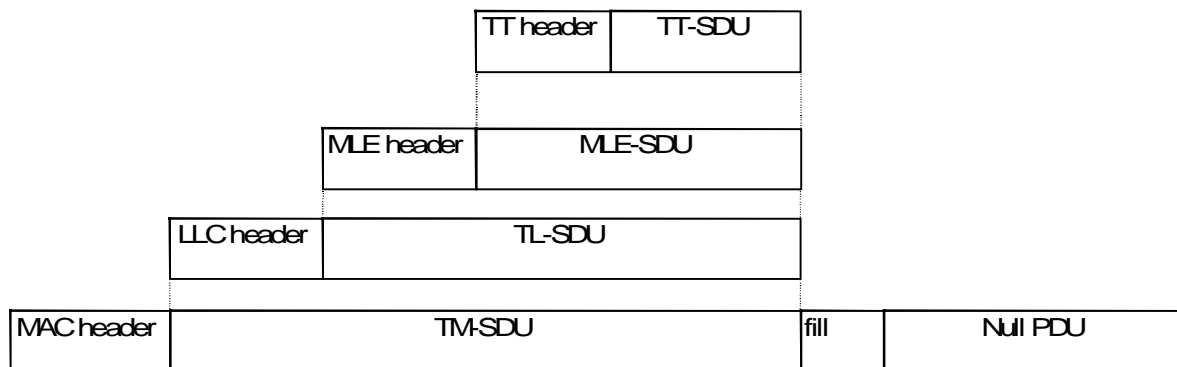
Figure D.3: Relationship between PDUs and SDUs showing how a TT-SDU fits into a MAC block
