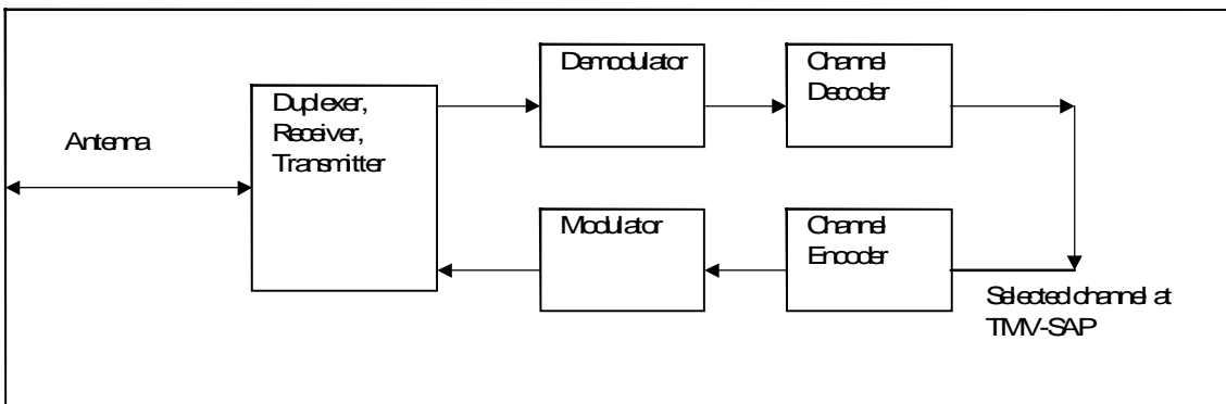
Figure E.2: Simplified diagram of MS during RF Loop Back
