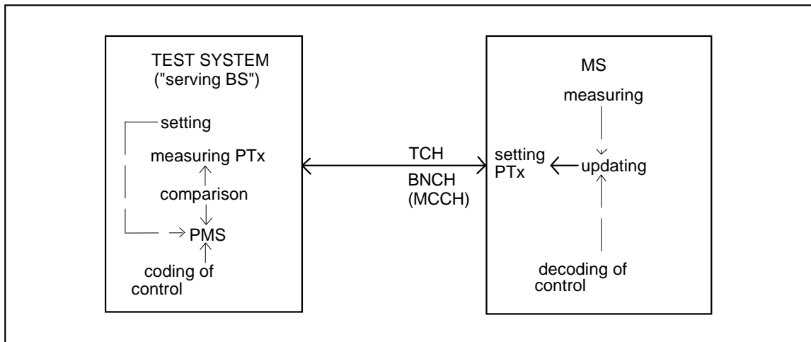
Figure 2: MS link control test scenario
