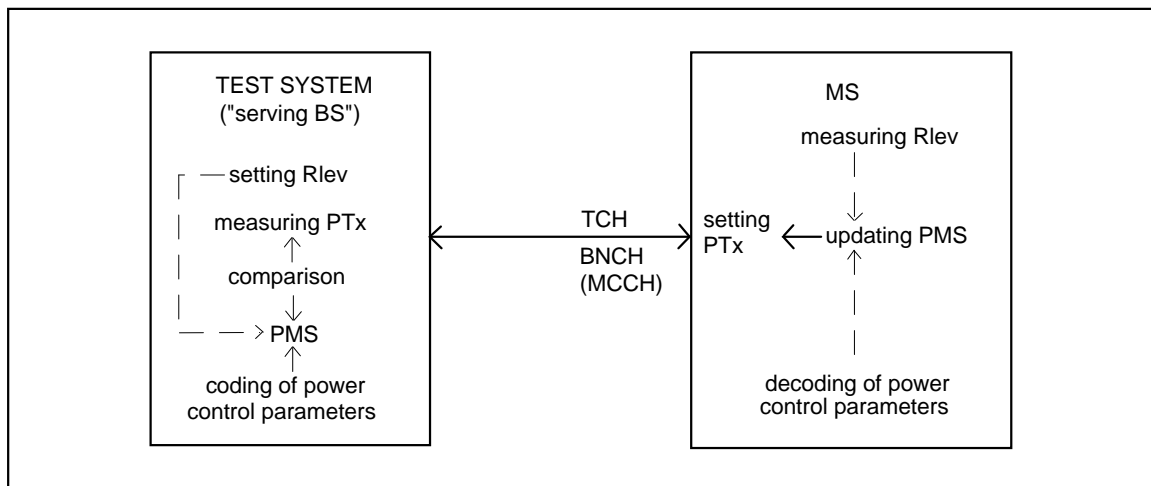
Figure 3: MS link control test scenario
