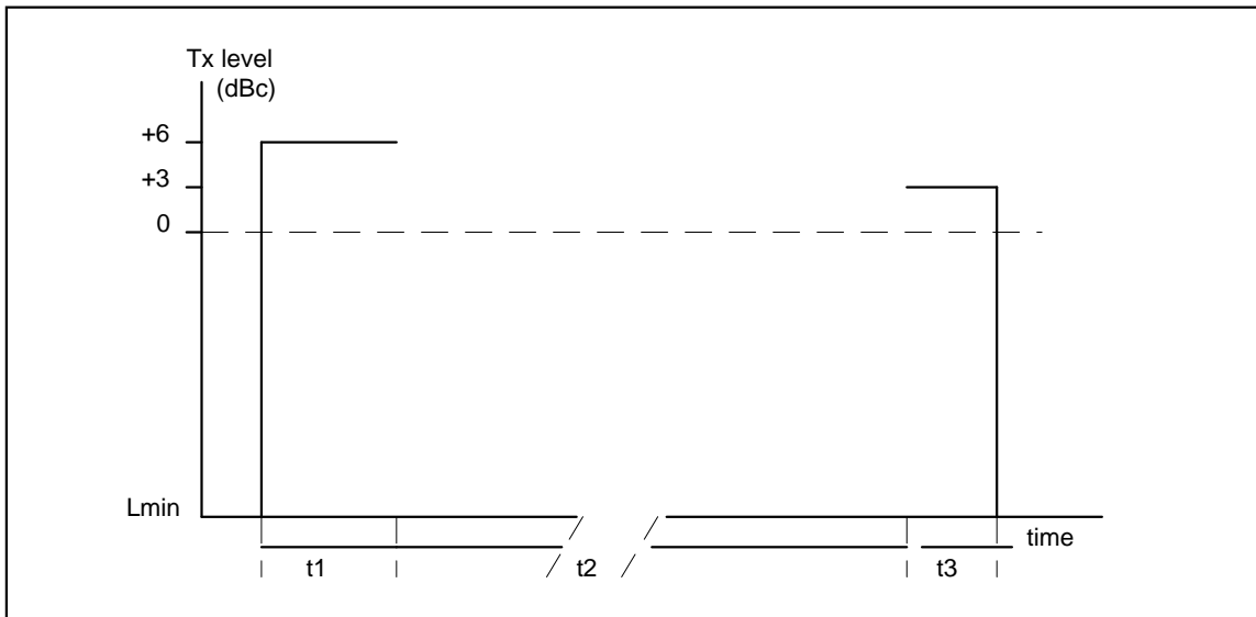
Figure 2: Power time mask of transmitted burst
