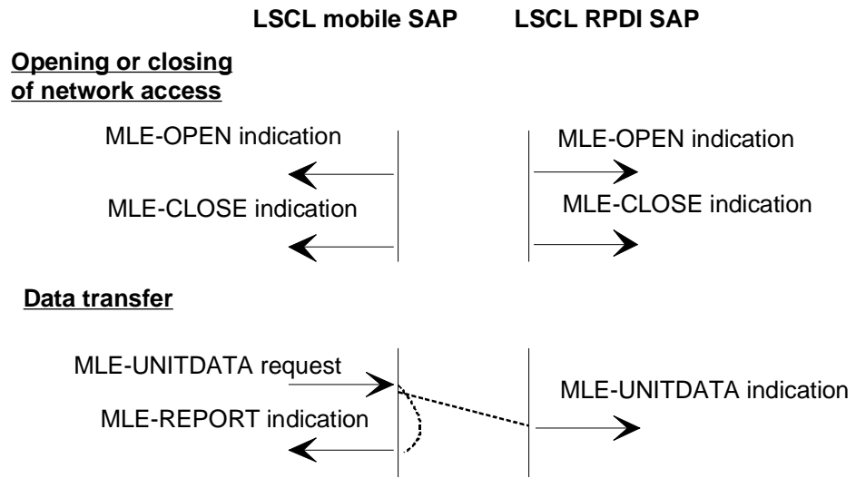
Figure 62: Primitive time sequence at the LSCL-SAP
