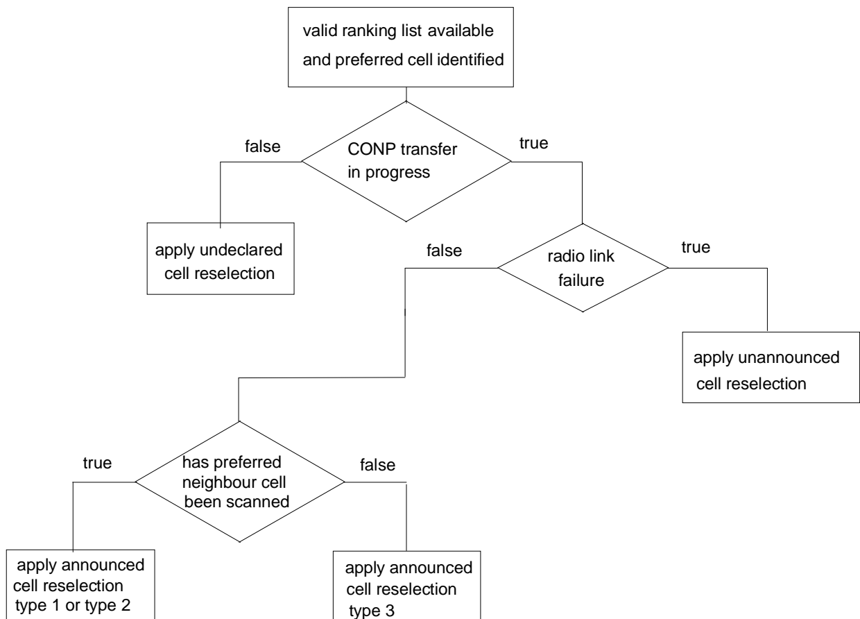
Figure 65: Decision tree to choose re-selection type
