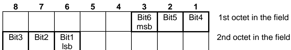
Figure 34: Field mapping
