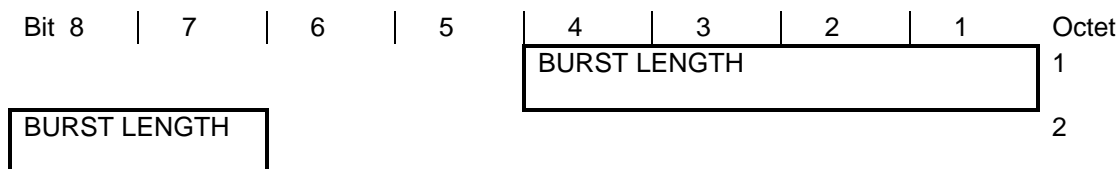
Figure 104: Burst length field
