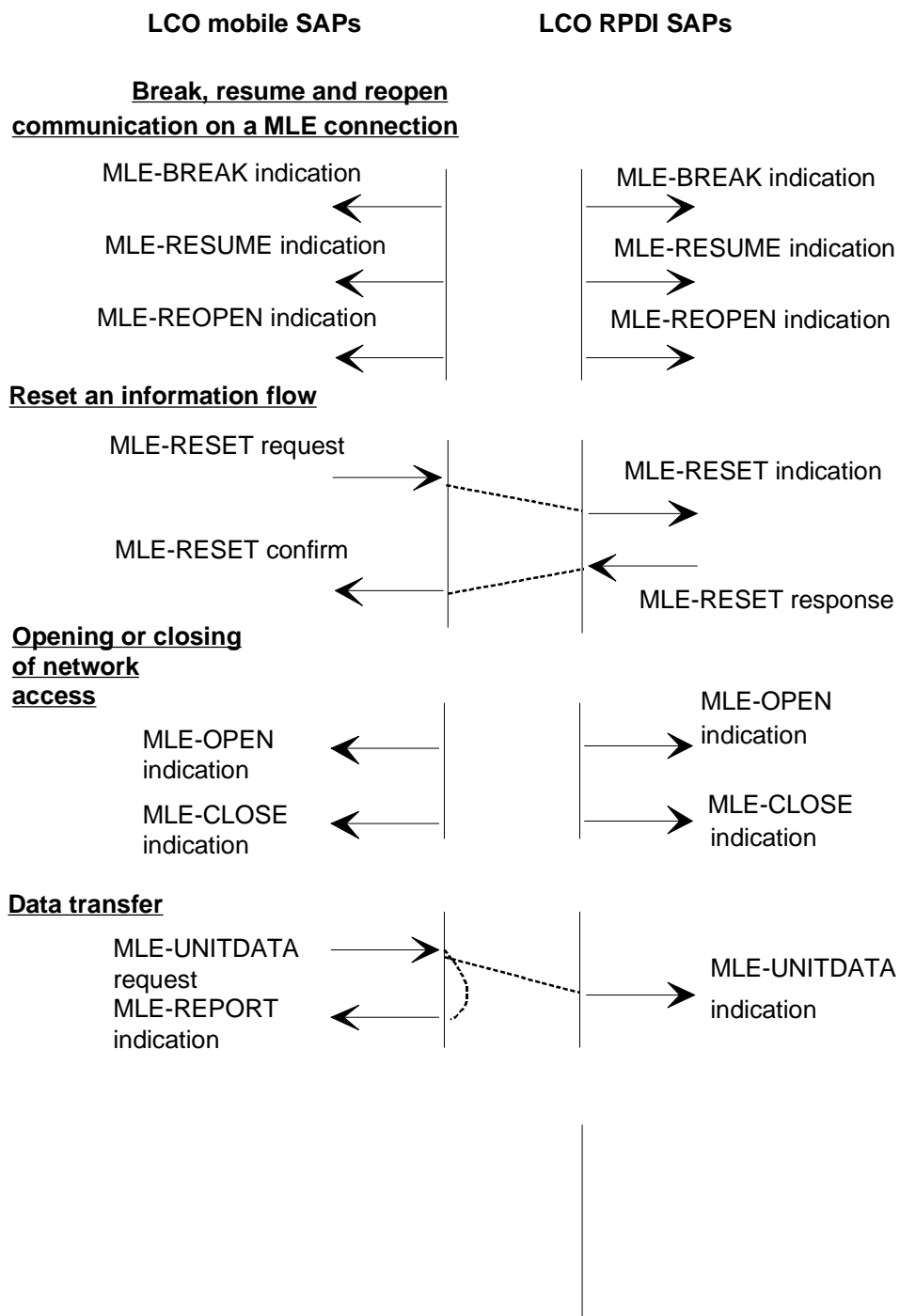
Figure 63: Primitive time sequence at the LCO-SAP
