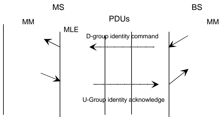
Figure 53: Procedure for group identity download
