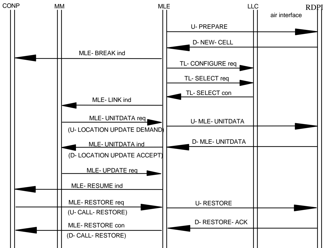
Figure 68: Announced type 2 cell re-selection procedure
