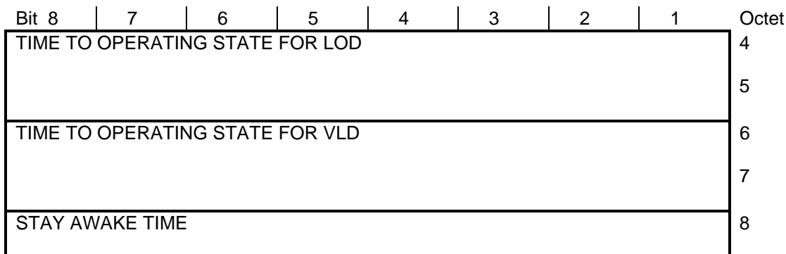
Figure 125: Wake interval parameters element
