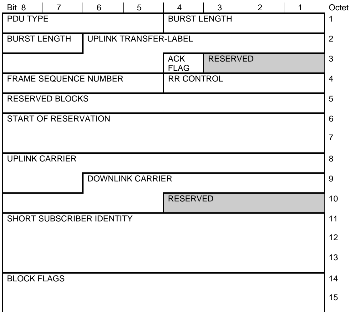
Figure 83: <DR3> PDU
