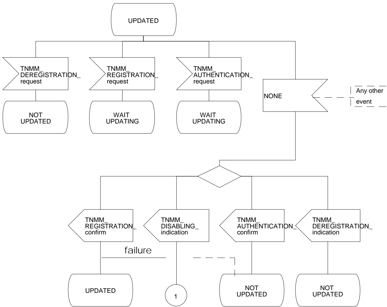
Figure 44: MM service state diagram (sheet 3 of 4)
