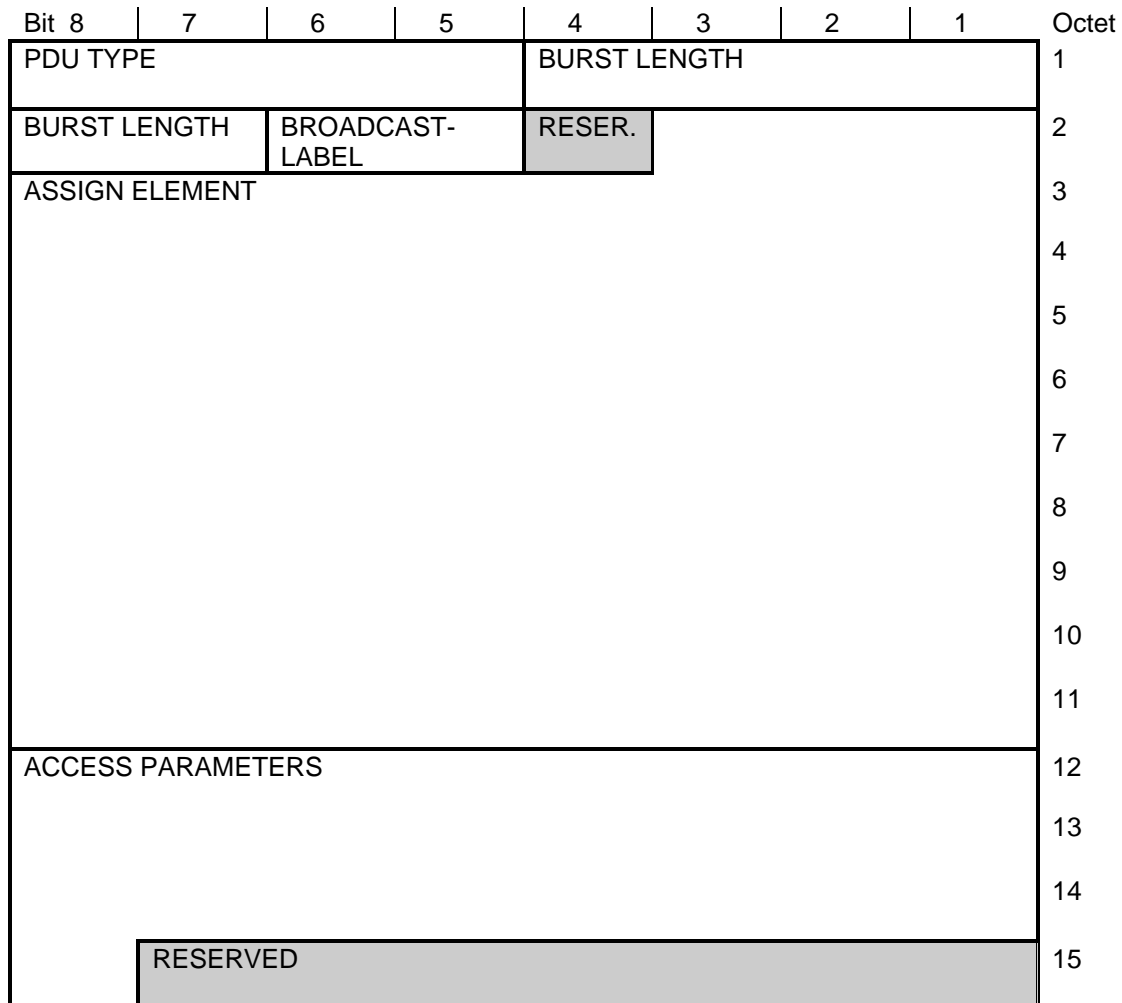
Figure 88: <AP> PDU
