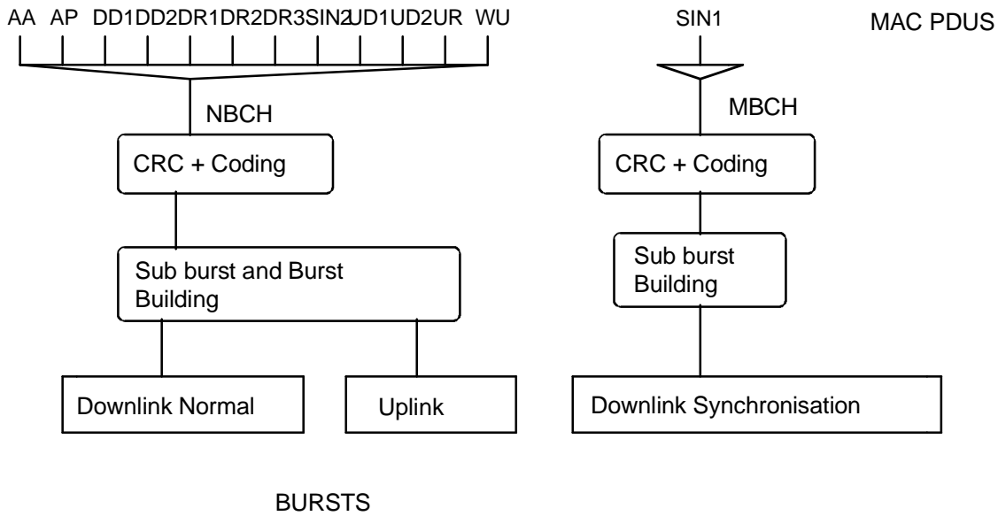
Figure 11: The NBCH and MBCH channels
