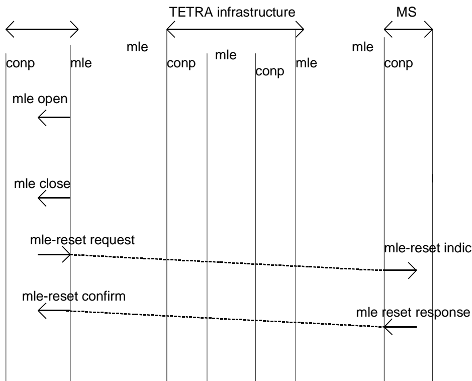
Figure 28: Access to resources and reset protocol sequence
