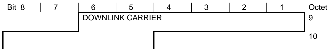
Figure 107: Downlink carrier
