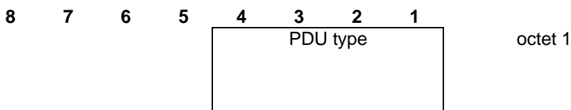
Figure 36: Type field
