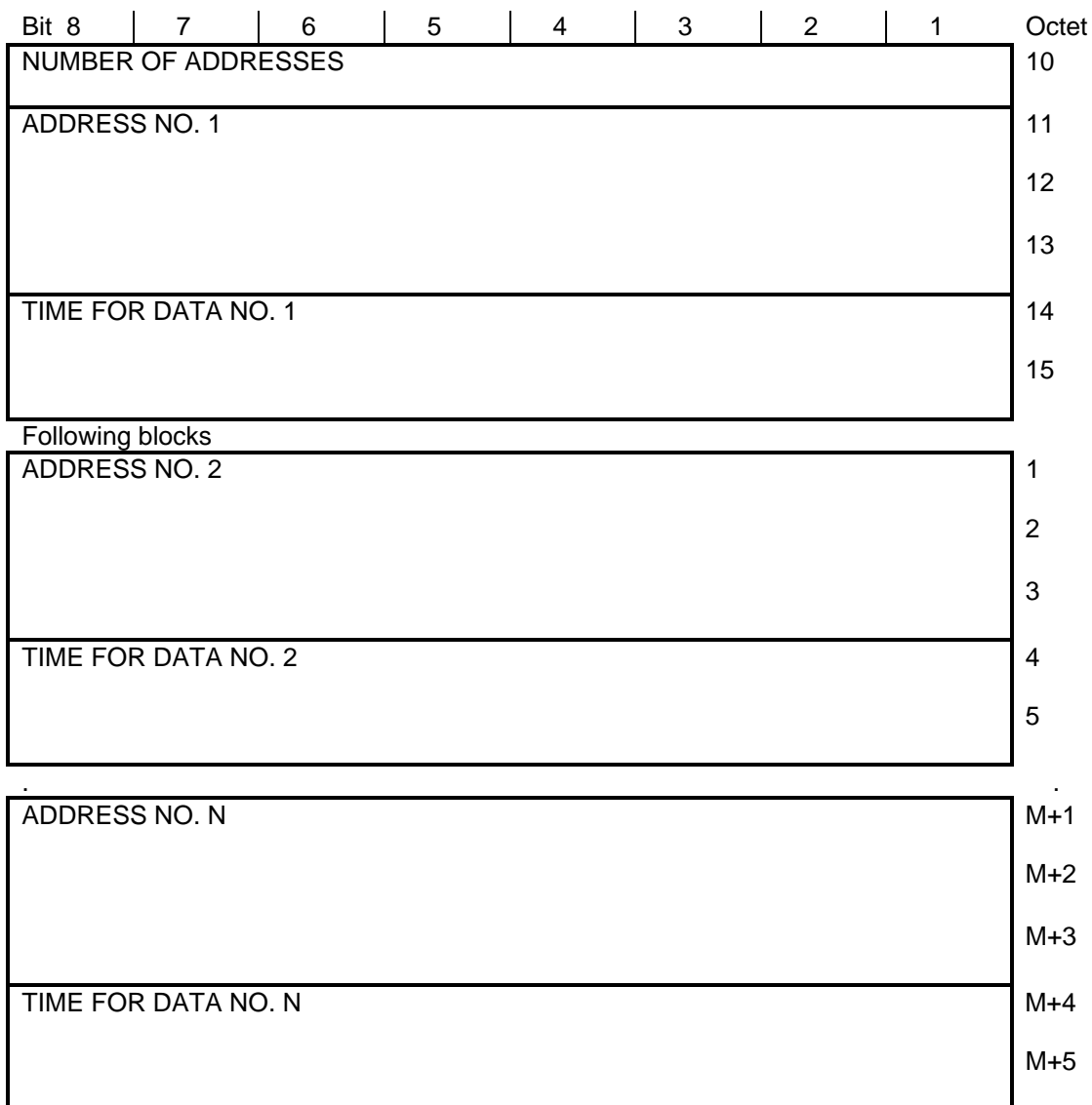
Figure 122: Traffic list element
