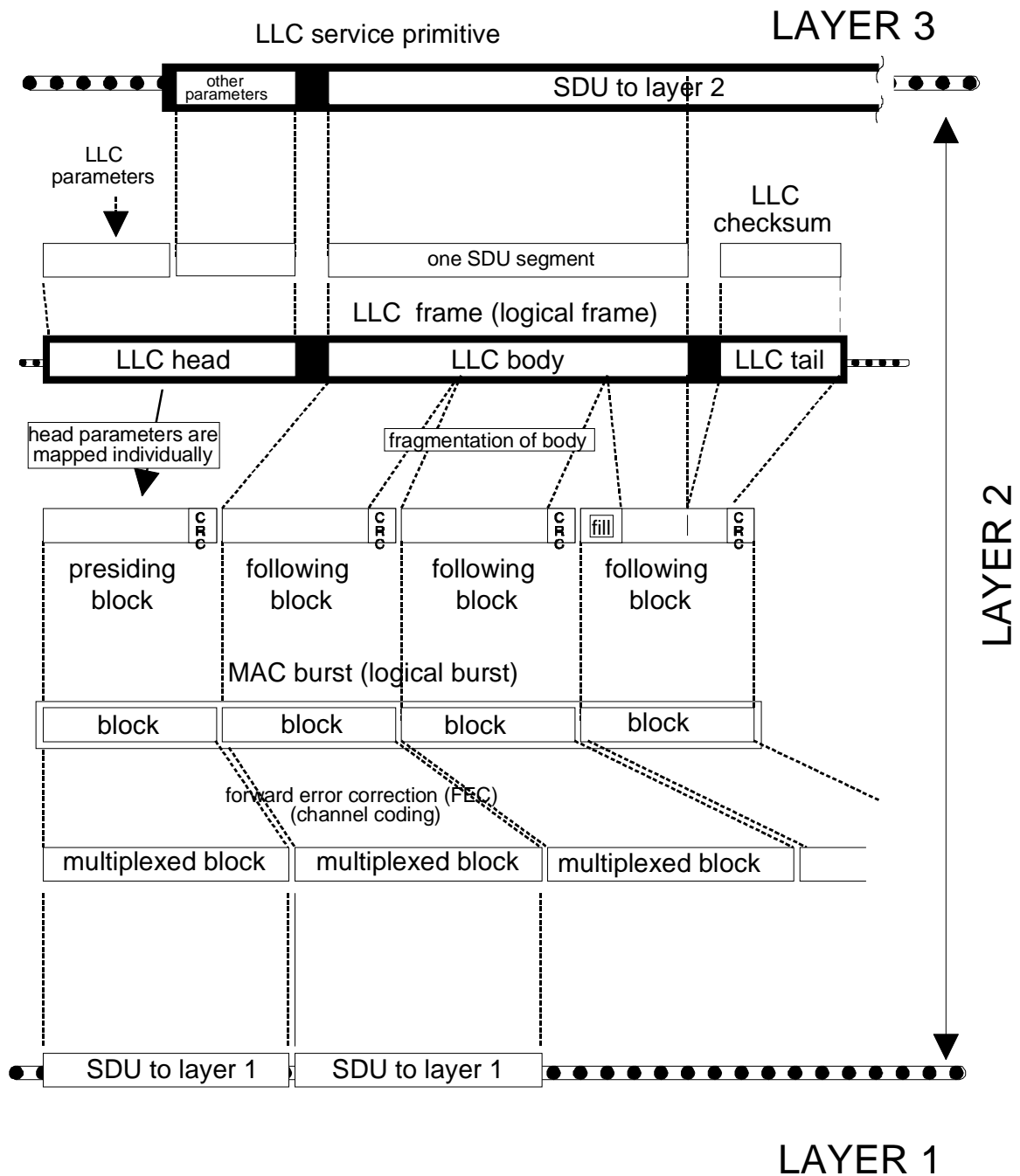
Figure 127: Layer 2 Data Structures
