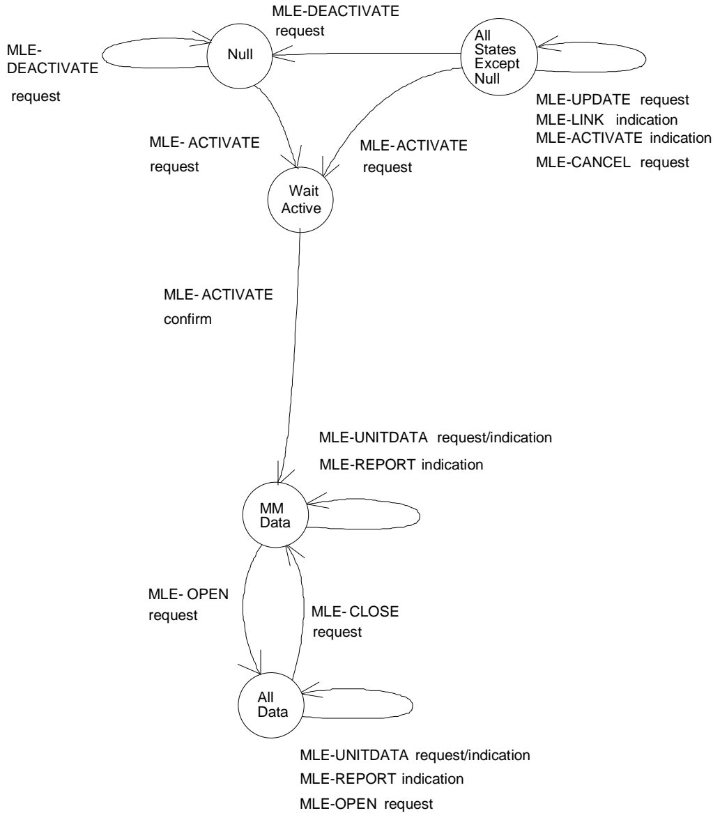
Figure 57: LMM-m SAP state transition diagram
