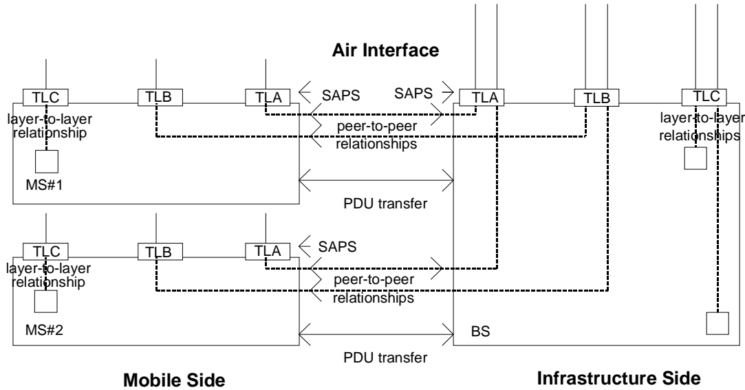
Figure 70: Services relationships offered by the layer 2 over the air interface
