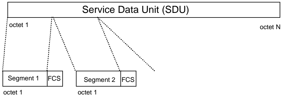
Figure 128: Segmentation
