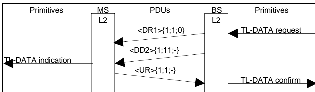
Figure J.13: Acknowledged downlink transfer. Data on another carrier than ACCH
