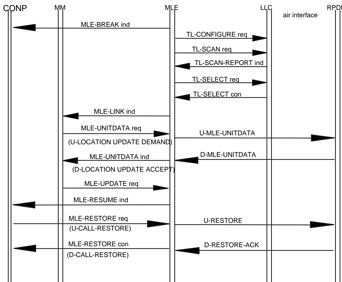
Figure 66: Unannounced cell re-selection procedure
