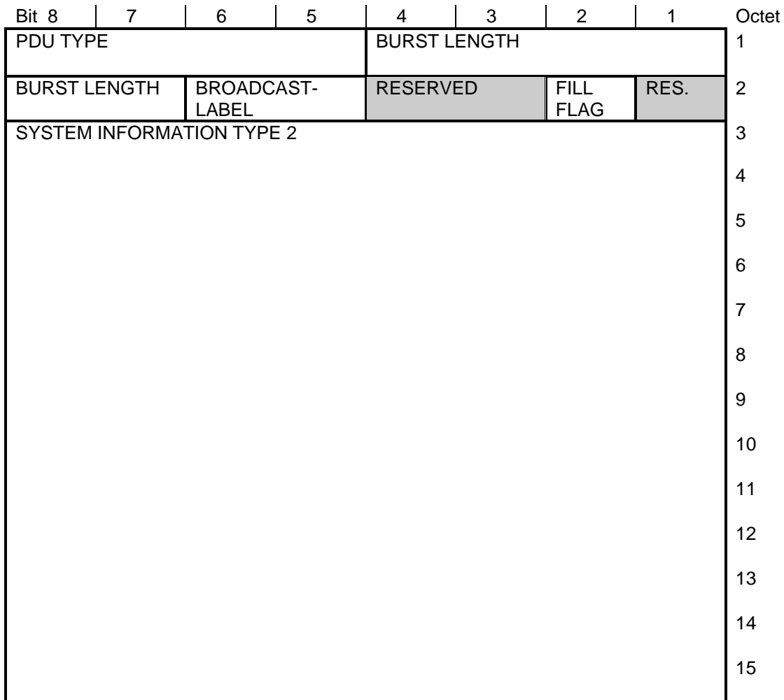
Figure 89: <SIN2> PDU
