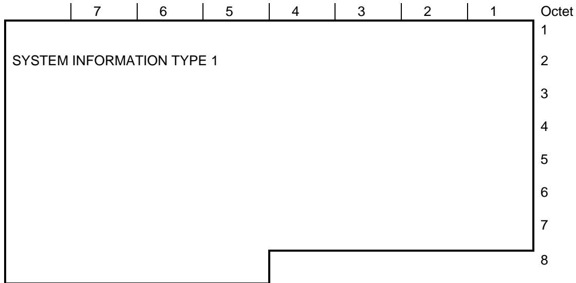
Figure 90: <SIN1> PDU
