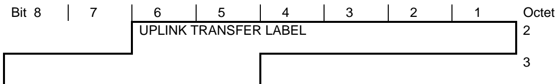
Figure 124: Uplink transfer label
