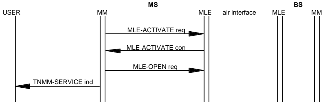
Figure 47: MM Activation procedure, Registration not supported
