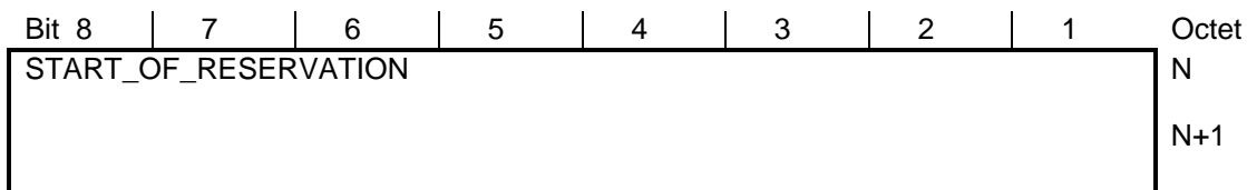
Figure 121: Start of reservation
