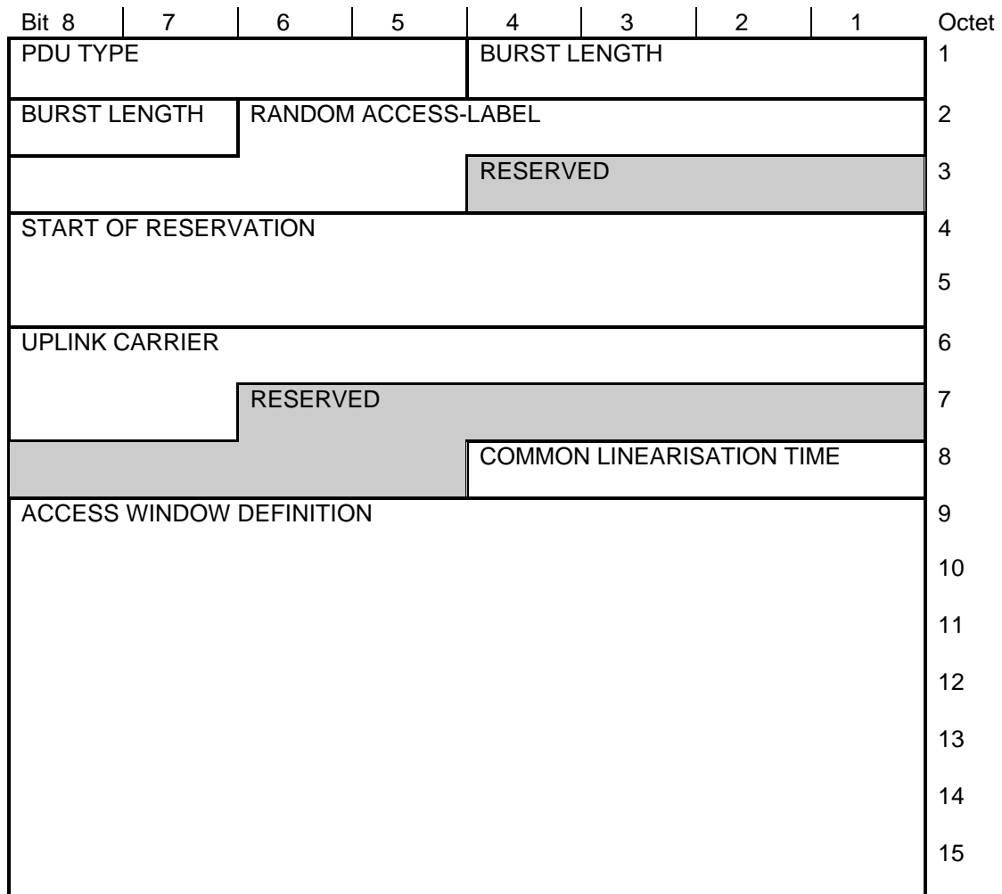
Figure 84: <AA> PDU
