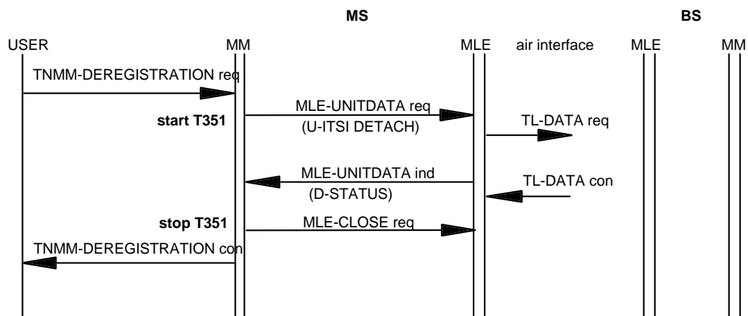
Figure 51: De-registration of MS (Detach)
