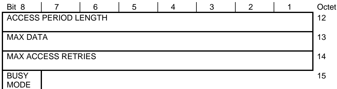
Figure 92: Access parameters element
