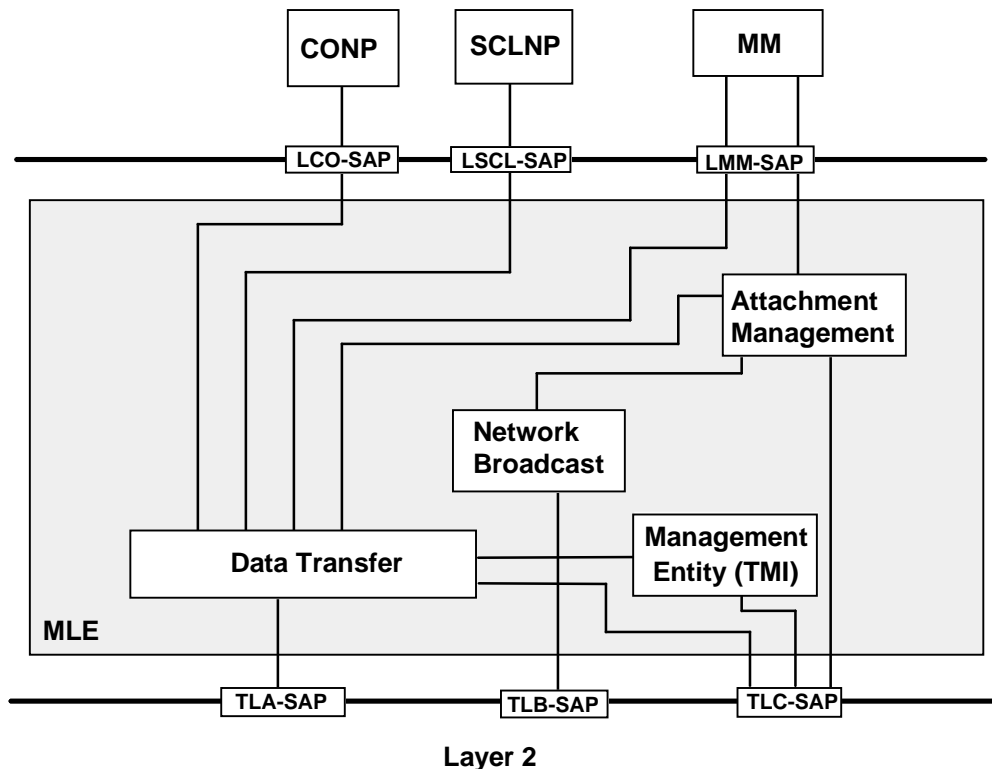
Figure 64: MLE functional model
