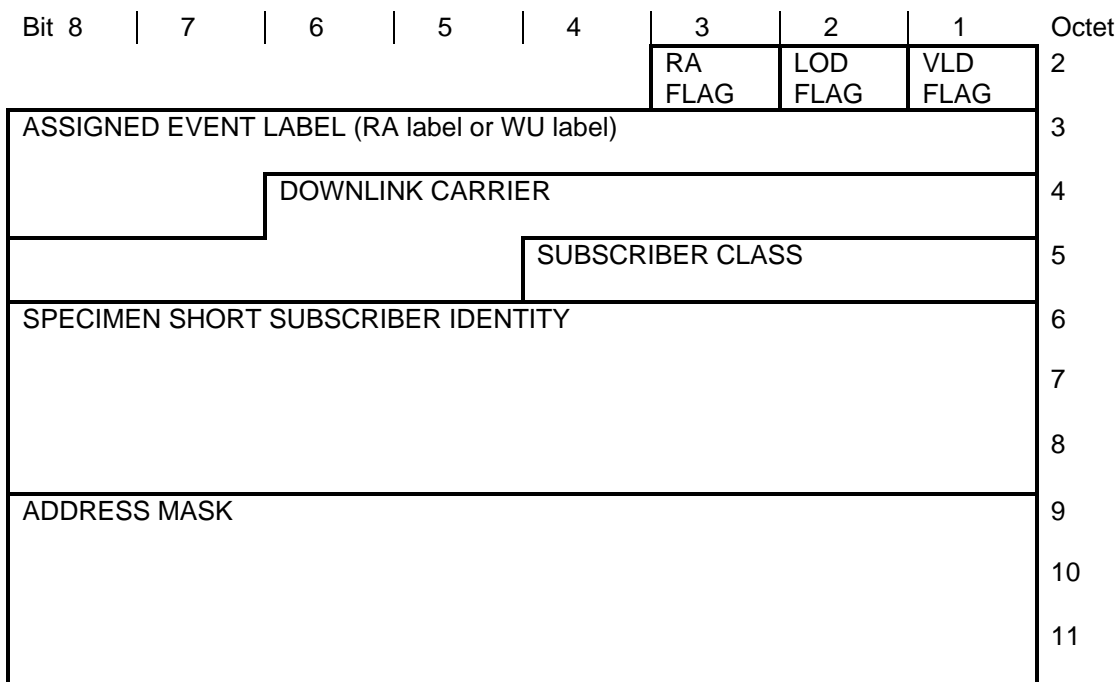
Figure 101: Assign element
