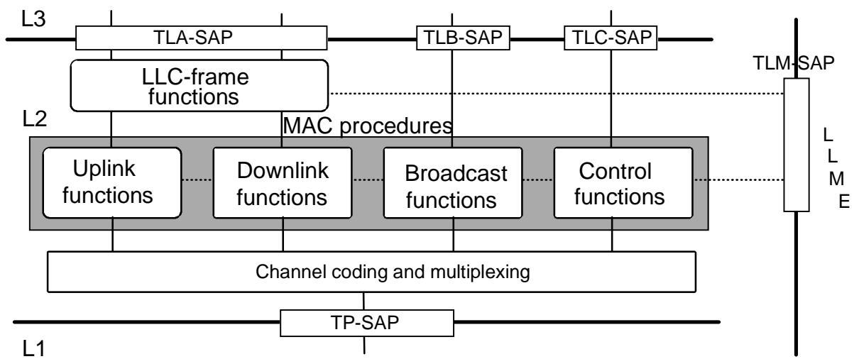
Figure 129: Grouping of layer 2 functions
