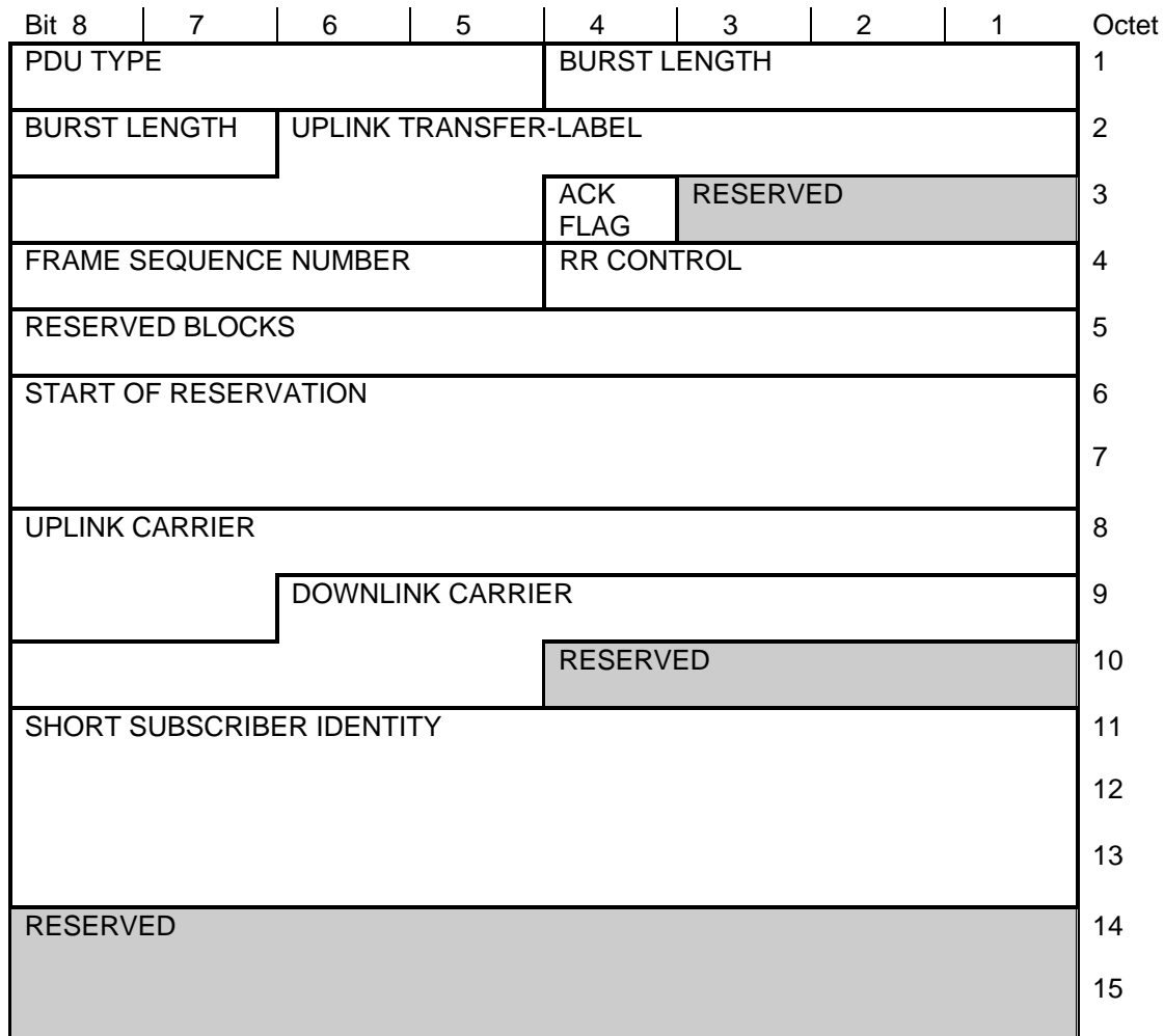
Figure 81: <DR1> PDU
