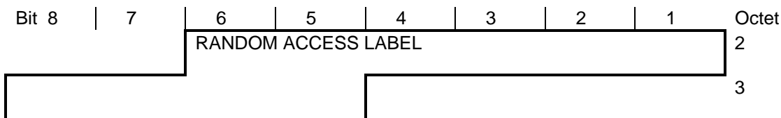
Figure 118: Random access label
