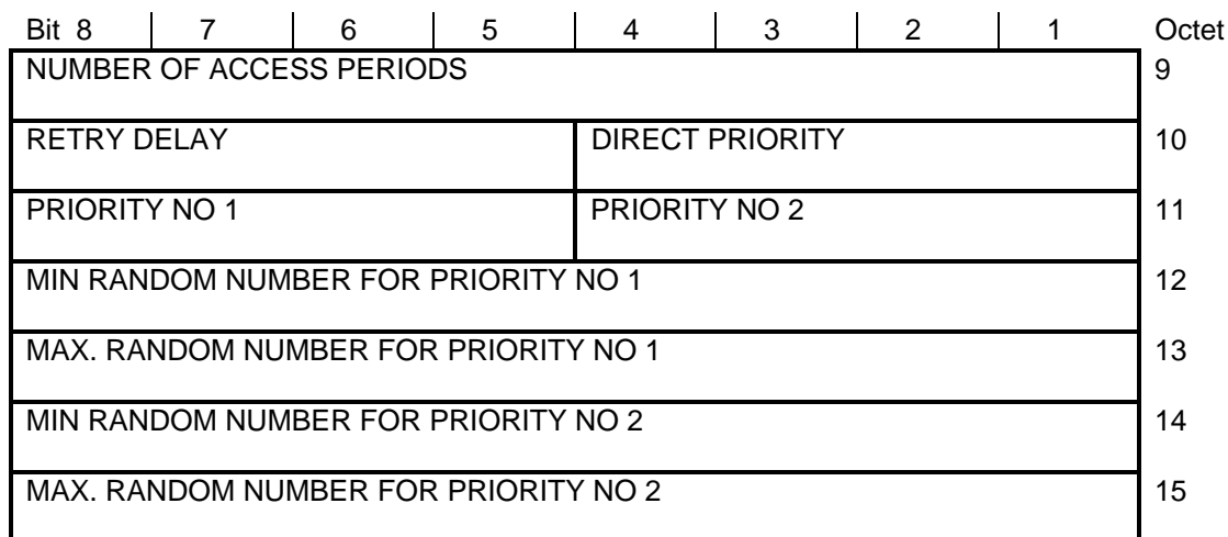
Figure 93: Access window definition element
