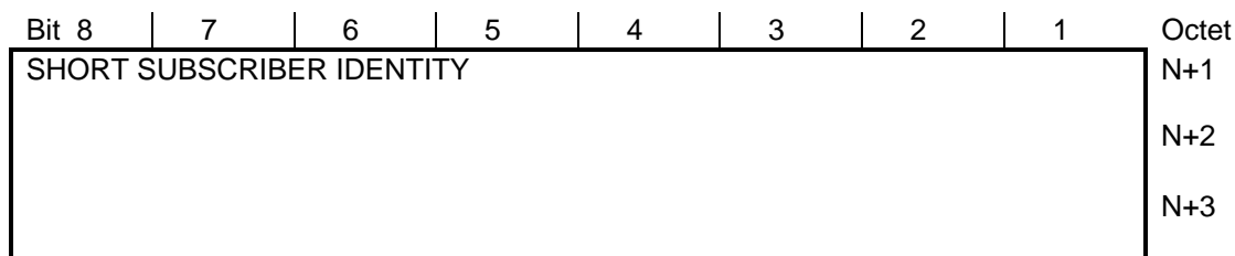
Figure 120: SSI
