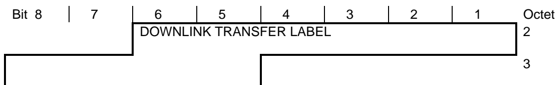
Figure 108: Downlink transfer label
