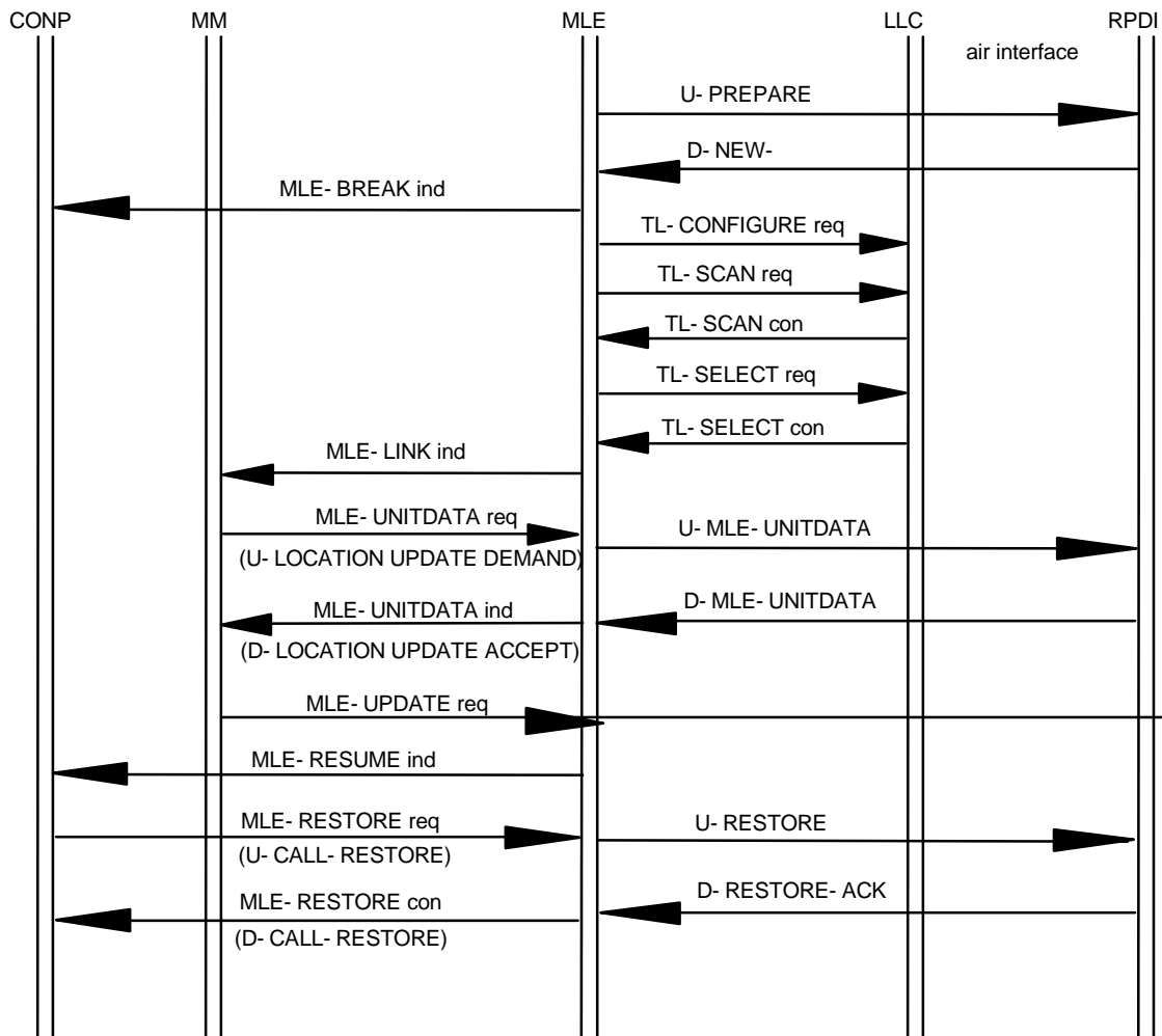
Figure 67: Announced type 3 cell re-selection procedure
