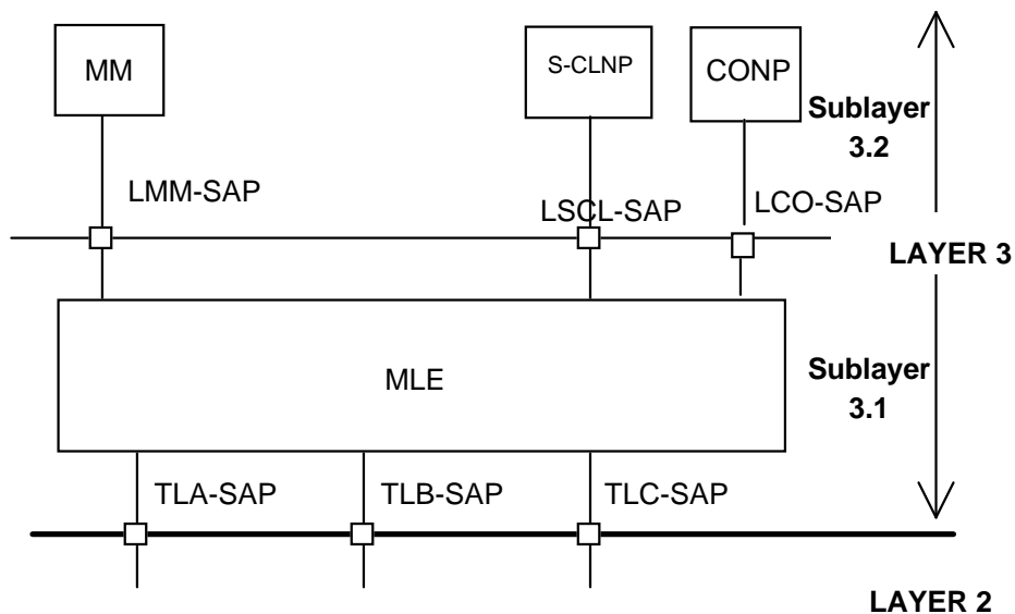
Figure 60: The MLE (sub-layer 3.1) in the MS protocol stack
