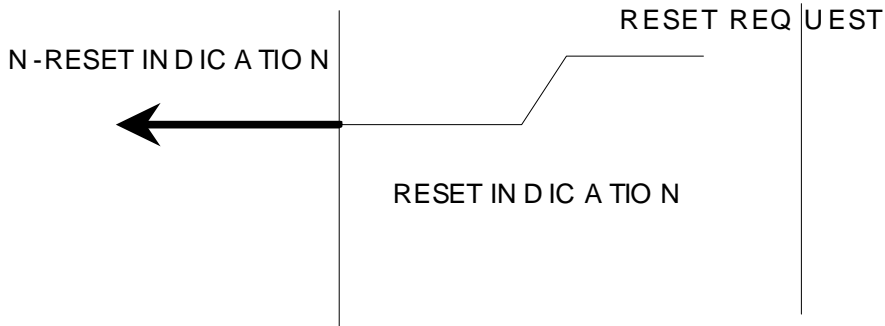
Figure 22: Reset scenario
