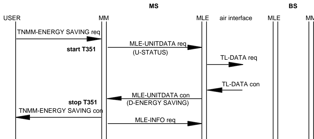
Figure 52: Change energy economy mode
