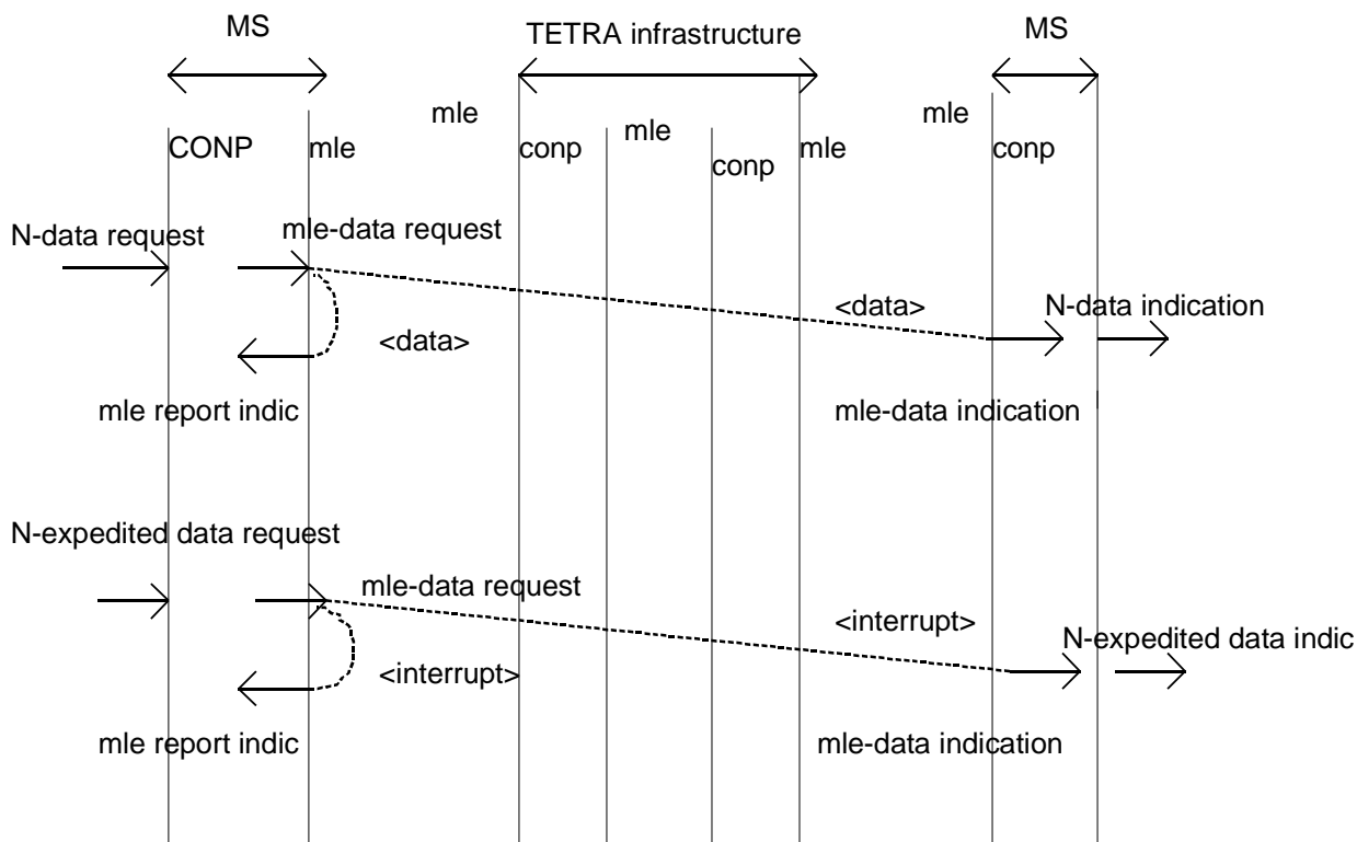
Figure 27: Data and interrupt transfer protocol sequence
