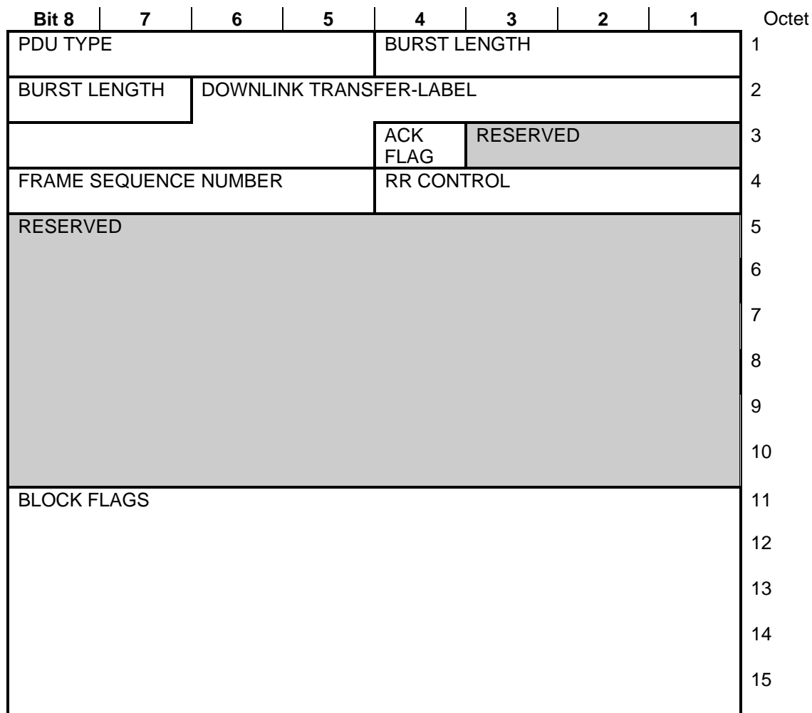
Figure 78: <UR> PDU
