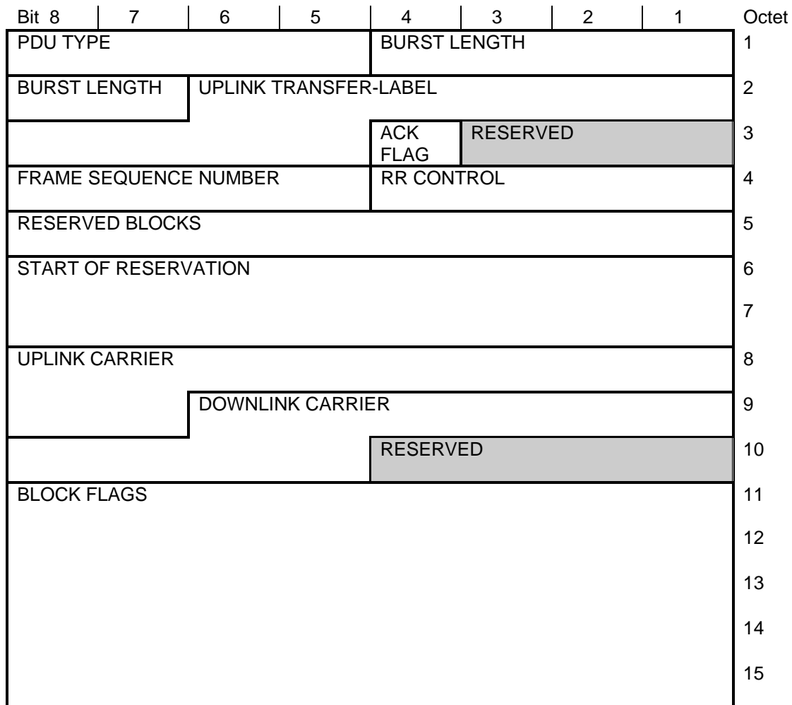
Figure 82a: <DR2> PDU
