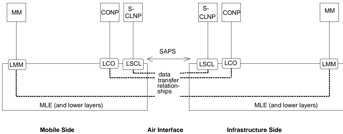
Figure 55: Services relationships offered by the MLE in the air interface
