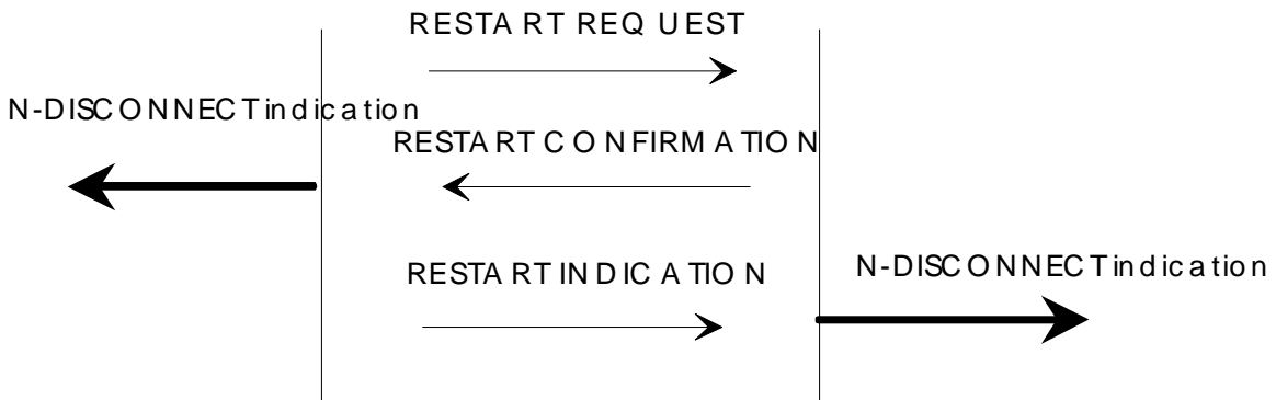
Figure 23: Error detected and reset scenario
