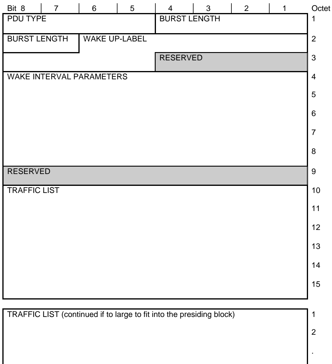
Figure 87: <WU> PDU
