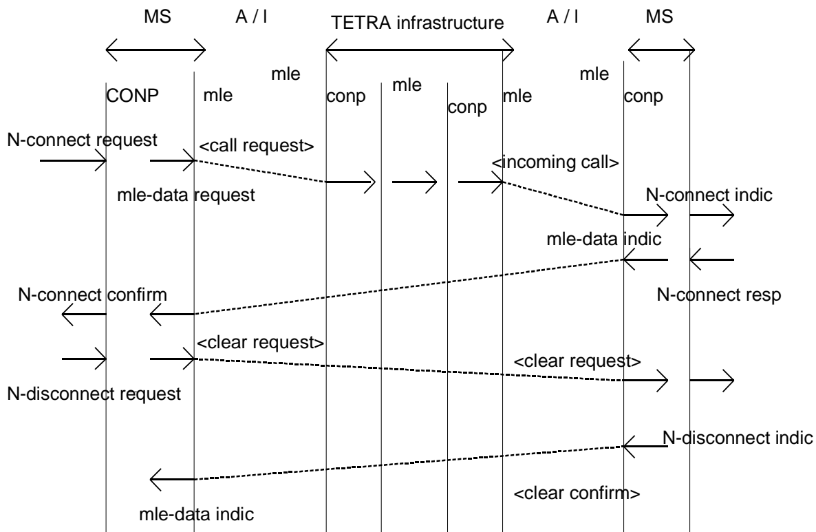
Figure 26: Connection and disconnection protocol sequence
