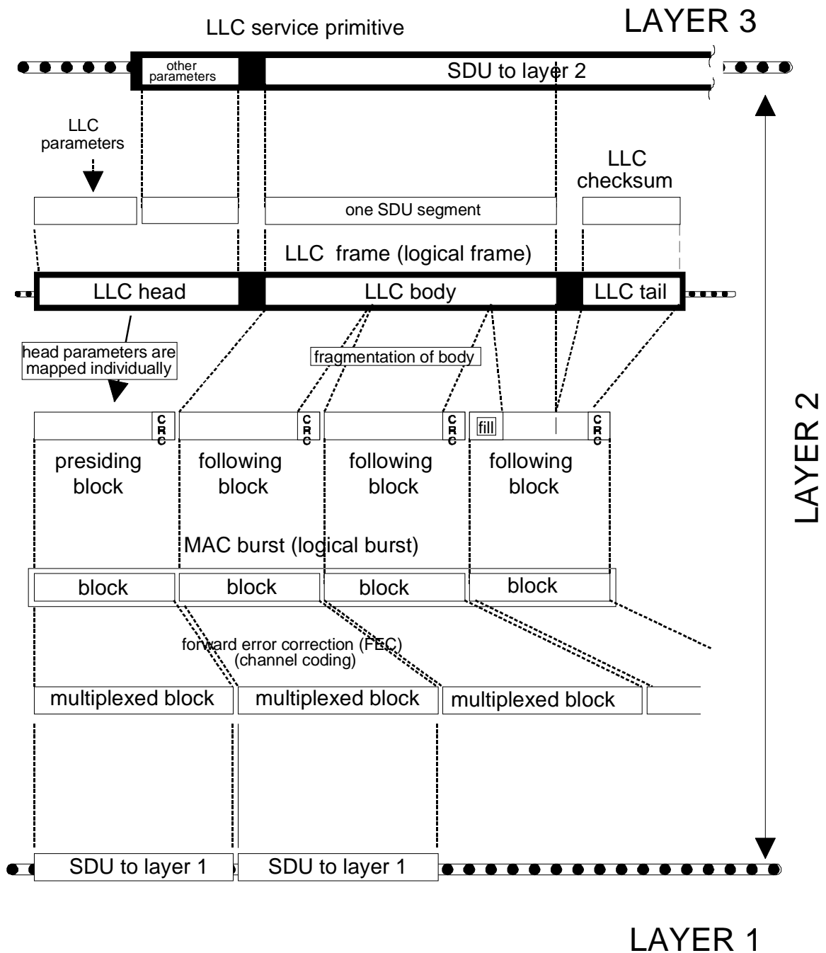
Figure 130: Layer 2 data structures
