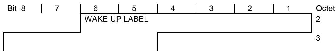
Figure 126: Wake up label
