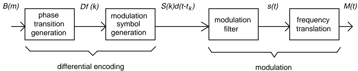
Figure 5: Block diagram of the modulation process
