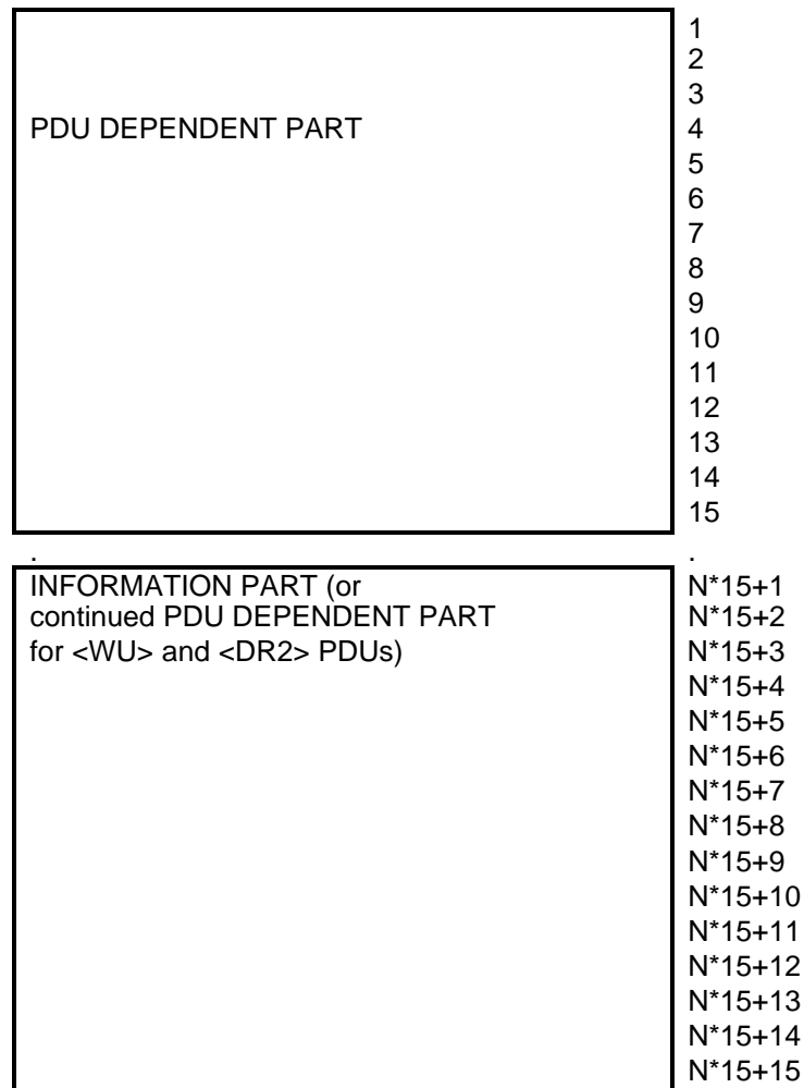
Figure 76: Structure of a variable length PDU, with N the number of following blocks
