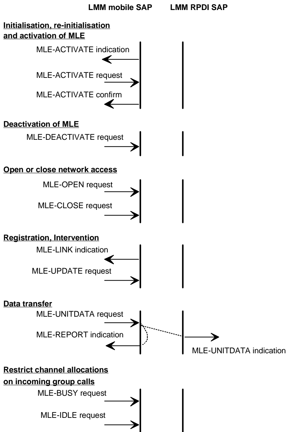
Figure 61: Primitive time sequence at the LMM-SAP
