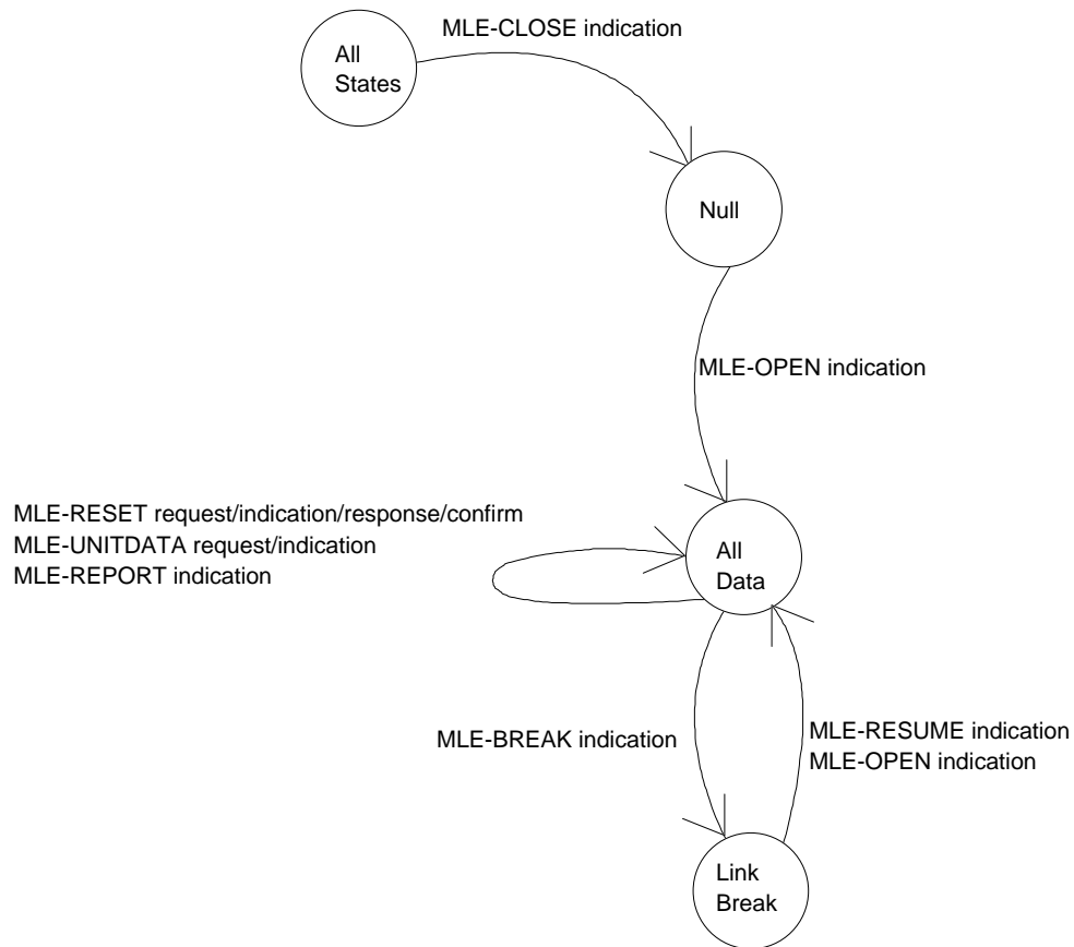
Figure 59: State transition diagram of LCO SAP
