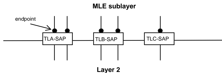
Figure 69: SAPs between Layer 2 and MLE
