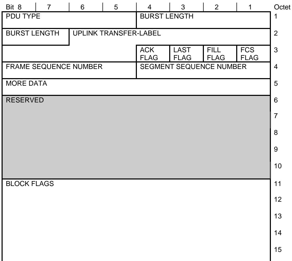
Figure 80: <UD2> PDU
