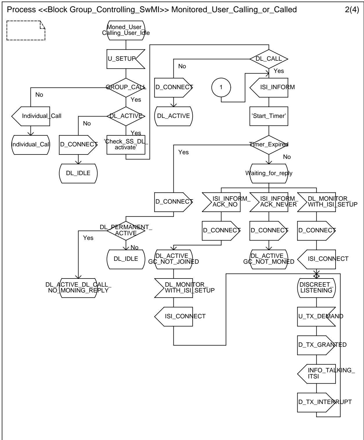
Figure A.2 (sheet 2 of 4): Group controlling SwMI SDL Monored user is the calling user
