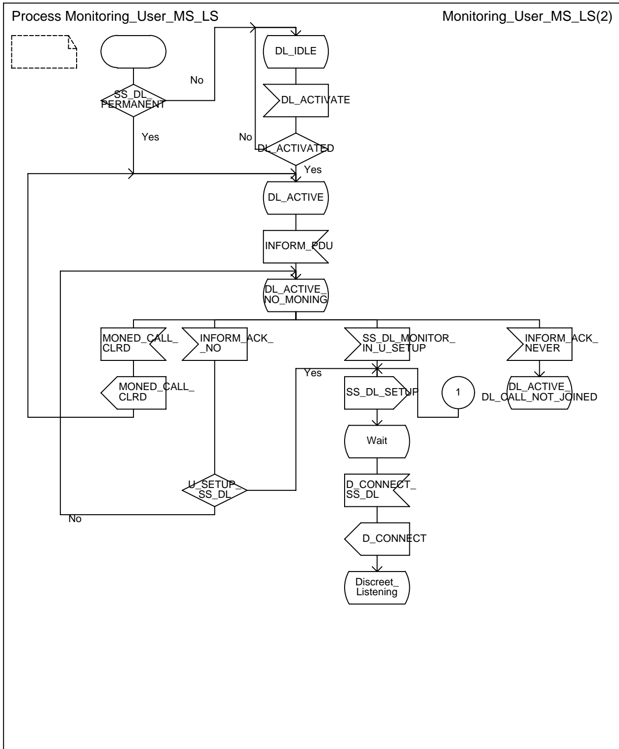
Figure A.1(sheet 1 of 2): Monitoring user MS/LS SDL
