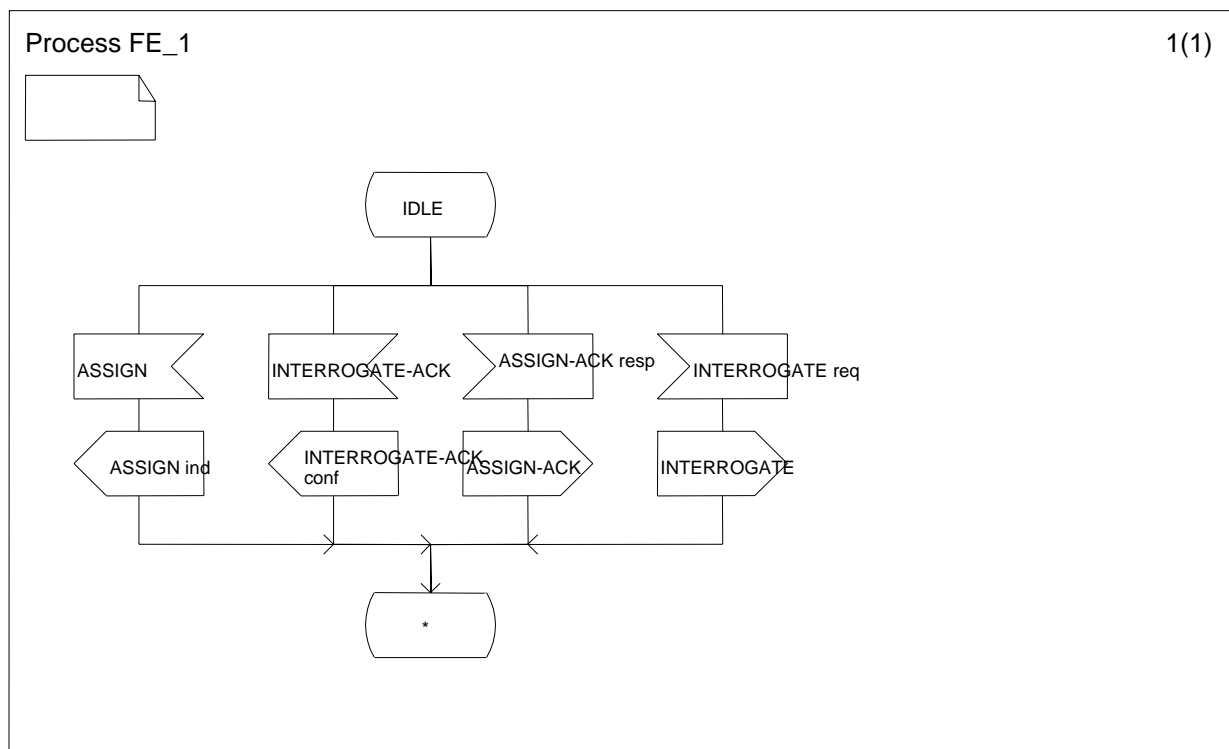
Figure 2: Process description for FE1
