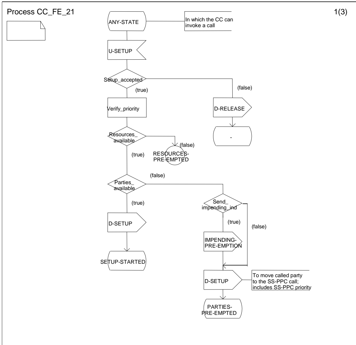
Figure 8: Process description for CC to which FE21 is collocated
