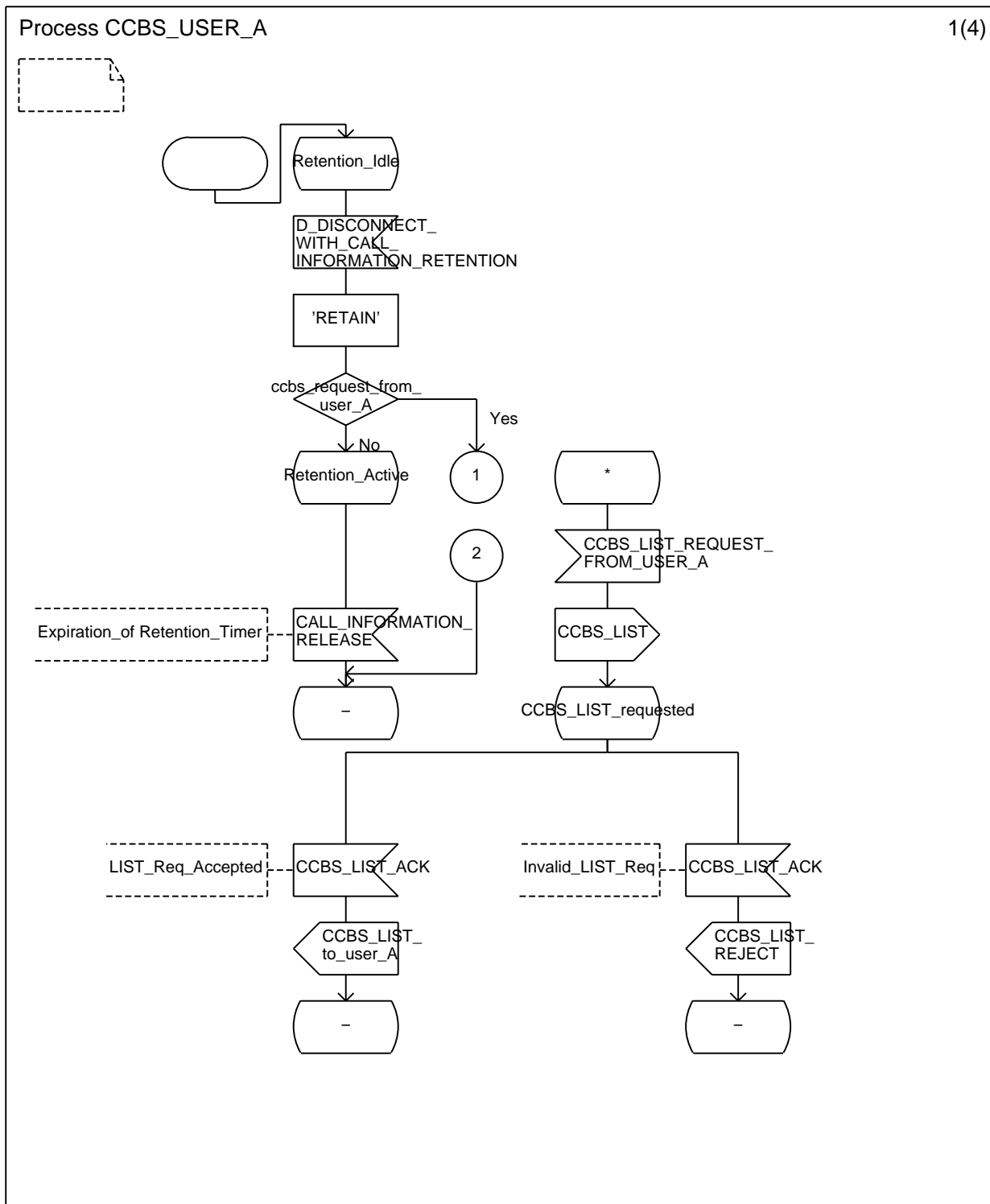
Figure A.3: CCBS Served User (User A MS/LS) process (sheet 1 of 4)
