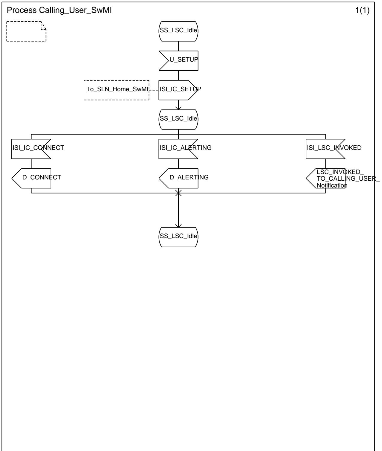
Figure A.2: Calling user A SwMI SDL
