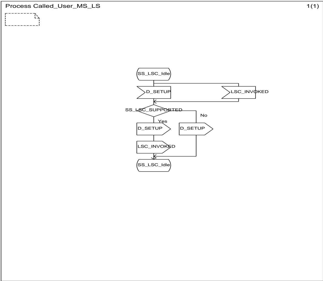
Figure A.7: Called user (attendant n) MS/LS SDL
