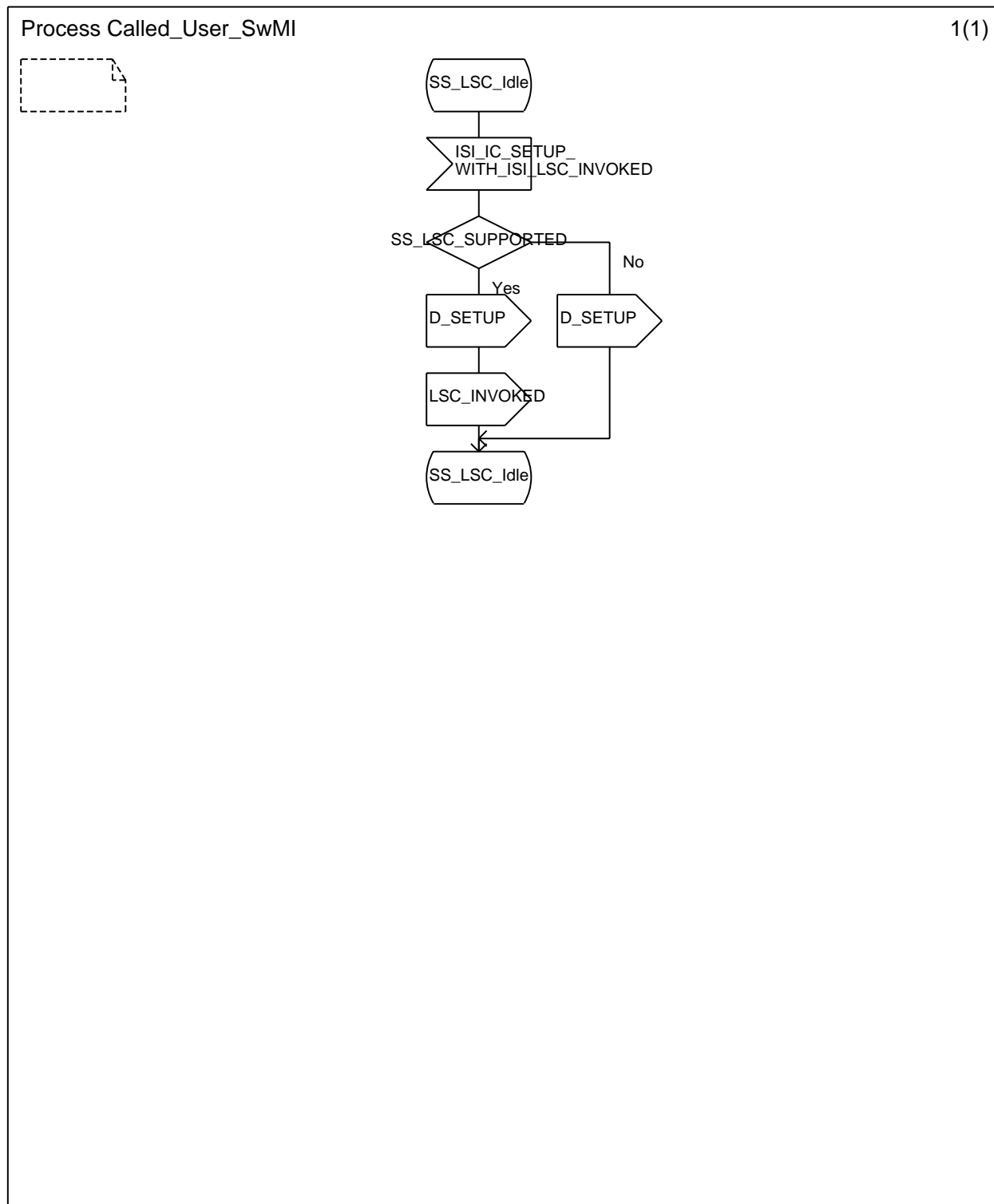
Figure A.6: Called user (attendant n) SwMI SDL
