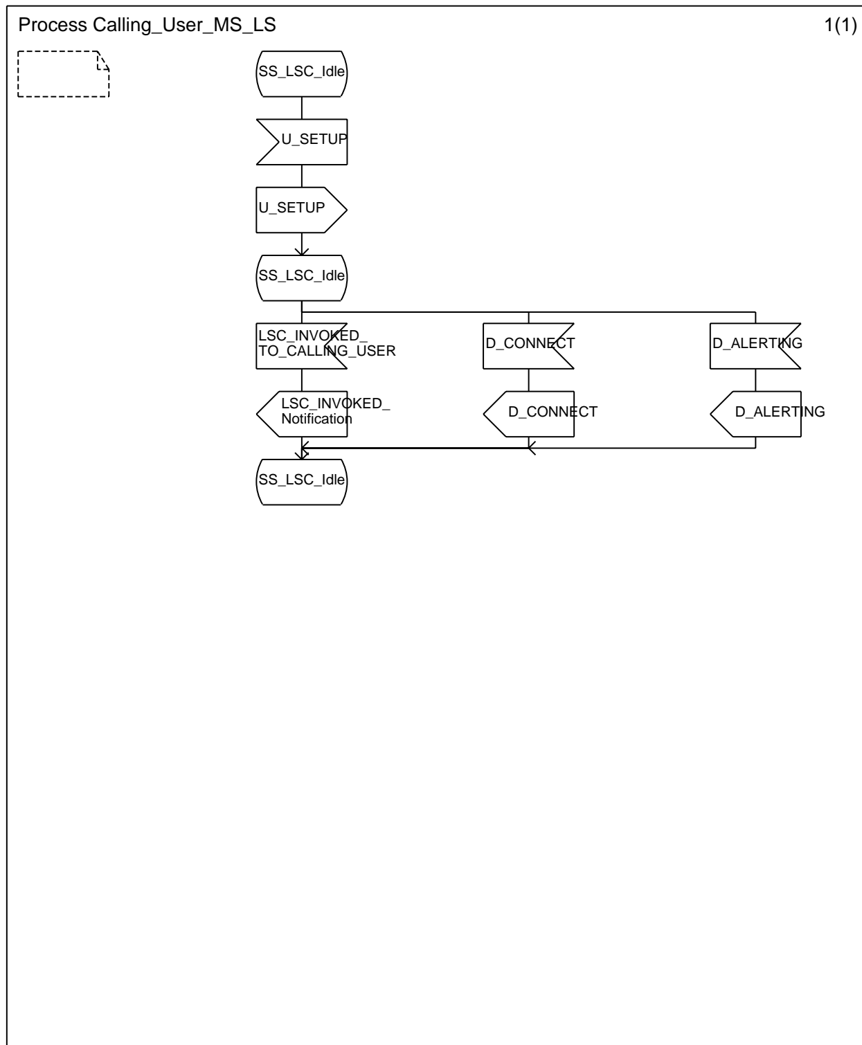
Figure A.1: Calling user A MS/LS SDL
