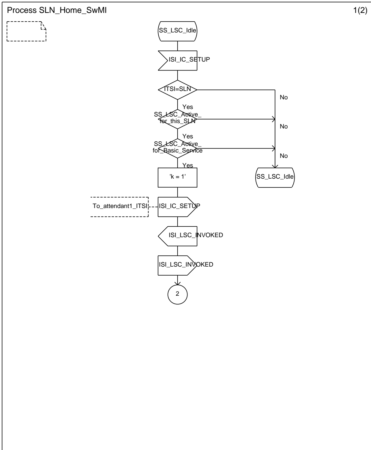
Figure A.5: Managed user home SwMI SDL (2/3)
