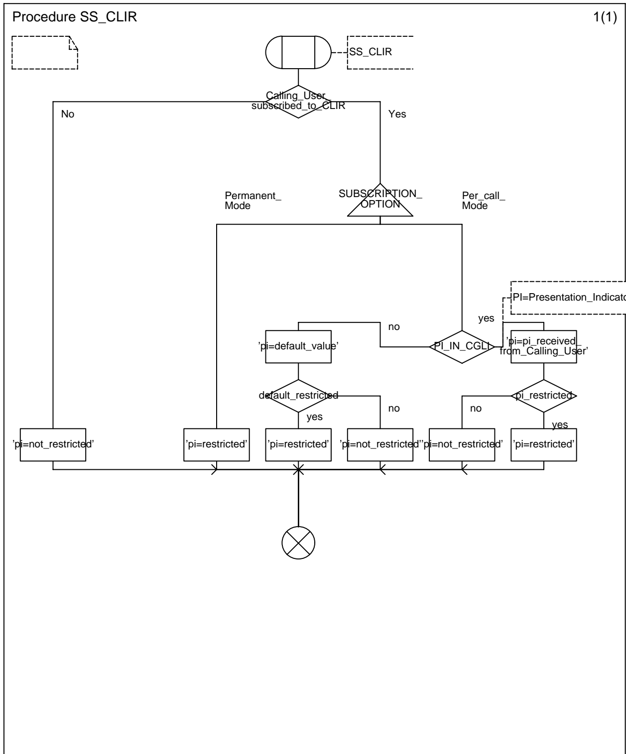
Figure B.2: SS-CLIR Procedure
