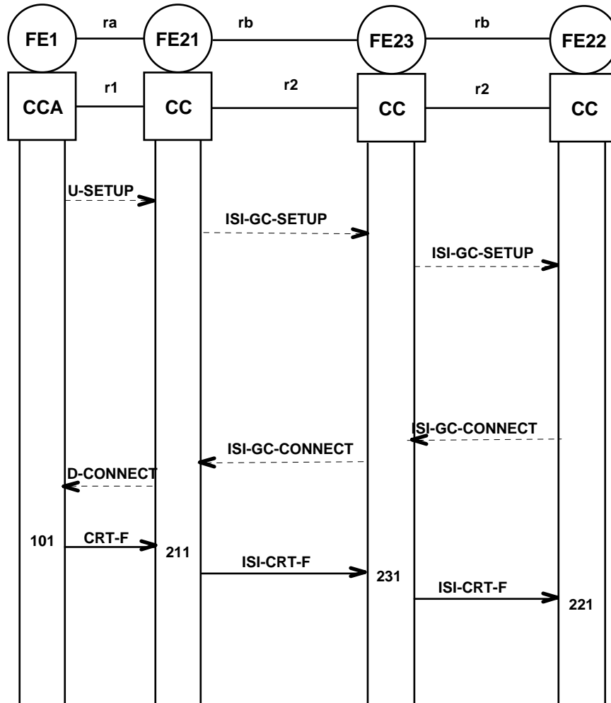
Figure 12: Information flow sequence for SS-CRT - normal operation, forward direction once group call is established.
