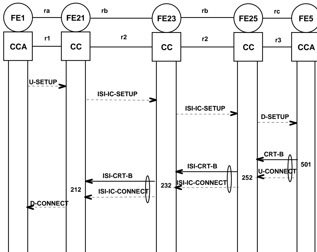
Figure 7: Information flow sequence for SS-CRT - normal operation, backward direction
