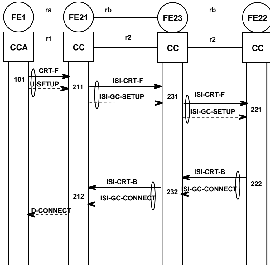
Figure 10: Information flow sequence for SS-CRT - normal operation, both directions, group call
