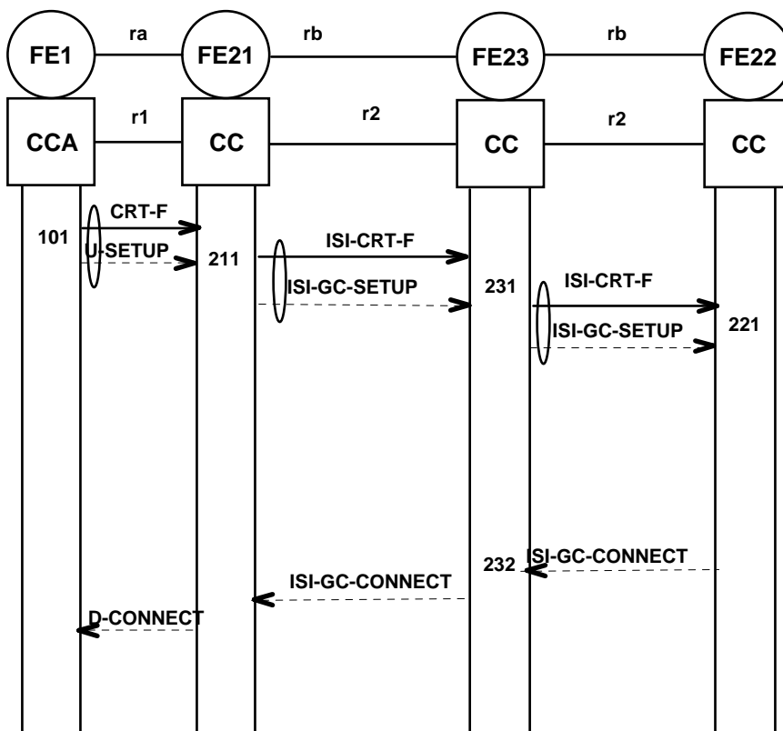
Figure 9: Information flow sequence for SS-CRT - normal operation, forward direction, group call
