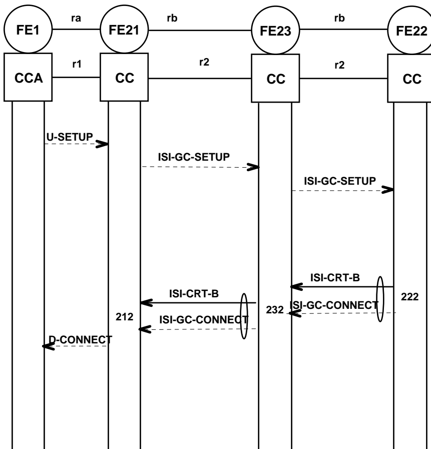
Figure 11: Information flow sequence for SS-CRT - normal operation, backward direction, group call
