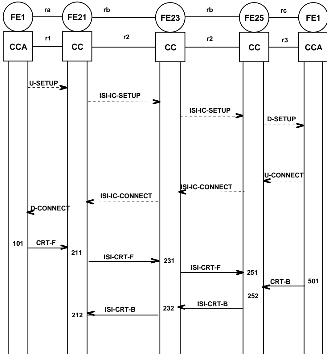
Figure 8: Information flow sequence for SS-CRT - normal operation, both directions
