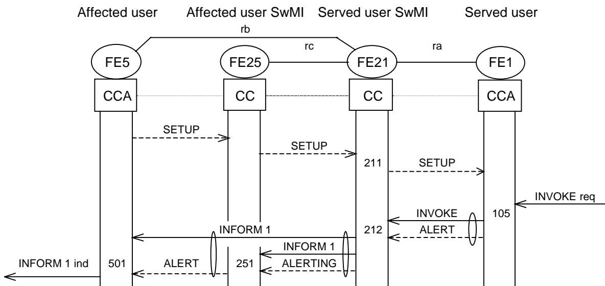
Figure 7: Successful invocation
