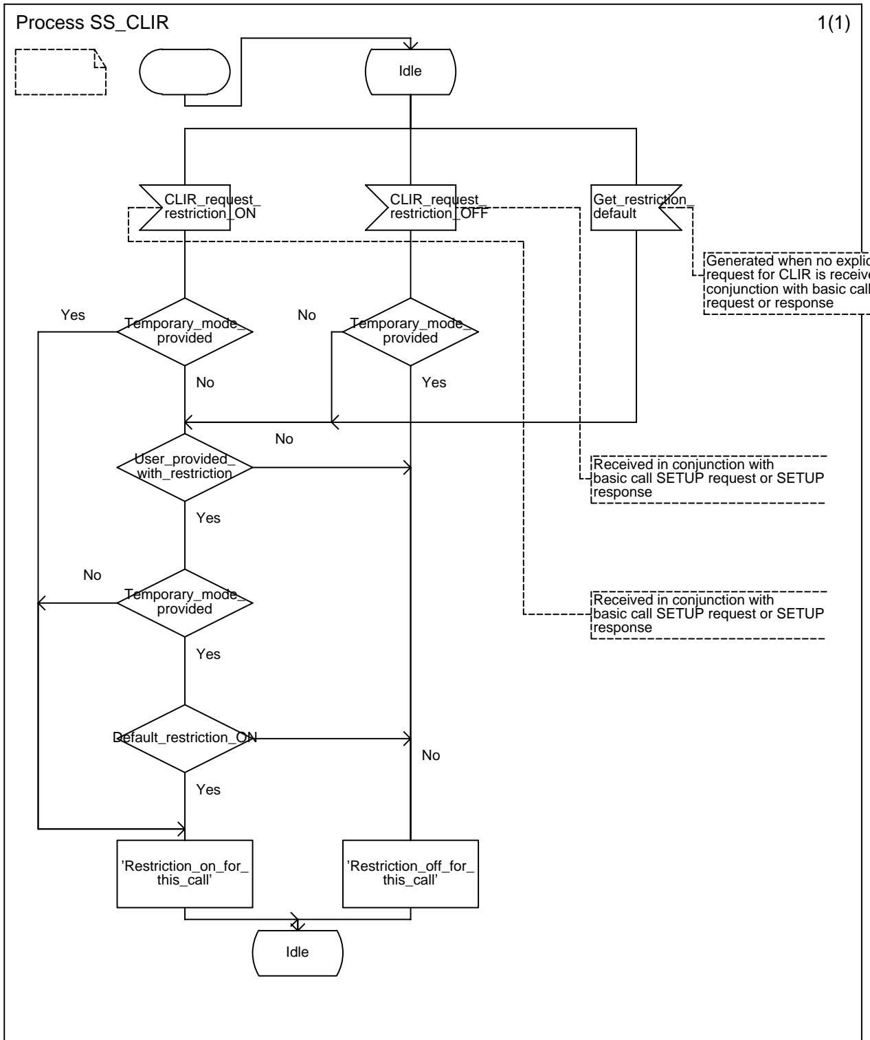
Figure 3: SS-CLIR, overall SDL
