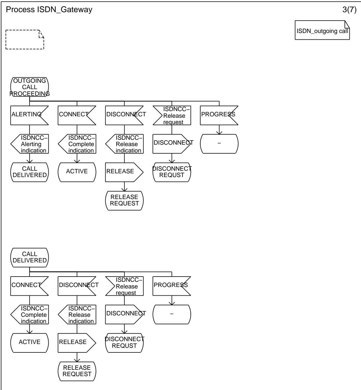
Figure A.3: SDL for ISDN gateway interface entity
