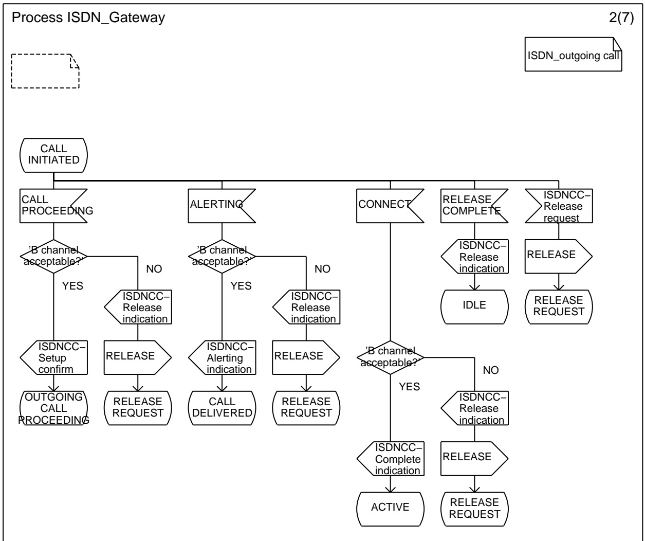
Figure A.2: SDL for ISDN gateway interface entity
