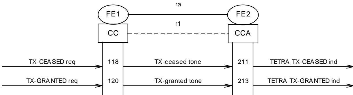
Figure 14: Information flow sequence - Request to transmit from a TETRA user 5.2.2.8 Call maintenance procedures - Request to interrupt
