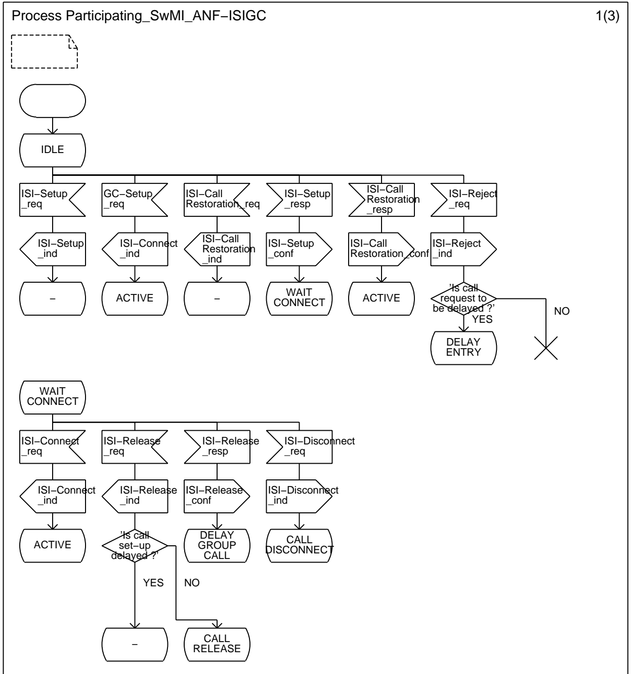
Figure A.9: SDL for participating SwMI ANF-ISIGC entity
