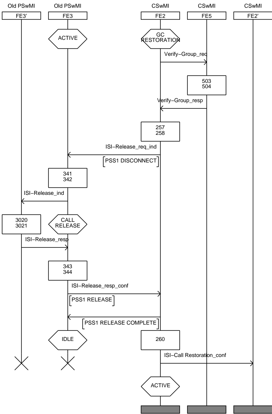
Figure 64: Information flow sequence - Group call restoration, case 3
