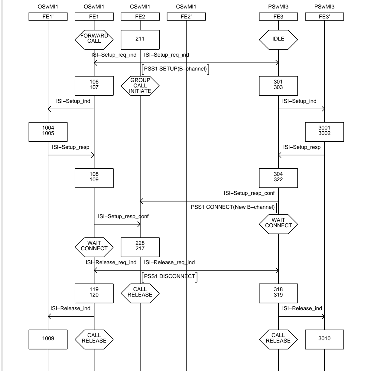
Figure 44: Information flow sequence - new B-channel not accepted (sheet 1 of 2)
