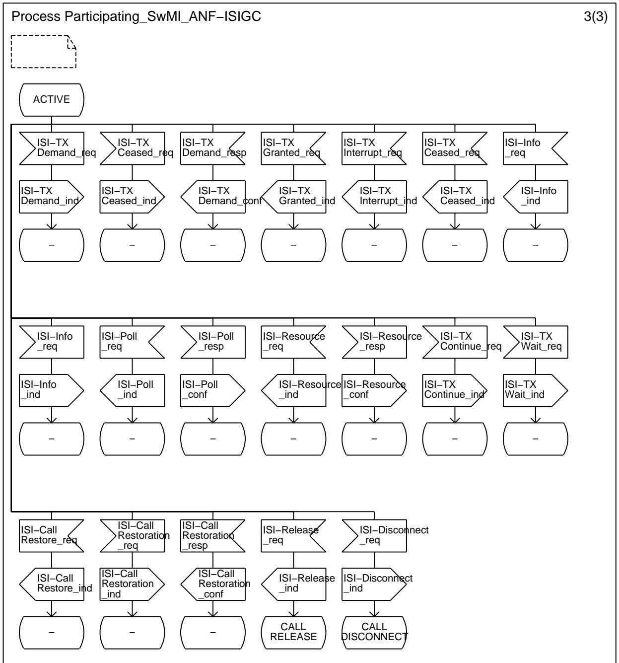
Figure A.11: SDL for participating SwMI ANF-ISIGC entity
