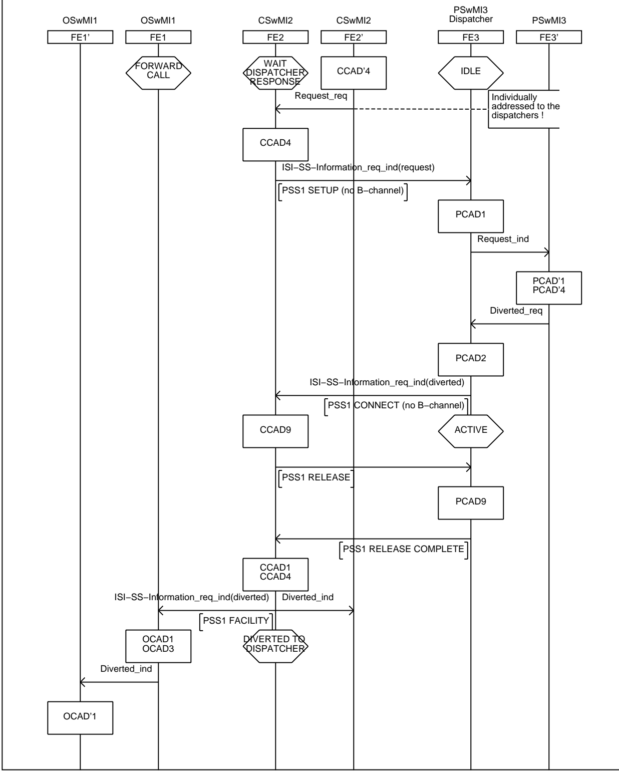
Figure B.10: Information flow sequence - On-demand call set-up (sheet 2 of 2)
