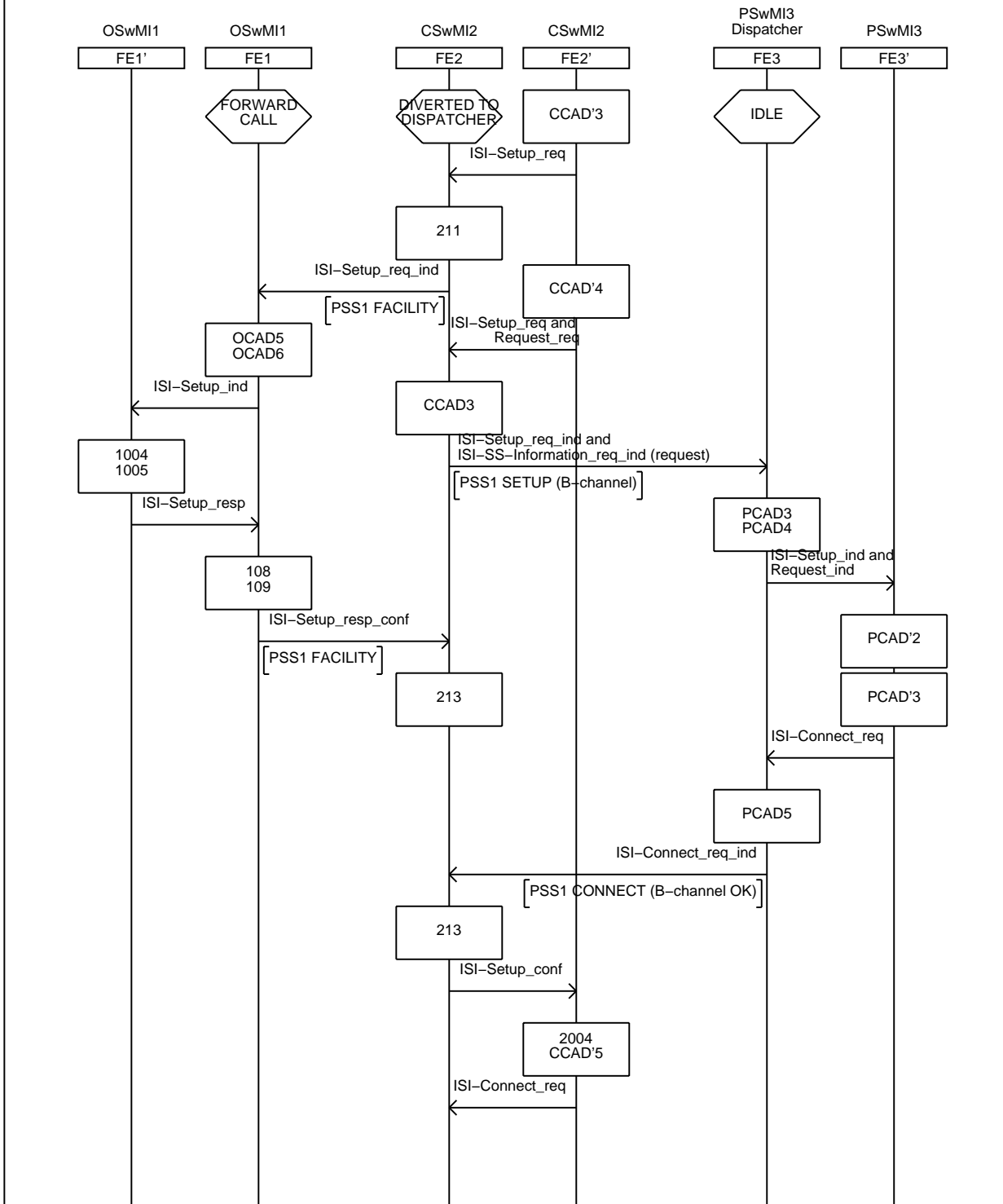
Figure B.2: Information flow sequence - Direct call set-up to dispatcher (sheet 2 of 5)
