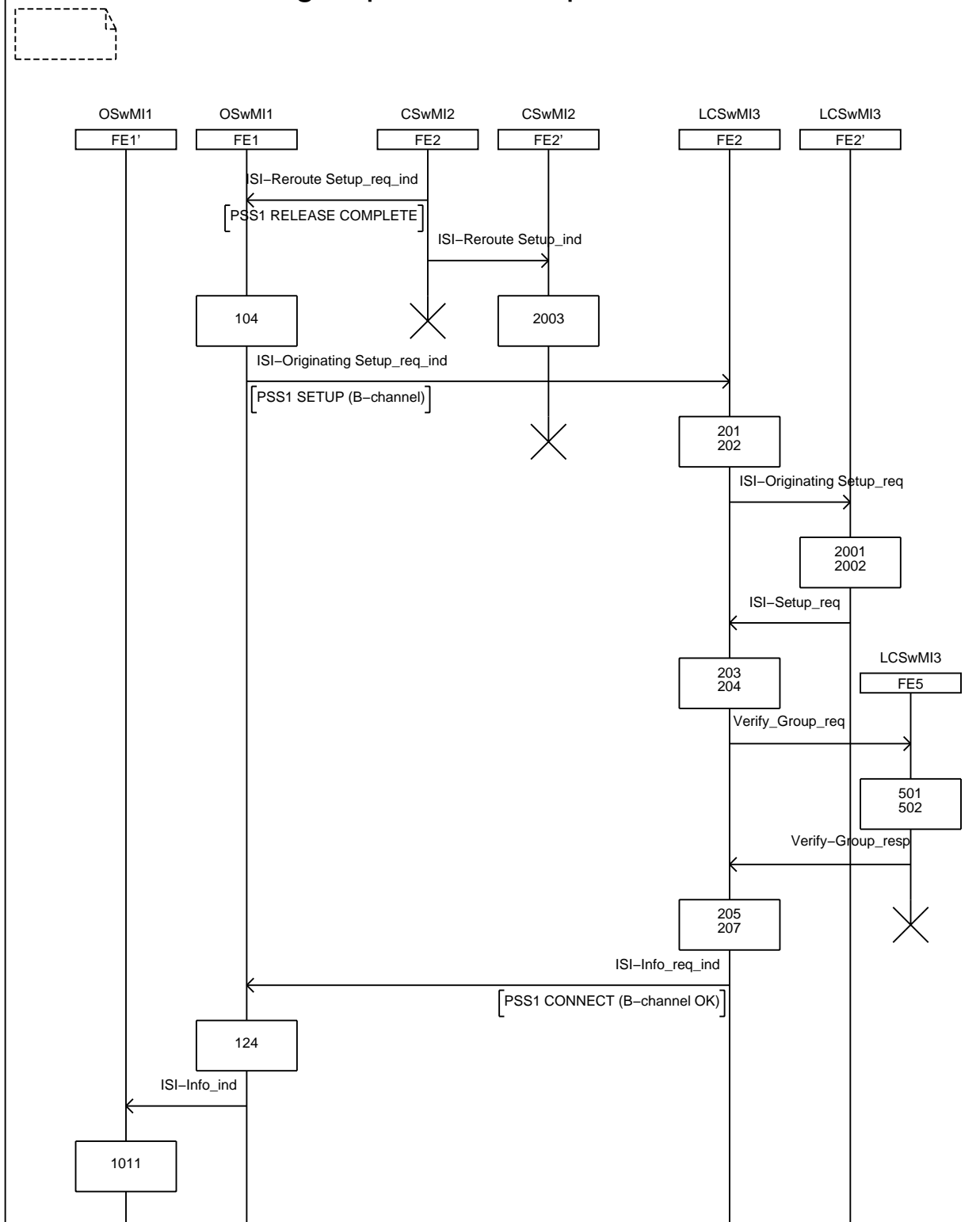
Figure 28: Information flow sequence - successful group call set-up, case 4 (sheet 2 of 4)
