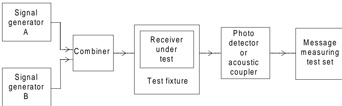
Figure 21: Measurement arrangement
