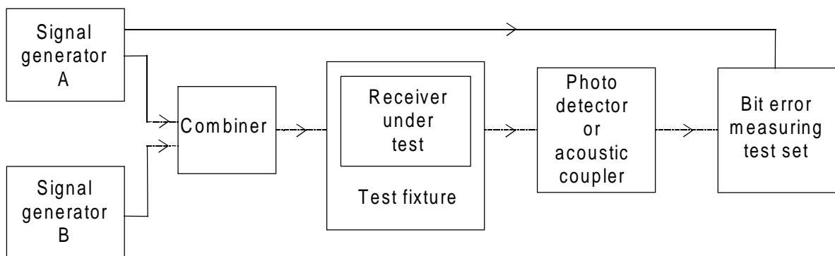
Figure 22: Measurement arrangement
