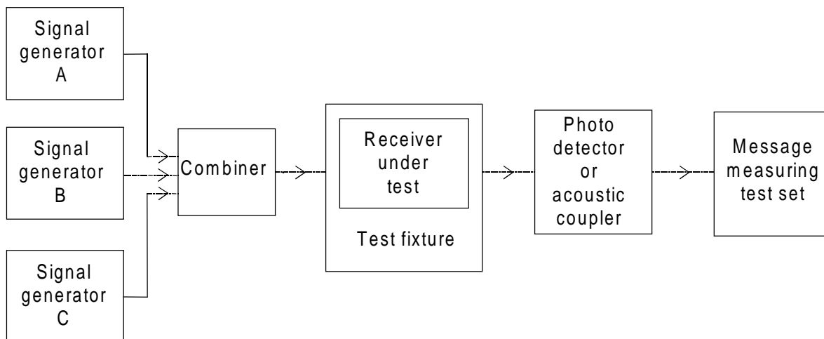
Figure 25: Measurement arrangement
