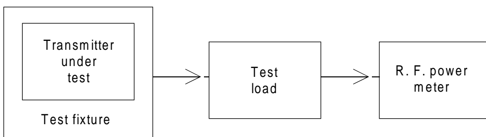
Figure 5: Measurement arrangement
