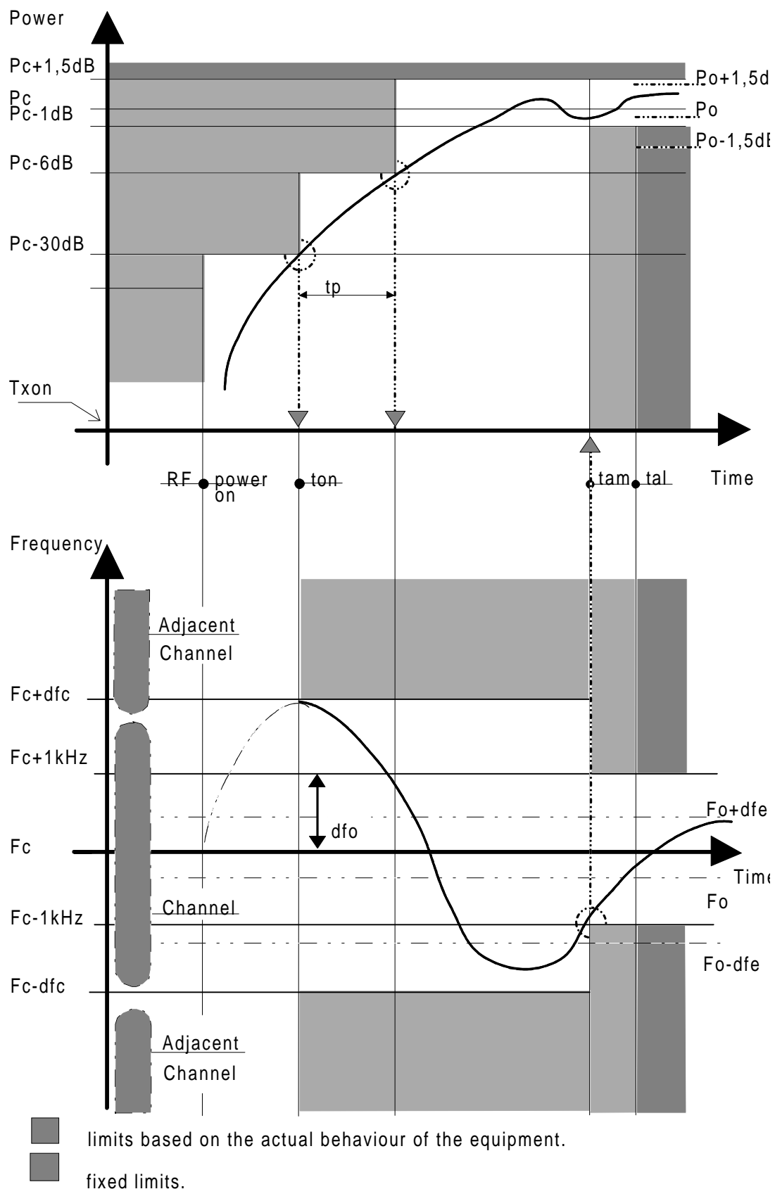
Figure 10: Transmitter attack time according to 8.5.1 b) and transient behaviour during switch-on (Case where the attack time is given by the behaviour of the frequency)
