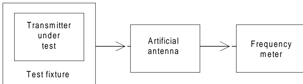
Figure 2: Measurement arrangement
