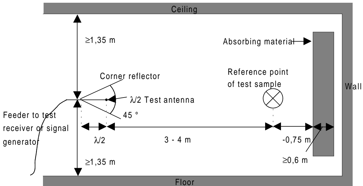
Figure A.5: Indoor test site arrangement (shown for horizontal polarisation)
