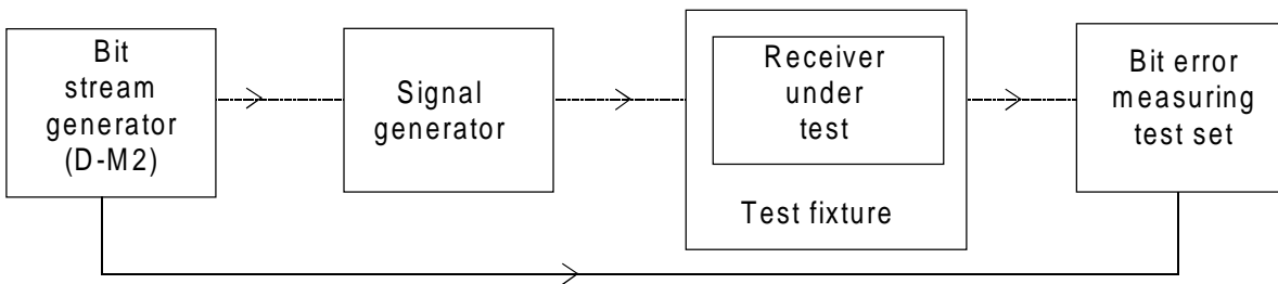
Figure 18: Measurement arrangement
