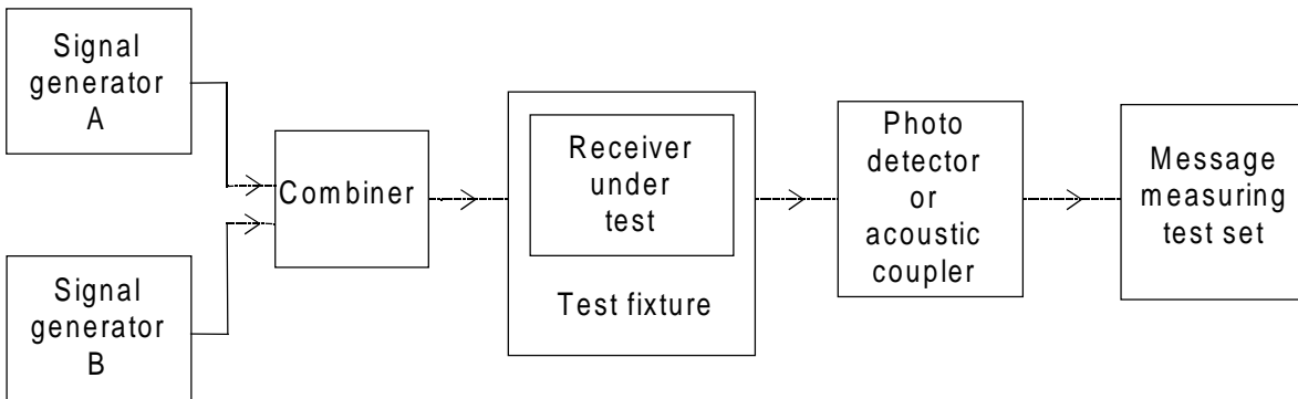
Figure 23: Measurement arrangement
