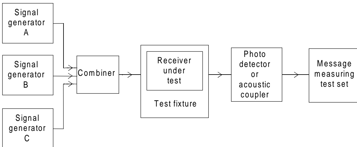
Figure 26: Measurement arrangement
