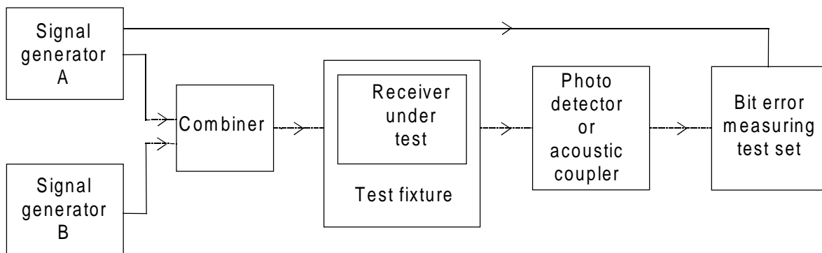
Figure 20: Measurement arrangement
