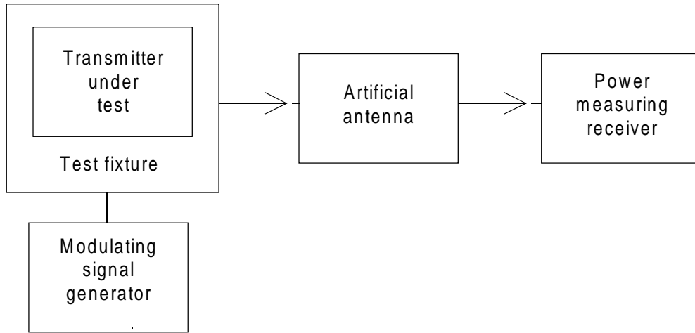
Figure 6: Measurement arrangement
