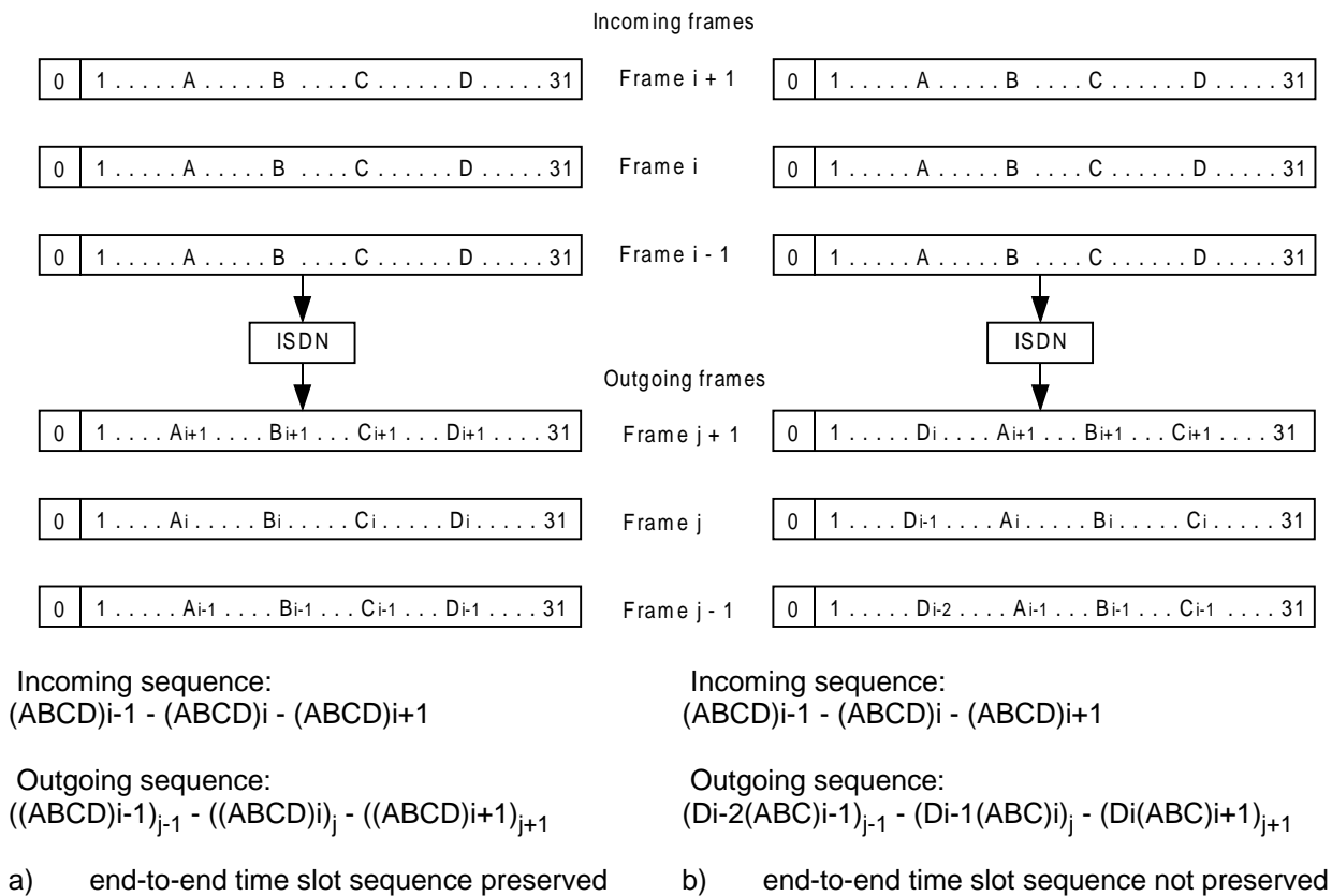
Figure A.2: Inter-frame TSSI
