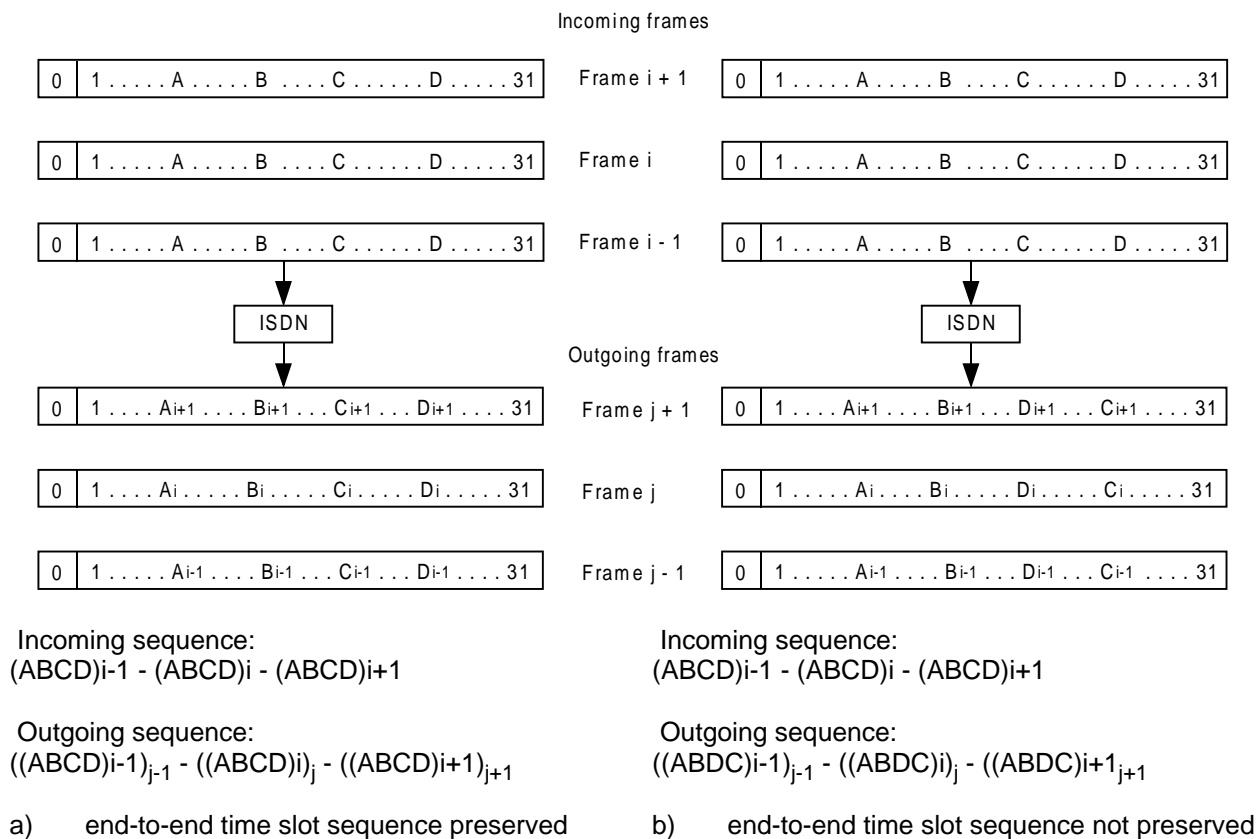
Figure A.3: Intra-frame TSSI
