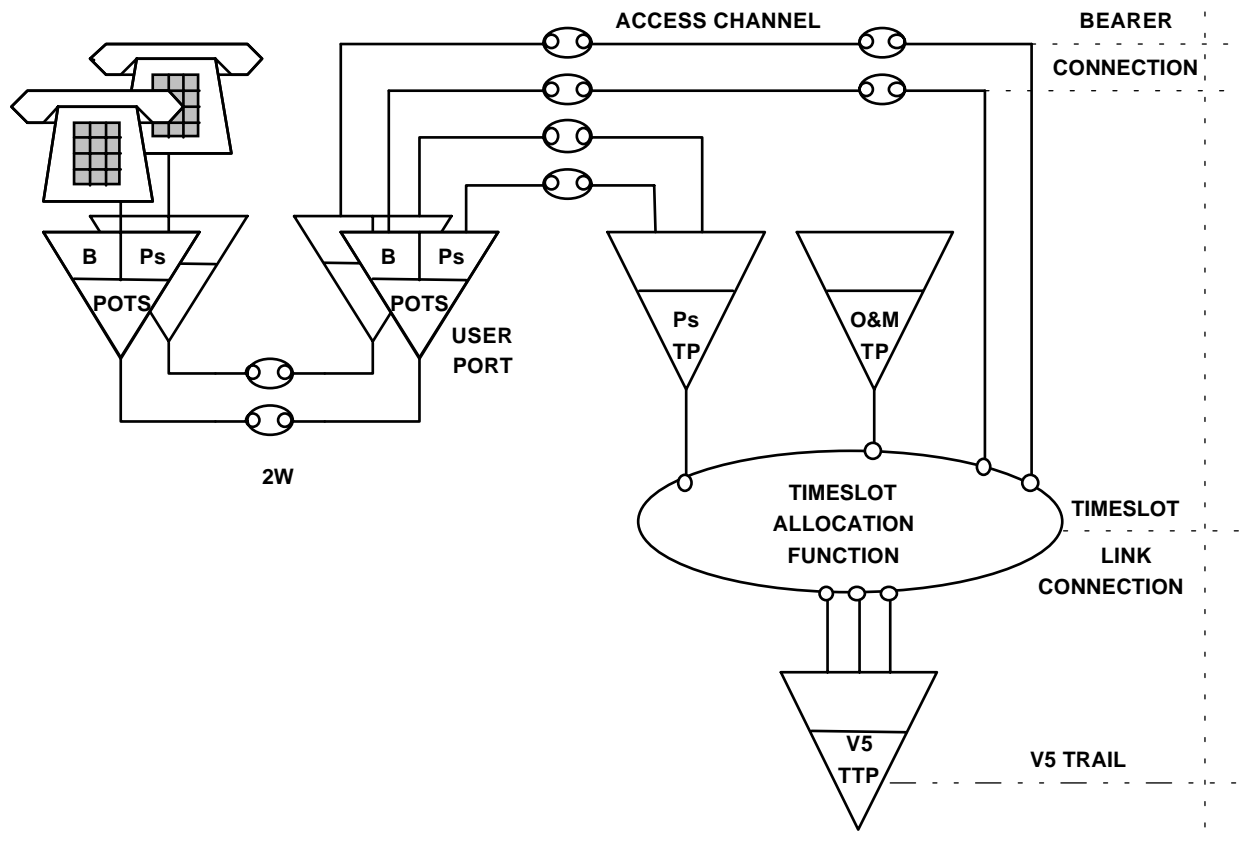
Figure D.1: Access network side V5 functional architecture for PSTN
