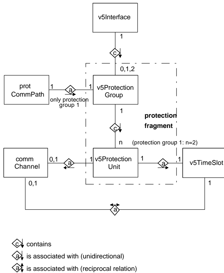
Figure 4: Entity relationship diagram - protection fragment
