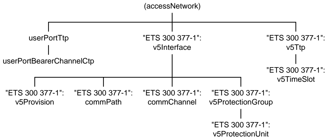
Figure 6: Naming hierarchy
