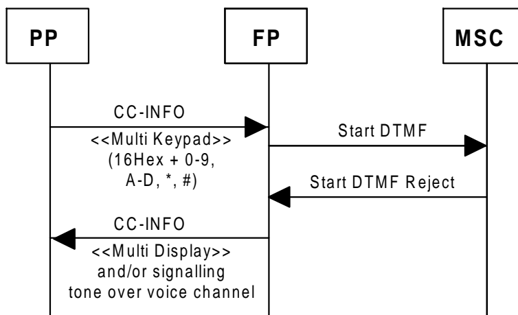
Figure 34: Rejection of DTMF start message
