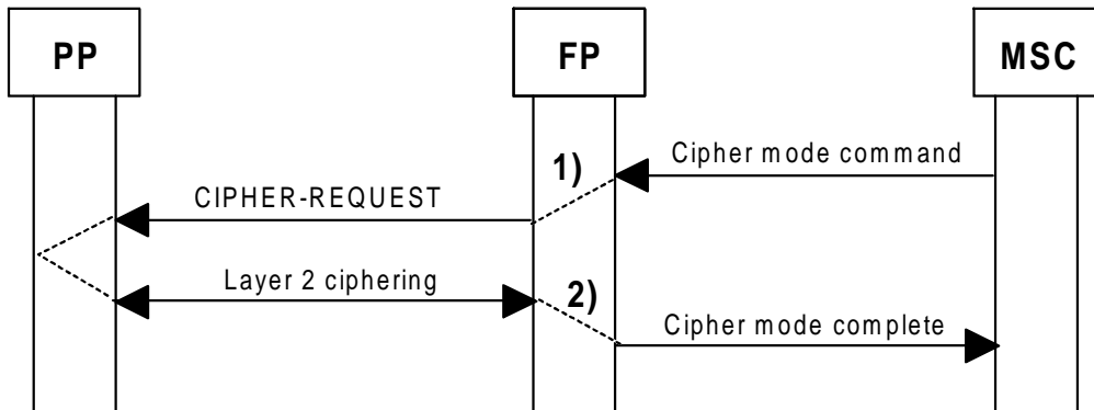
Figure 23: Cipherng procedure
