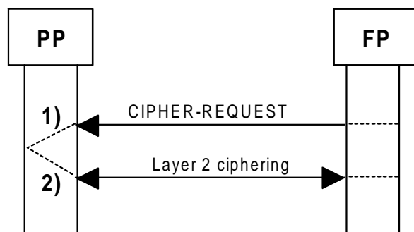
Figure 42: Cipherng procedure
