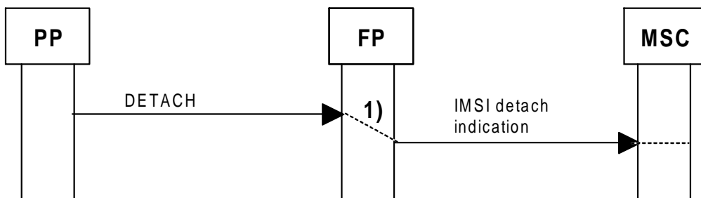
Figure 20: Detach procedure
