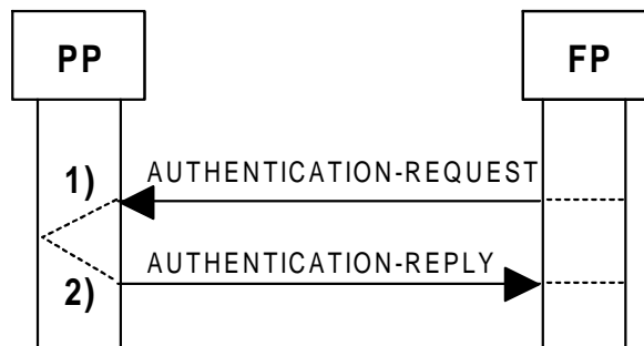
Figure 37: Authentication procedure
