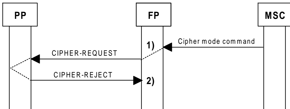
Figure 24: Ciphering procedure - rejection
