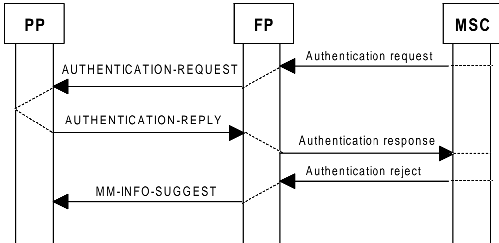
Figure 16: Authentication procedure
