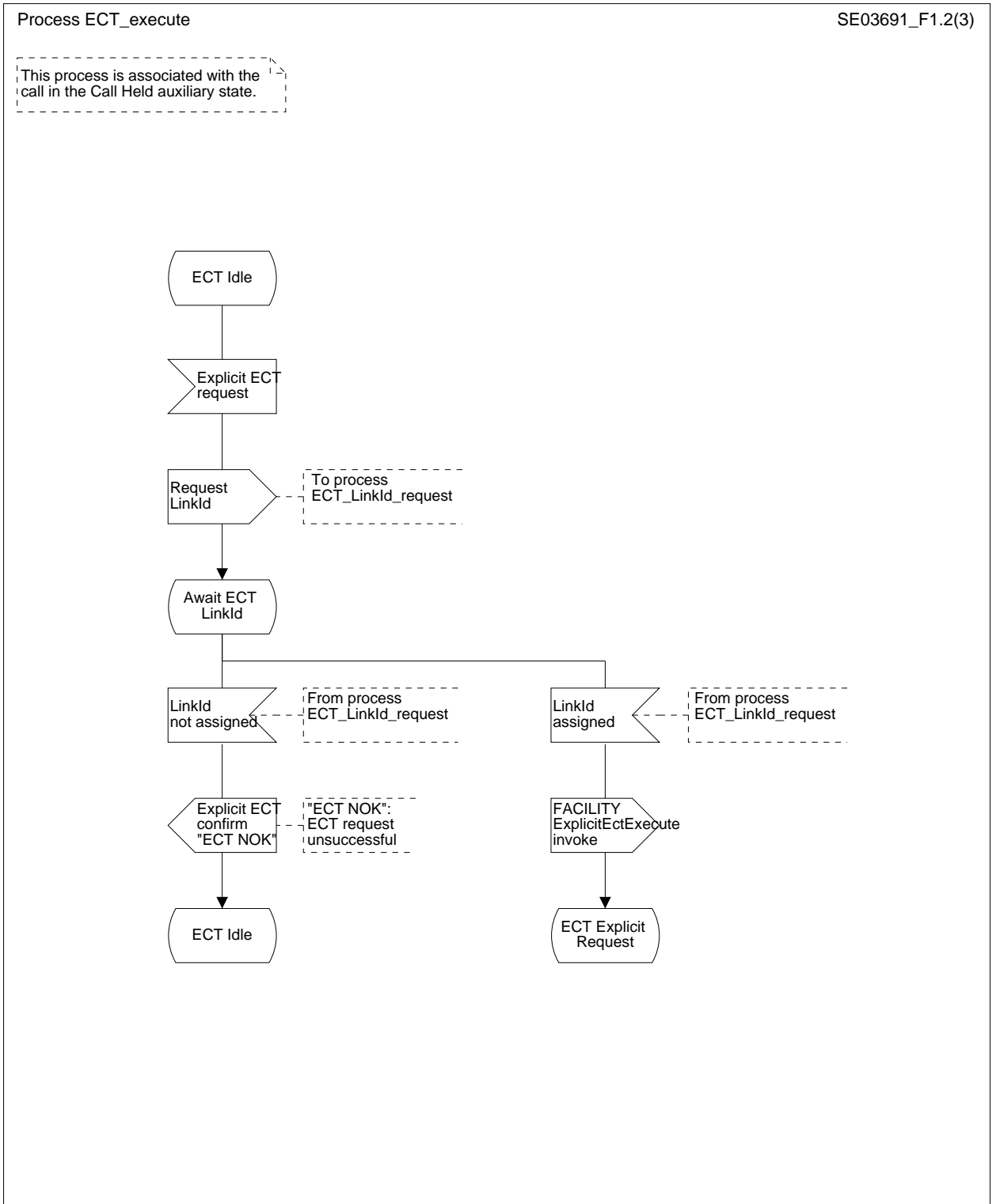
Figure 1 (sheet 2 of 3): ECT user A, ECT execute
