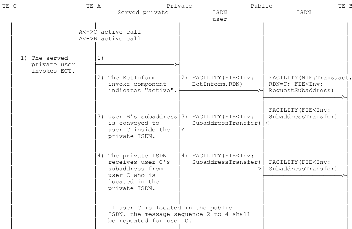
Figure A.9: Served user in a private ISDN
