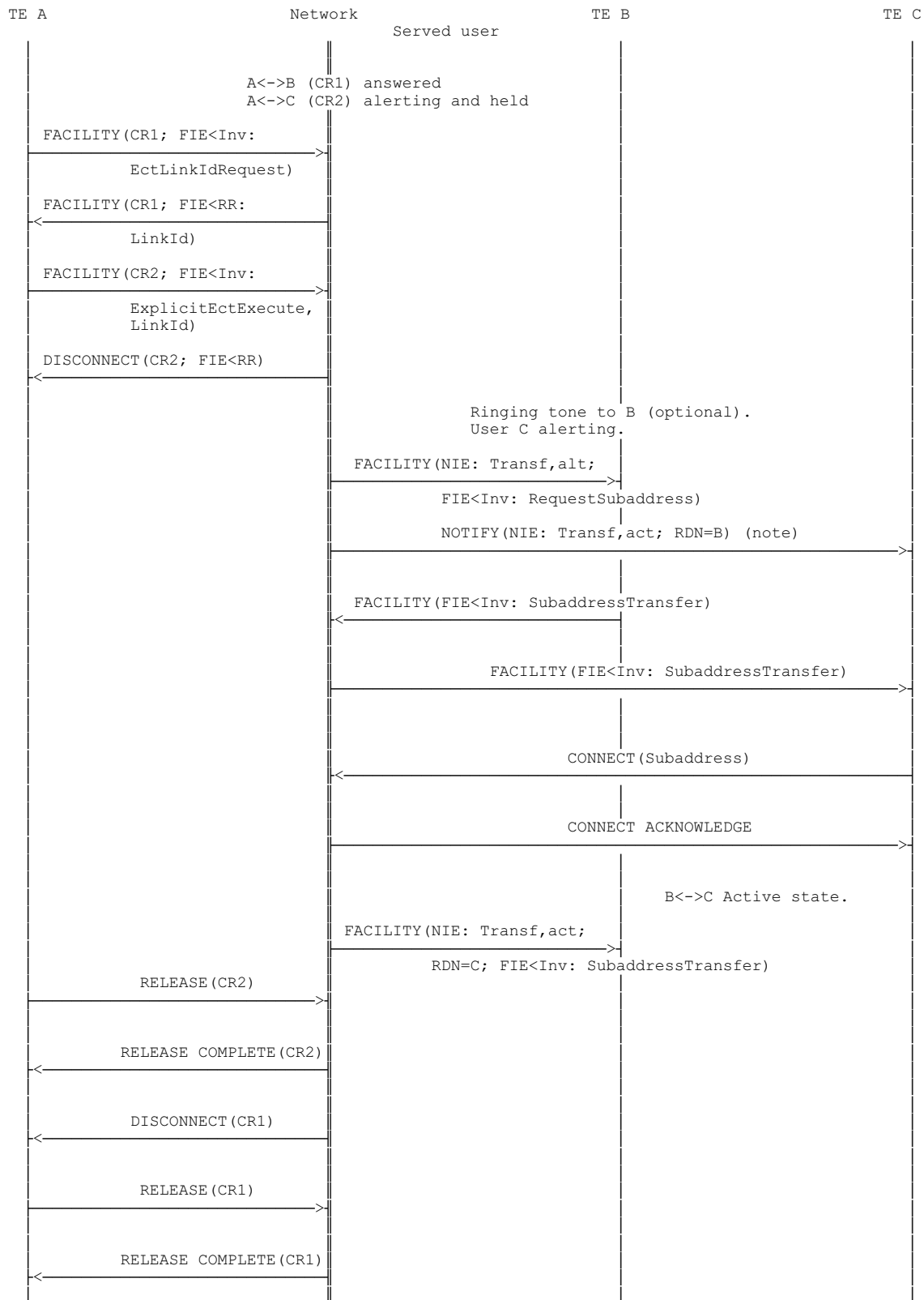
Figure A.8: ECT explicit invocation - Transfer while alerting
