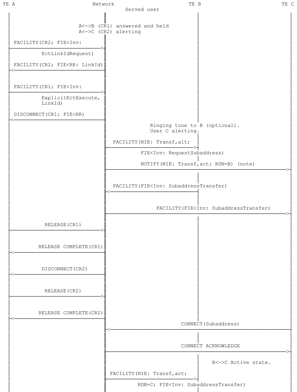
Figure A.7: ECT explicit invocation - Transfer while alerting
