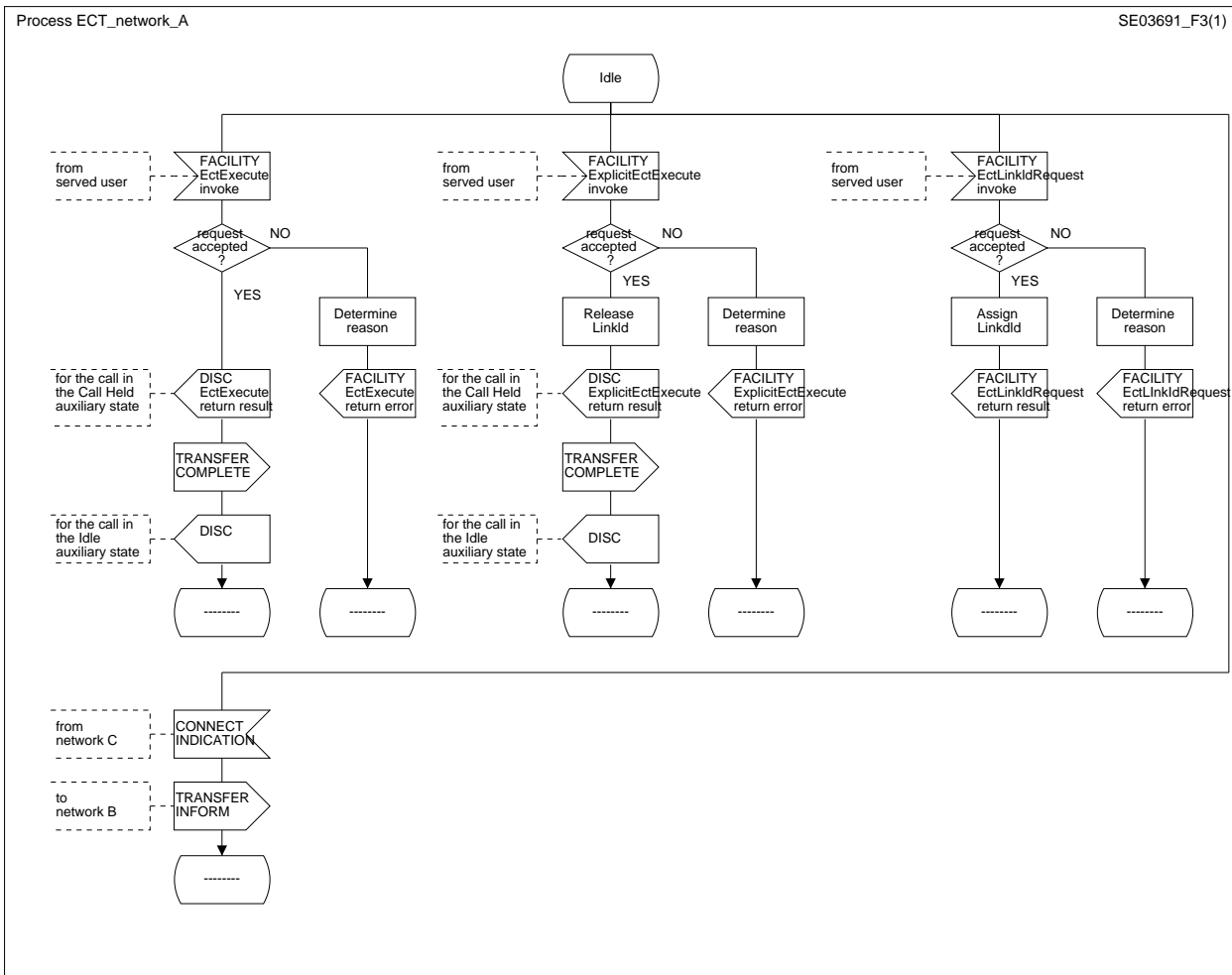
Figure 3: ECT network A
