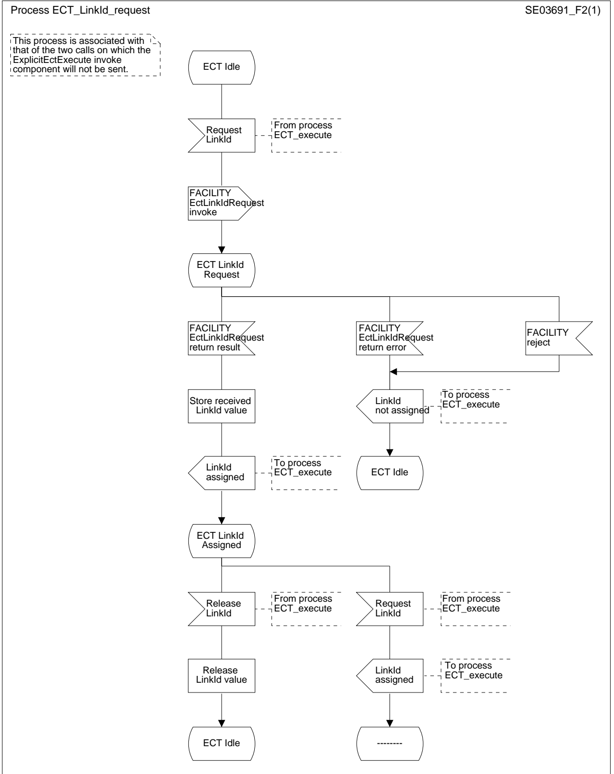
Figure 2: ECT user A, ECT LinkId request
