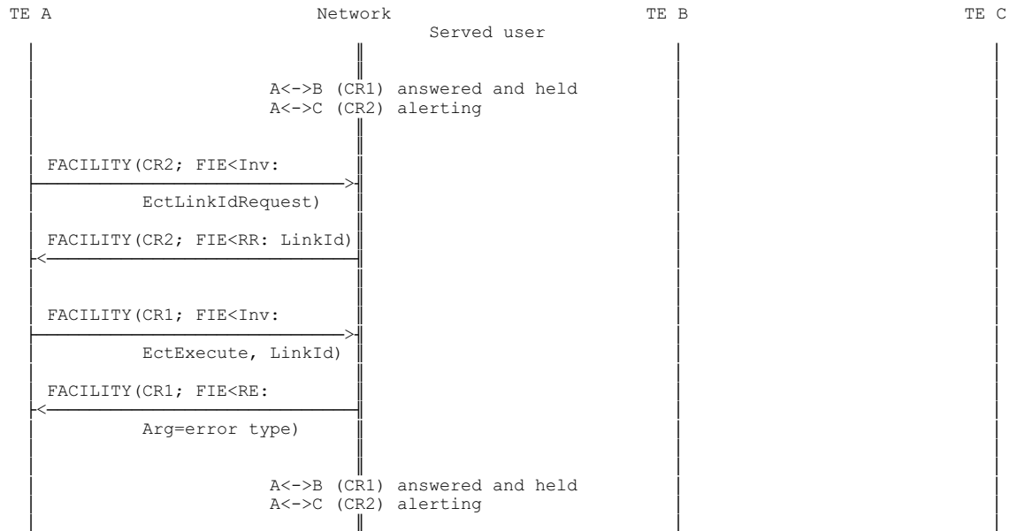
Figure A.4: ECT explicit invocation - EctExecute fails
