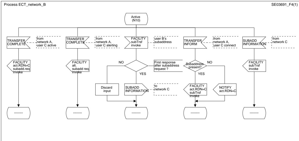
Figure 4: ECT network B
