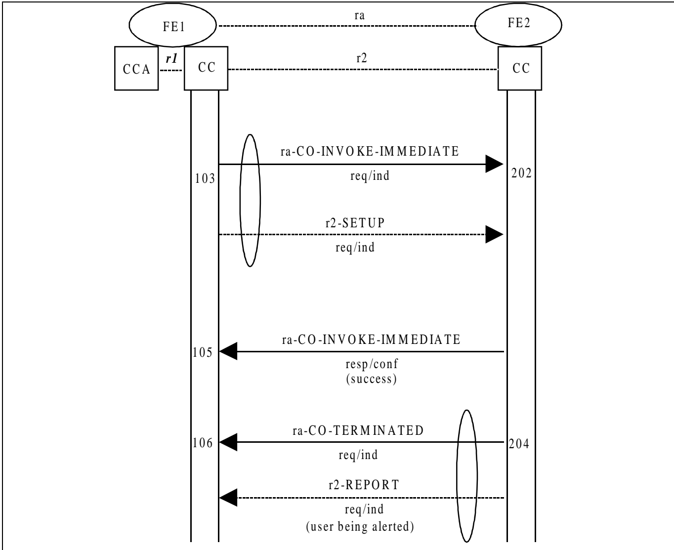
Figure 4 - Information flow sequence - normal operation of SS-CO without path retention and with the called user being alerted after resources become available
