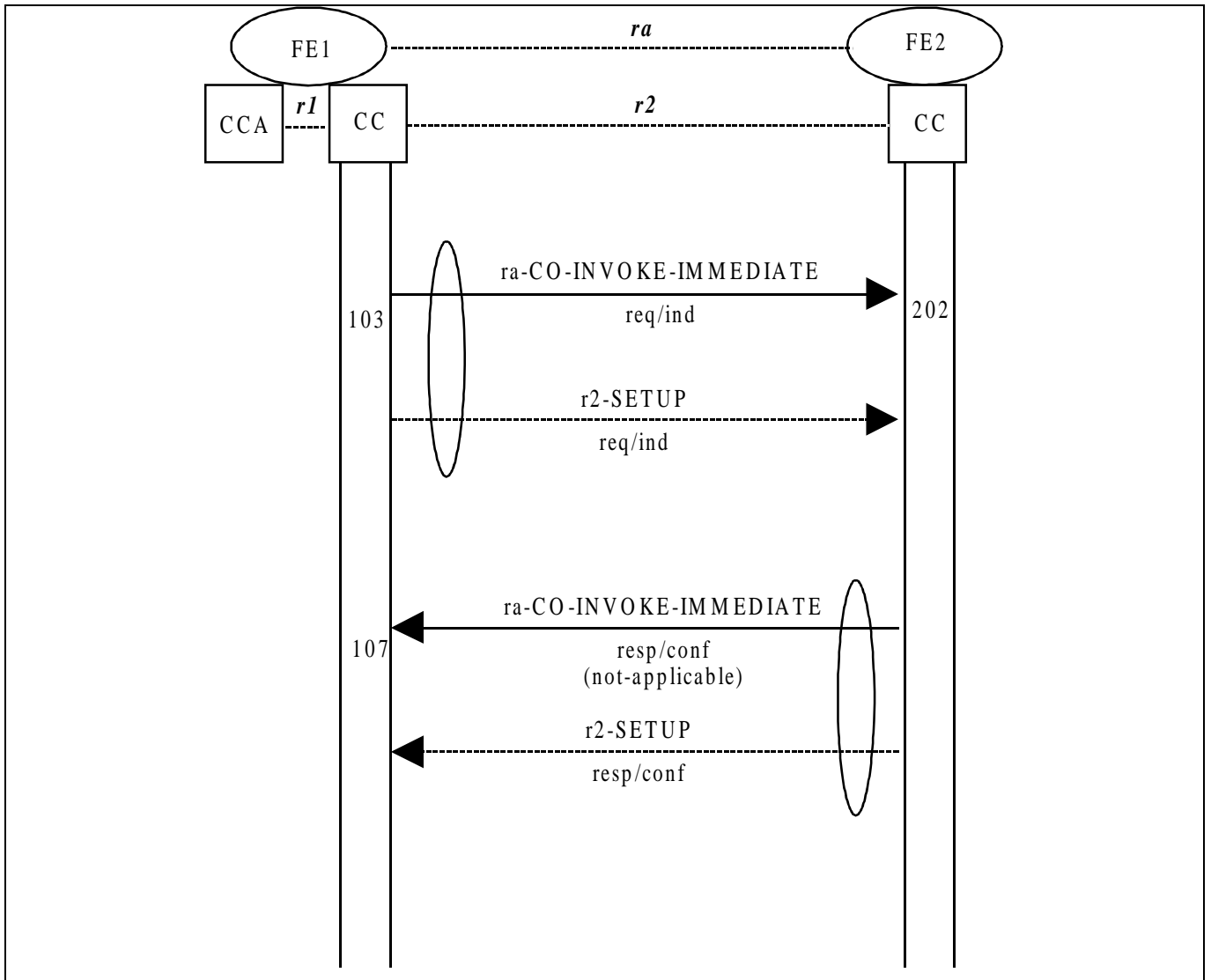
Figure 9 - Information flow sequence - failure operation of SS-CO without path retention (called user is not busy and accepts the call immediately)
