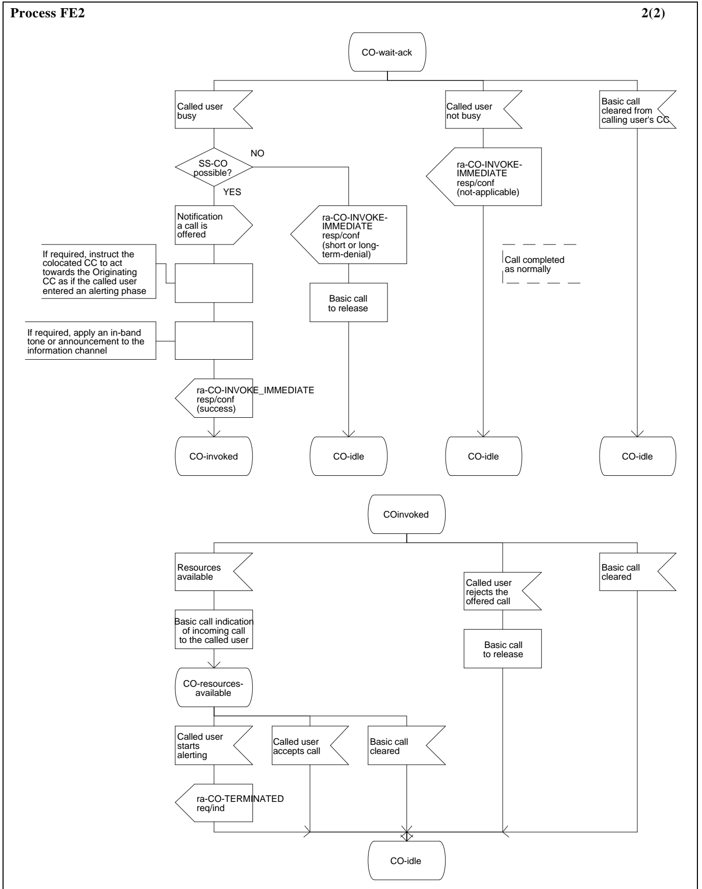
Figure 12 (sheet 2 of 2) - SDL for Functional Entity FE2
