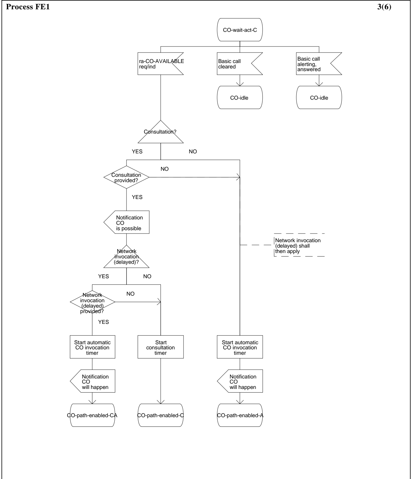
Figure 11 (sheet 3 of 6) - SDL for Functional Entity FE1
