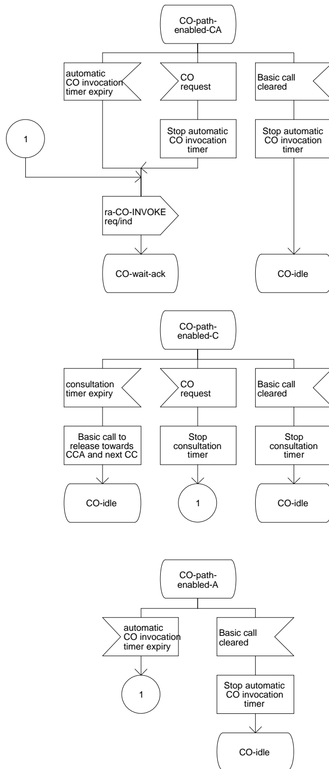
Figure 11 (sheet 4 of 6) - SDL for Functional Entity FE1
