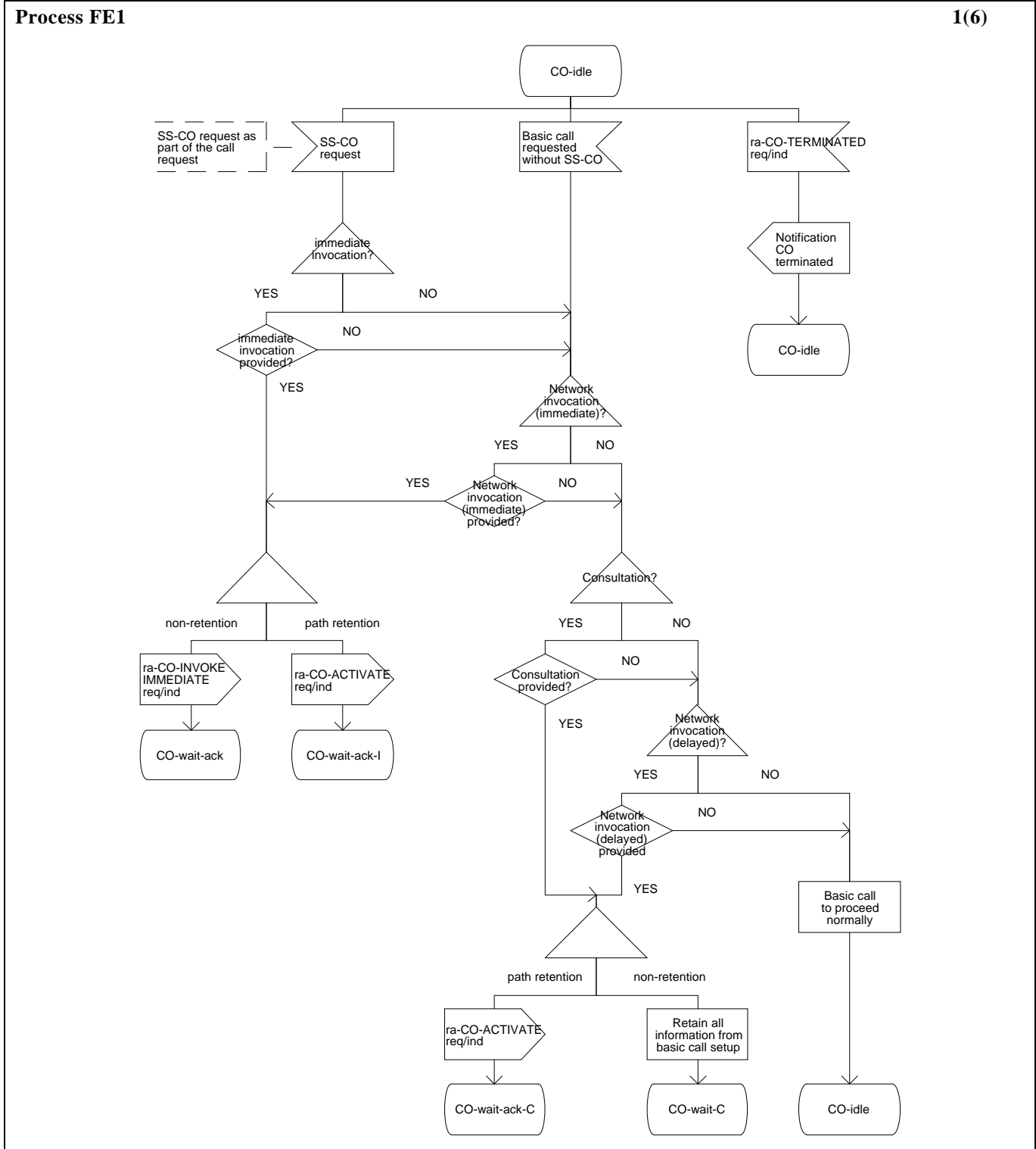
Figure 11 (sheet 1 of 6) - SDL for Functional Entity FE1
