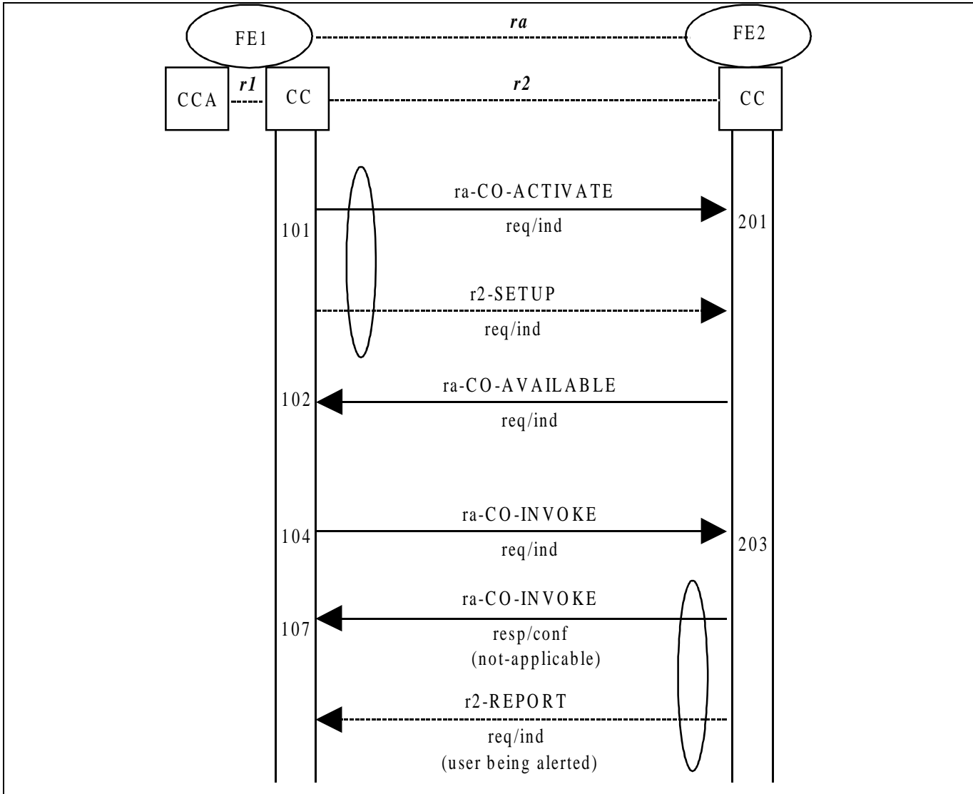
Figure 10 - Information flow sequence - failure operation of SS-CO with path retention (called user not busy when receiving the SS-CO request)
