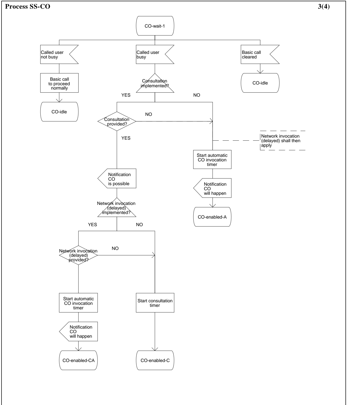
Figure 1 (sheet 3 of 4) - SS-CO, overall SDL
