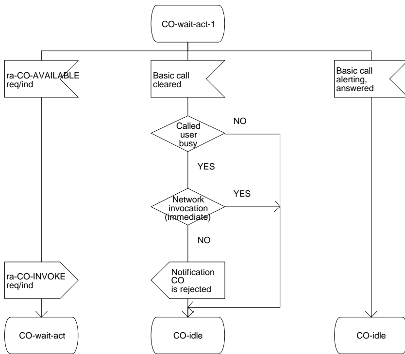
Figure 11 (sheet 2 of 6) - SDL for Functional Entity FE1
