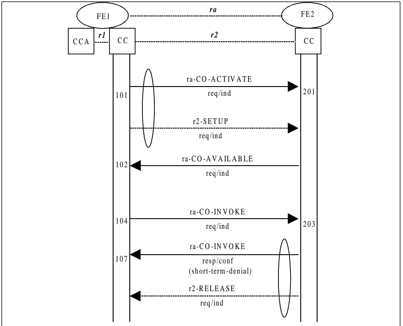
Figure 7 - Information flow sequence - failure operation of SS-CO with path retention (for instance, because the called user is unable to accept a further offered call)
