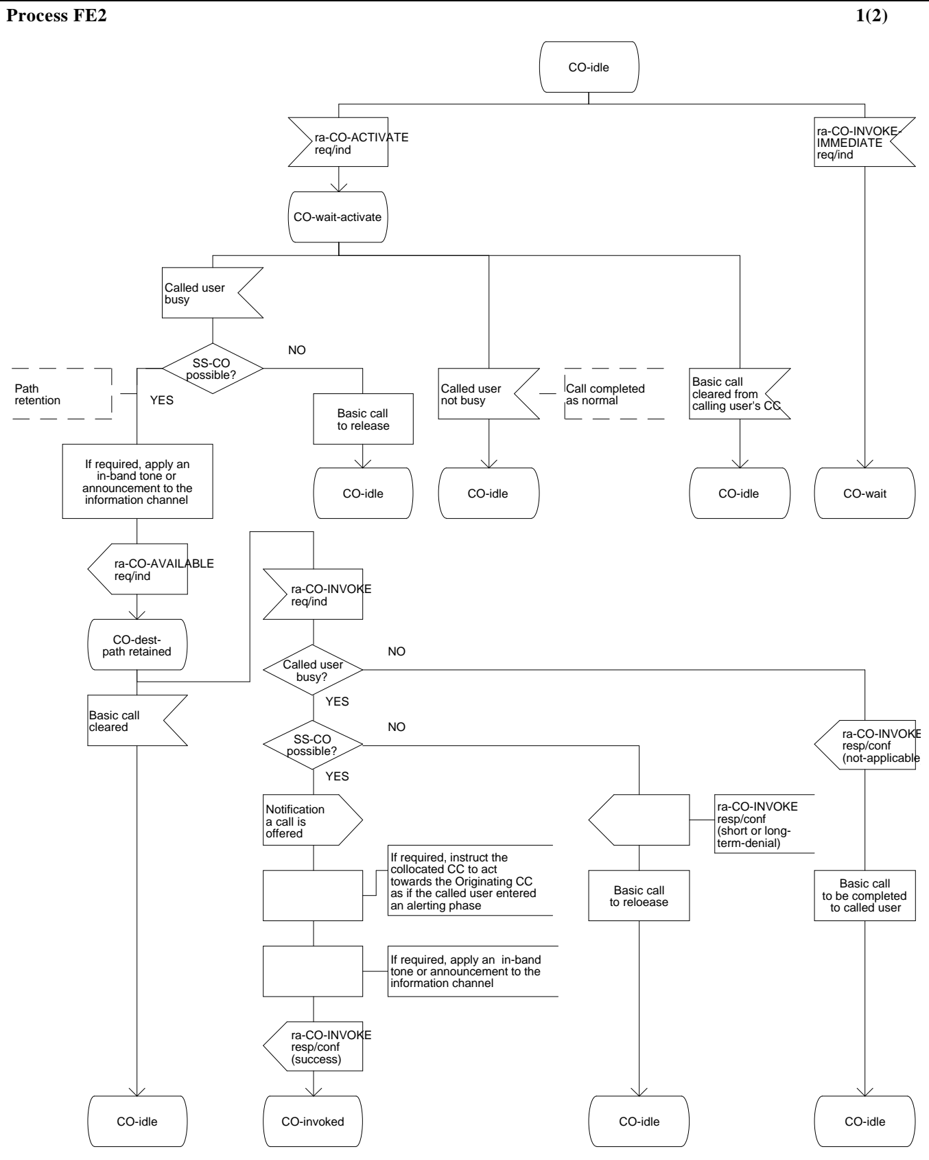
Figure 12 (sheet 1 of 2) - SDL for Functional Entity FE2
