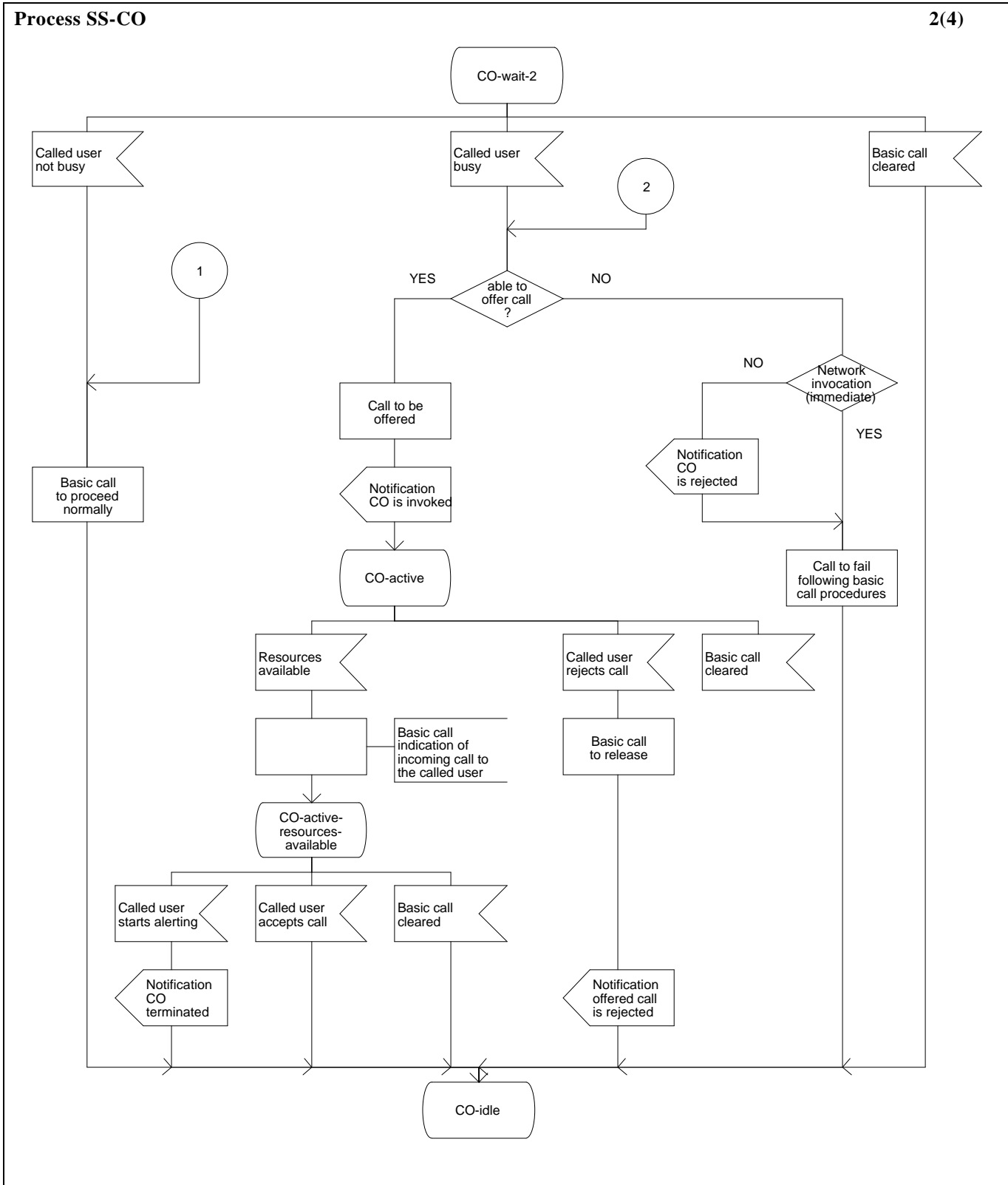
Figure 1 (sheet 2 of 4) - SS-CO, overall SDL
