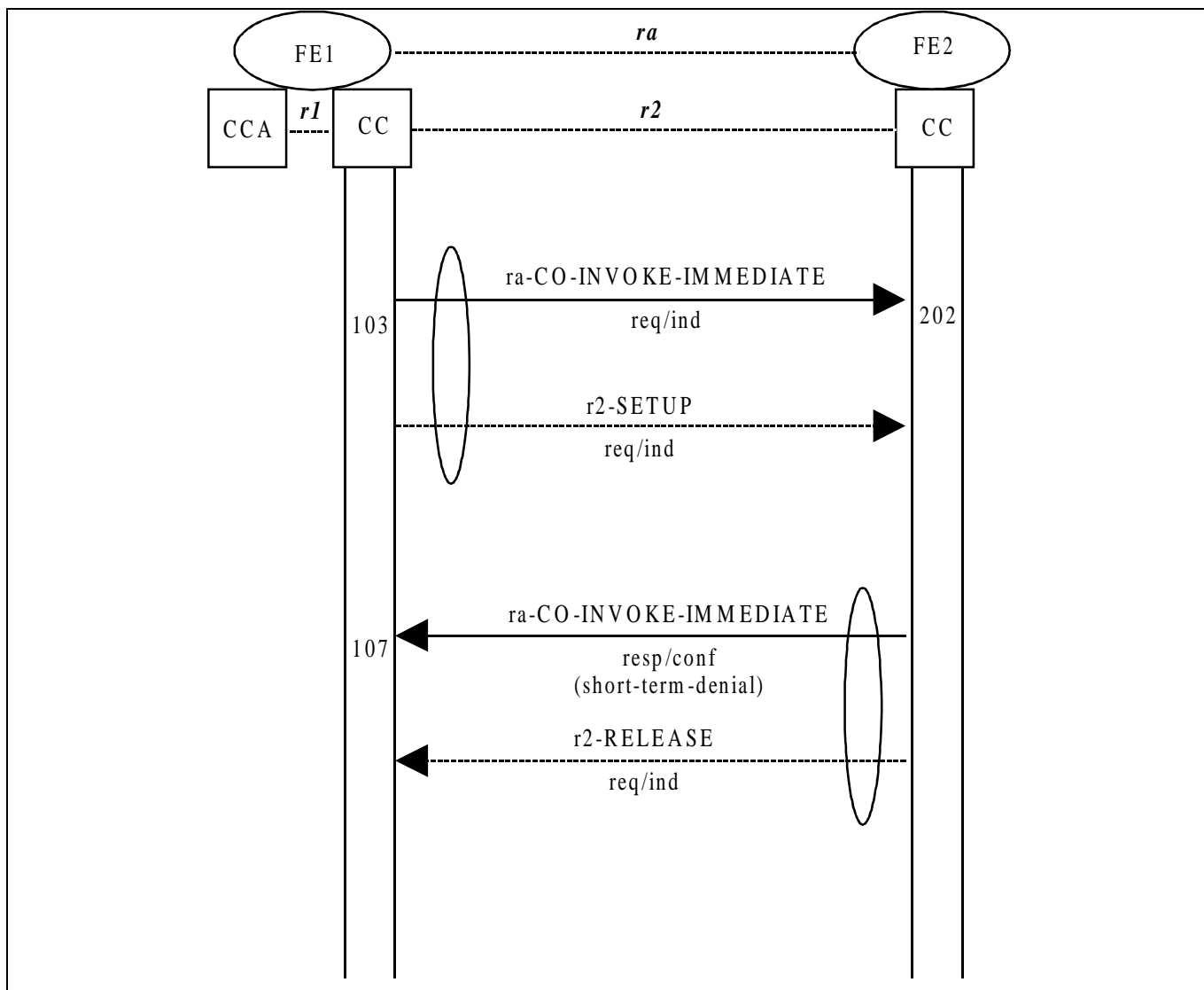
Figure 6 - Information flow sequence - failure operation of SS-CO without path retention (for instance, because the called user is unable to accept a further offered call)
