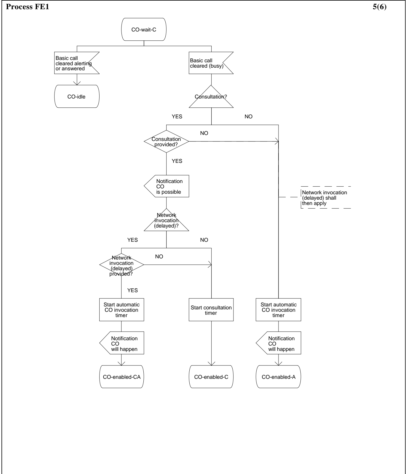
Figure 11 (sheet 5 of 6) - SDL for Functional Entity FE1
