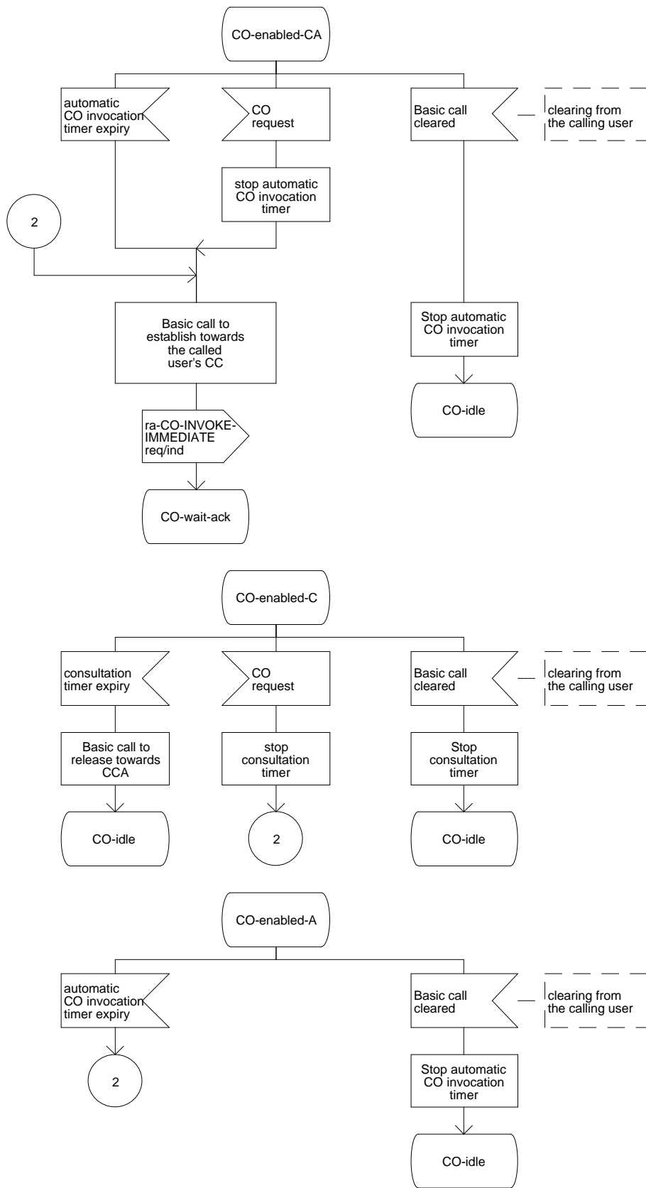
Figure 11 (sheet 6 of 6) - SDL for Functional Entity FE1
