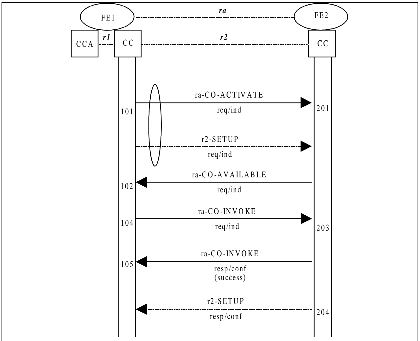
Figure 5 - Information flow sequence - normal operation of SS-CO with path retention and with acceptance of the call by the called user
