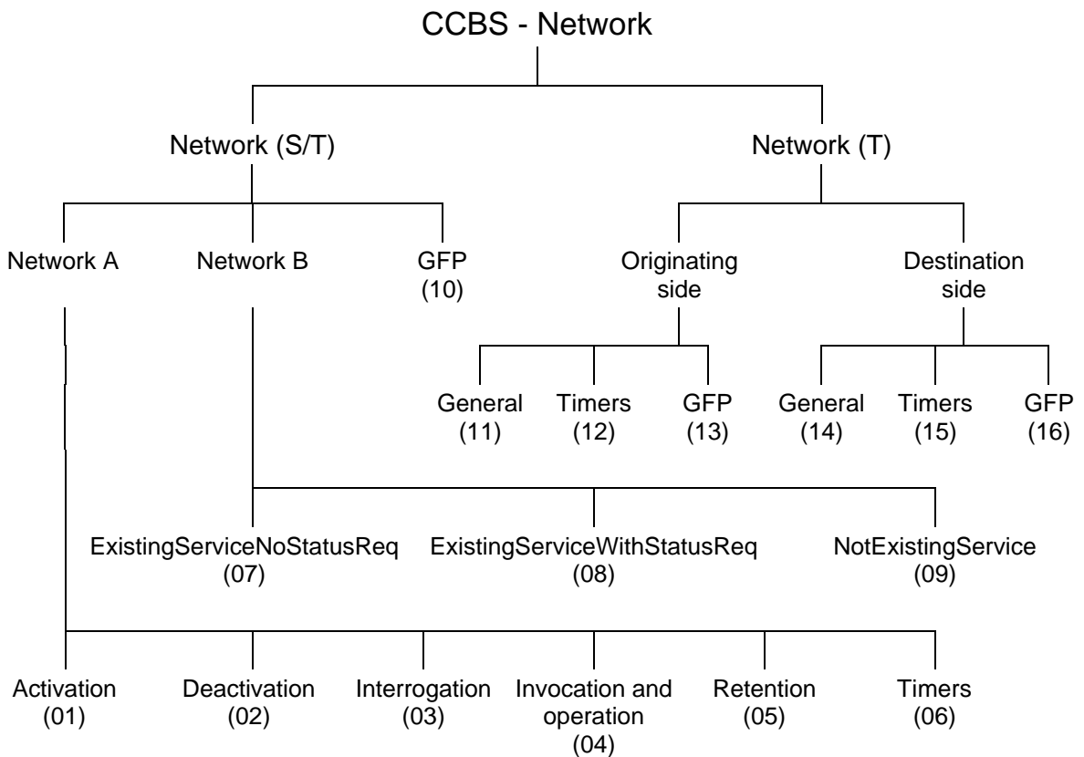
Figure 1: Test suite structure
