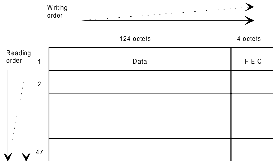
Figure 10: Structure and format of the long interleaver matrix
