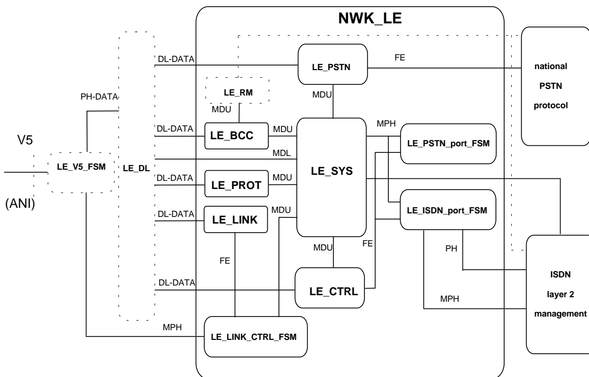
Figure 2: Network layer LE - protocol entity overview
