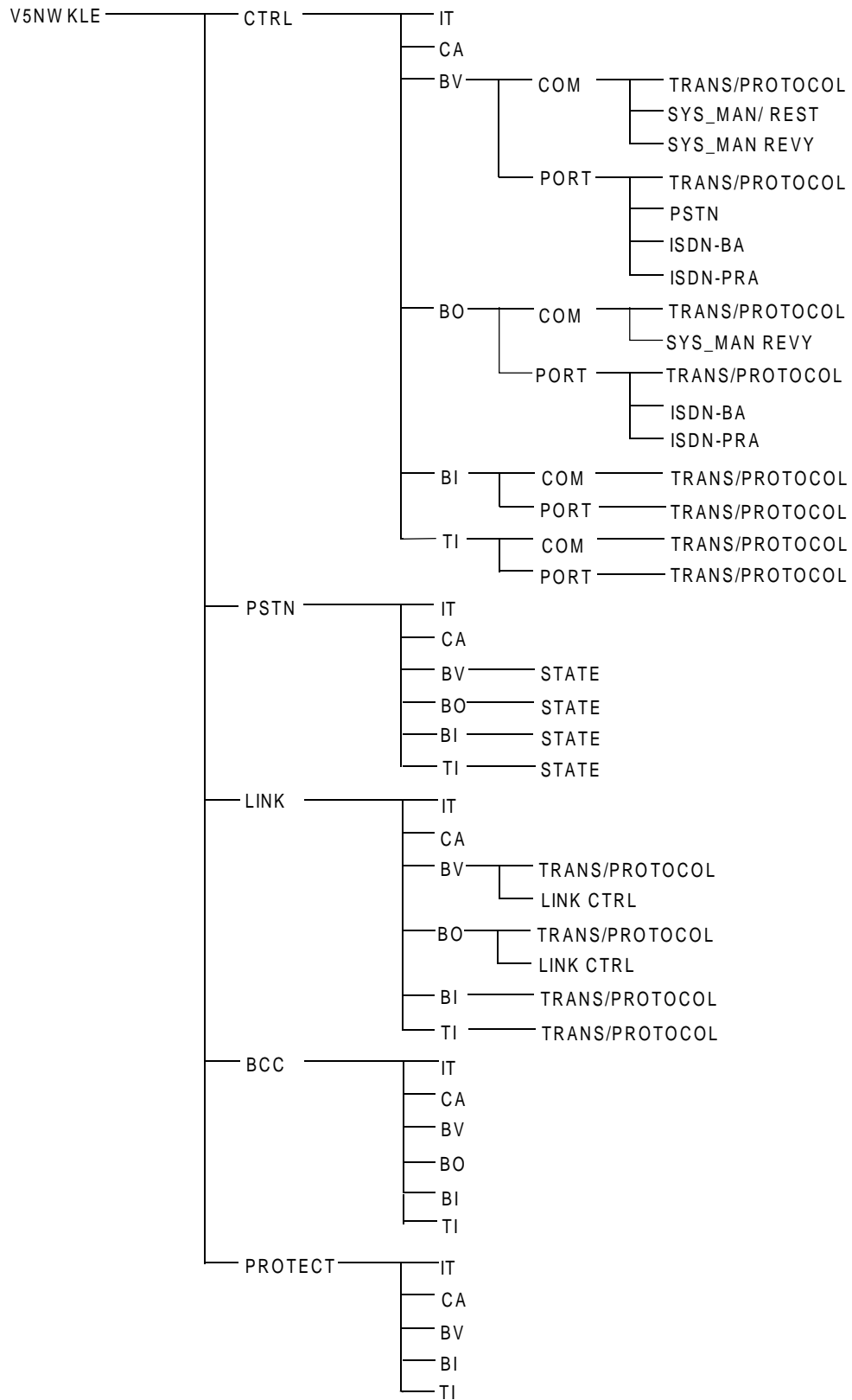
Figure 1: Network Layer LE test suite structure
