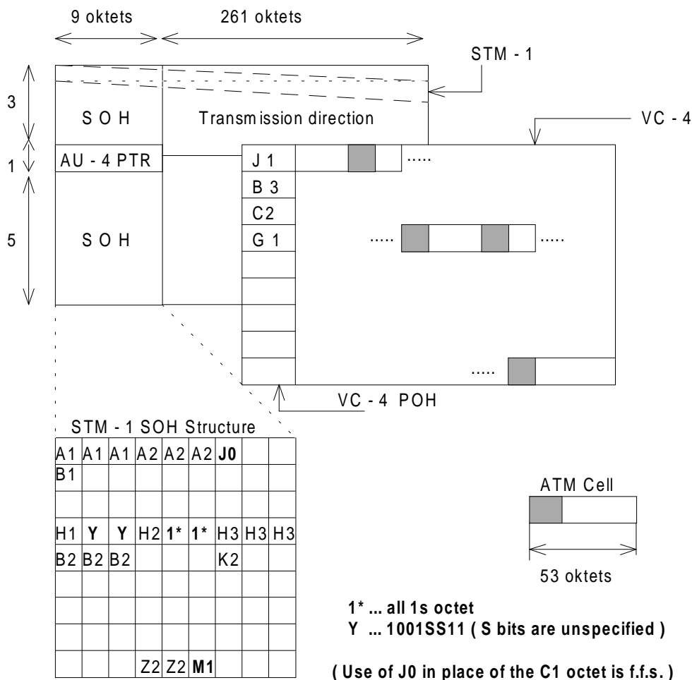
Figure 10: 155 520 kbit/s frame structure
