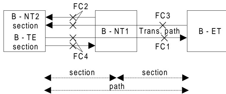
Figure 16: Fault conditions and operational span of section path maintenance signals
