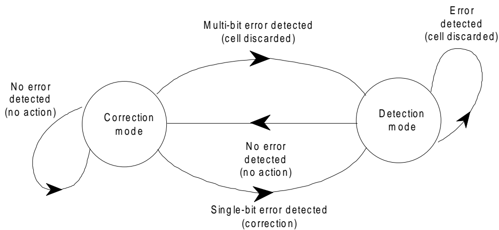
Figure 13: Header Error Control (HEC) - receiver modes of operation
