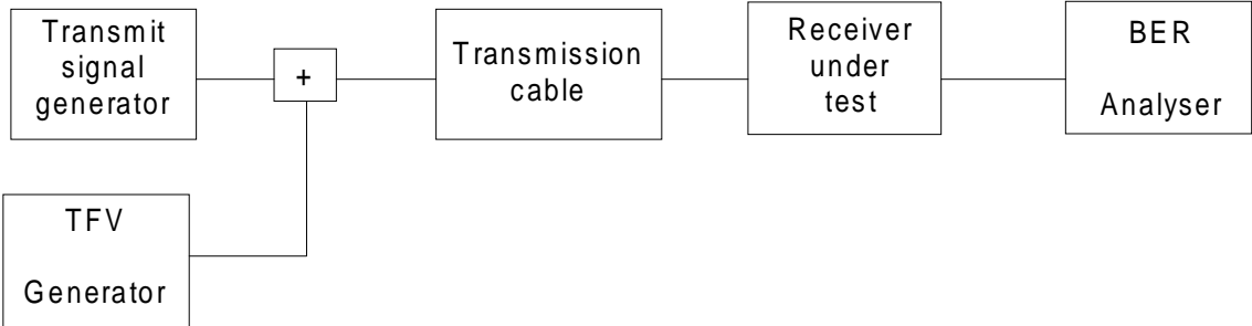
Figure 8: Measurement configuration
