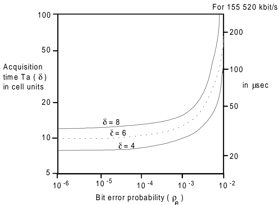
Figure A.2: Acquisition time vs. bit error probability ( T_a(\delta) vs. \rho_e )
