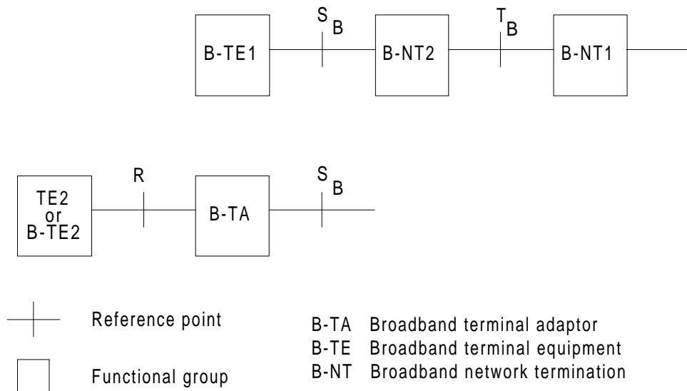
Figure 1: B-ISDN reference configurations
