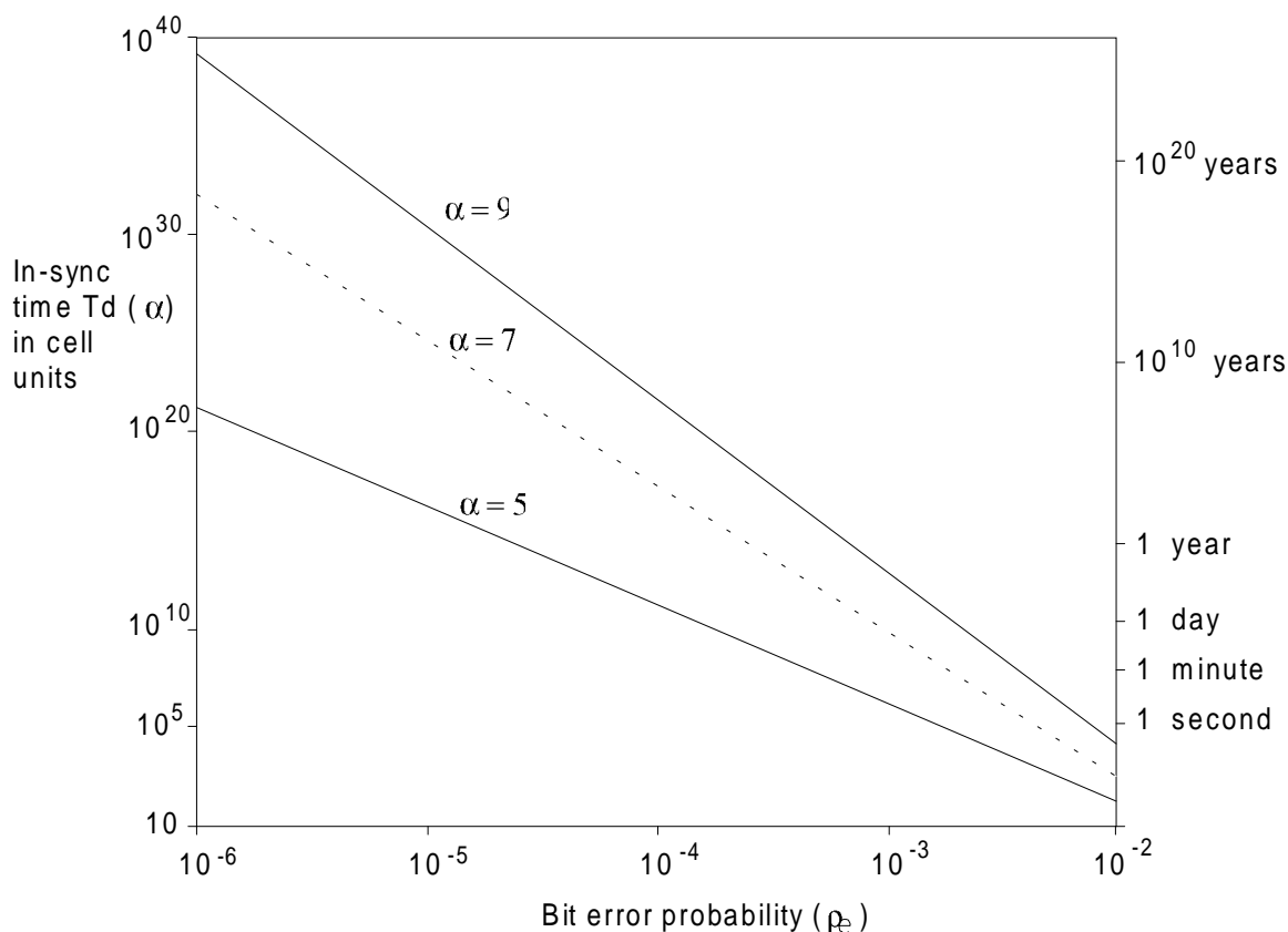
Figure A.1: In-sync time vs. bit error probability ( T_d(\alpha) vs. r_e )
