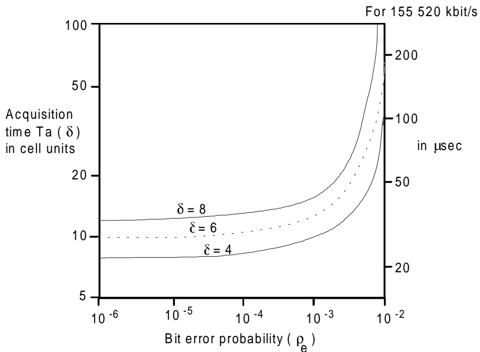
Figure A.2: Acquisition time vs. bit error probability ( T_a(\delta) vs. r_e )
