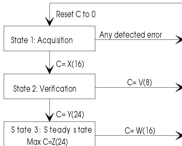
Figure 12: State transition diagram
