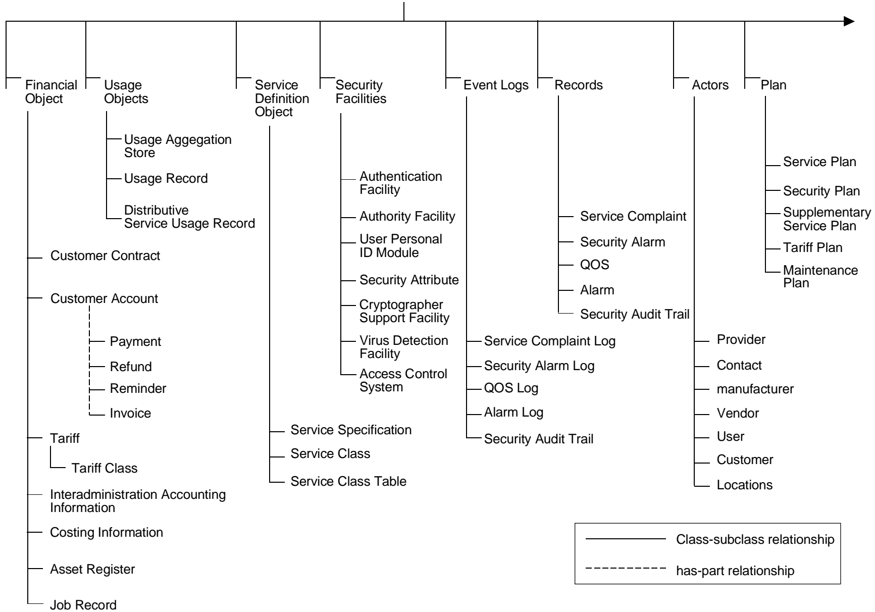
Figure D.1 : Service level object hierarchy
