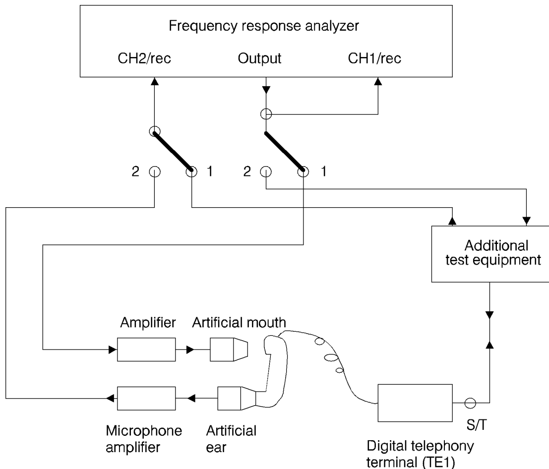
Figure A.2: Configuration for delay measurement
