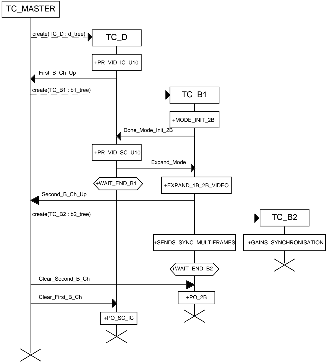
Figure 3: Example of an exchange of co-ordination messages
