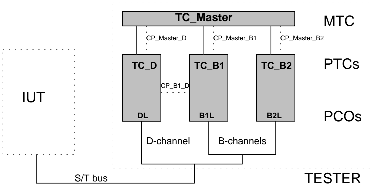
Figure 1: Multi-party test method
