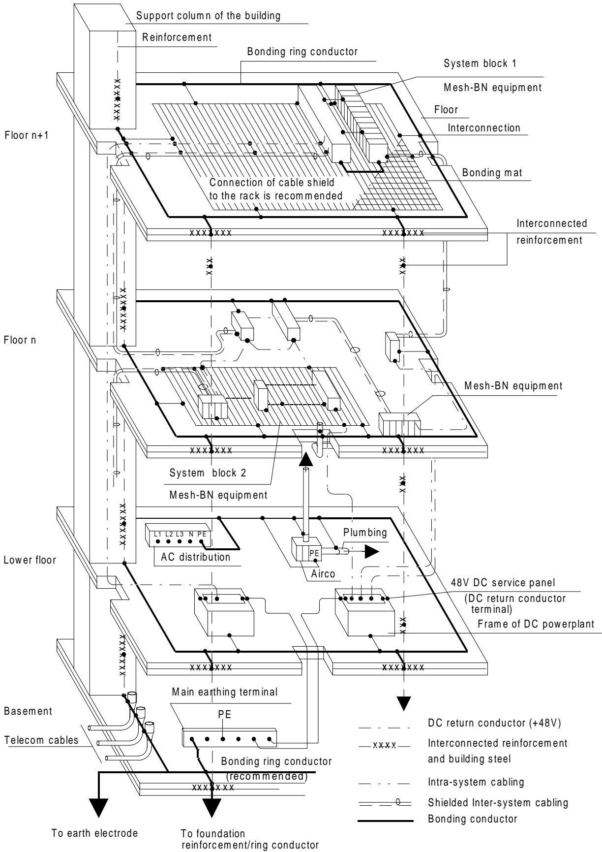
Figure 1: CBN/MESH-BN installation inside a telecommunication building
