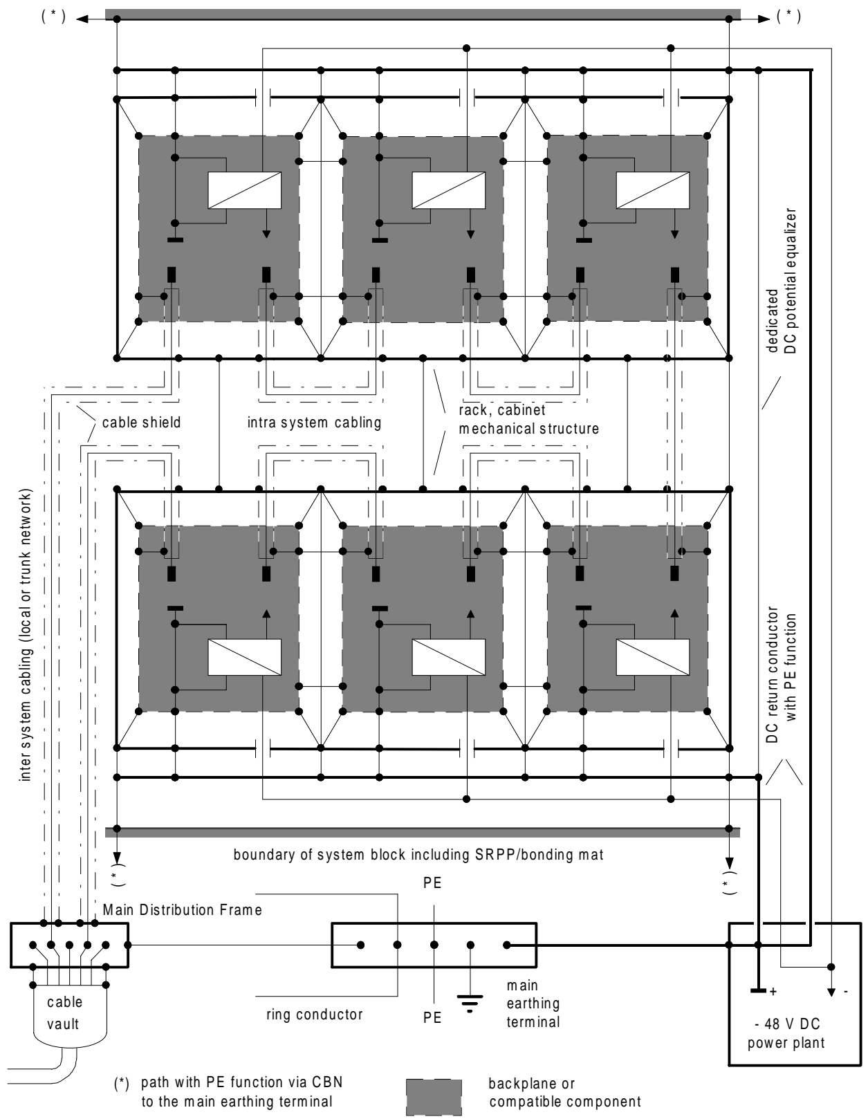
Figure 2: Example of a system block installation with an overall CBN/MESH-BN configuration
