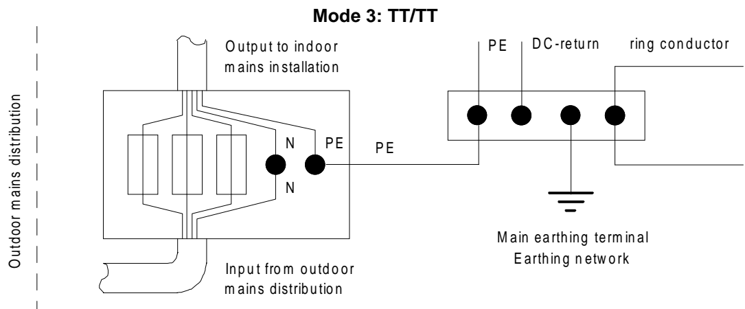
Figure 4: Arrangements for the transition from the outdoor mains distribution network to the indoor mains installation
