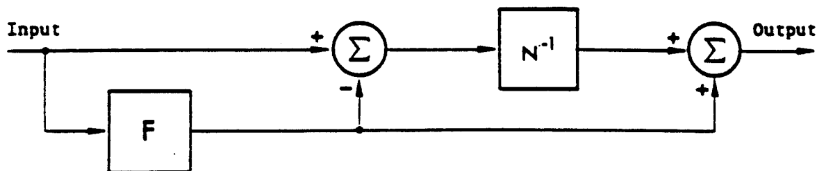
Fig. 4: The de-emphasis network of Fig. 3
