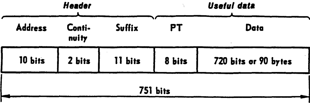
Fig. 1: Packet structure
