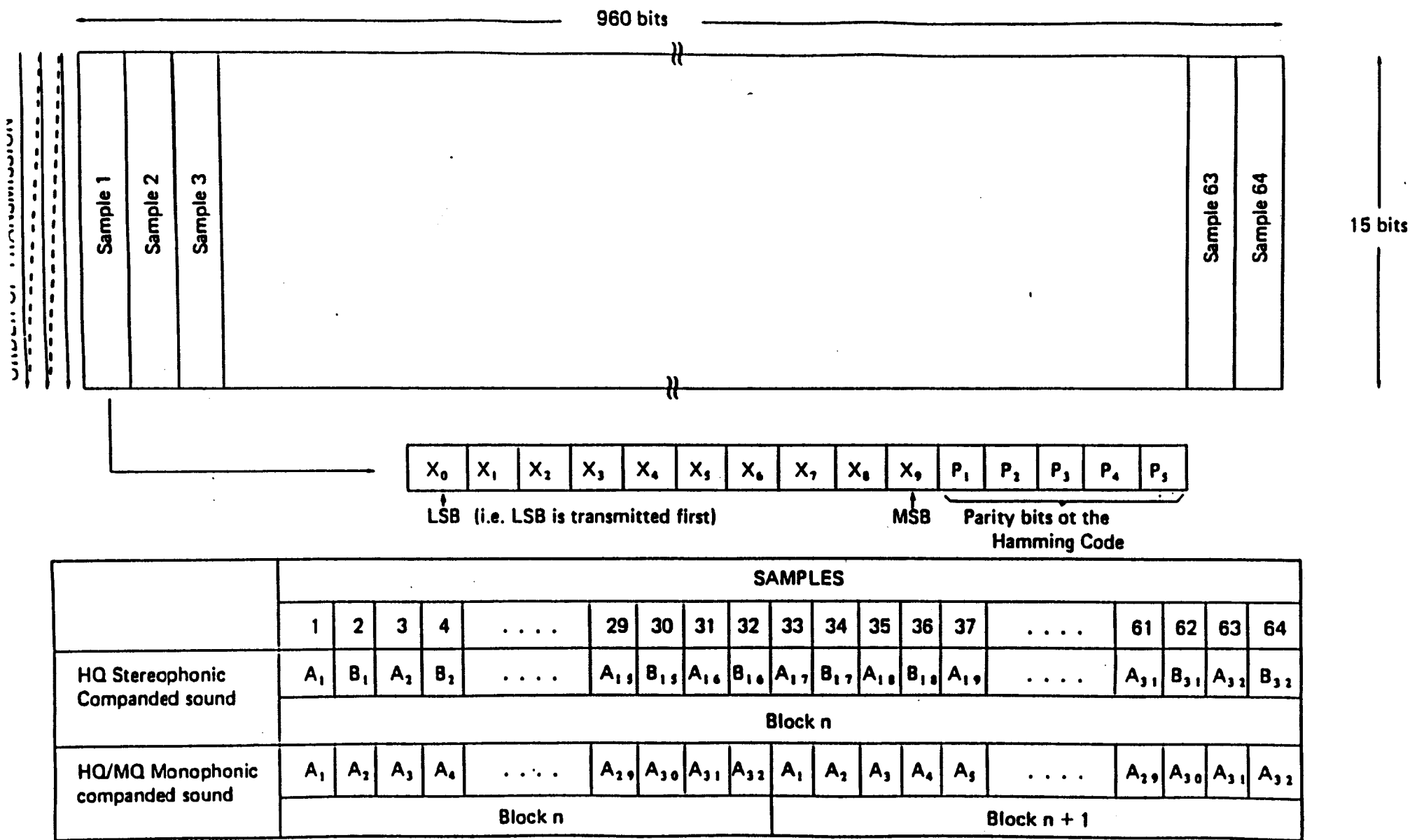
Fig. 4d: Arrangement of 120-byte COMPANDED sound coding blocks in relation with the SECOND-LEVEL PROTECTION
