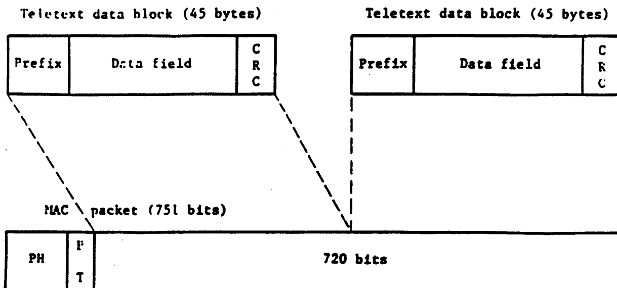
Fig. 2a: First-level protection
