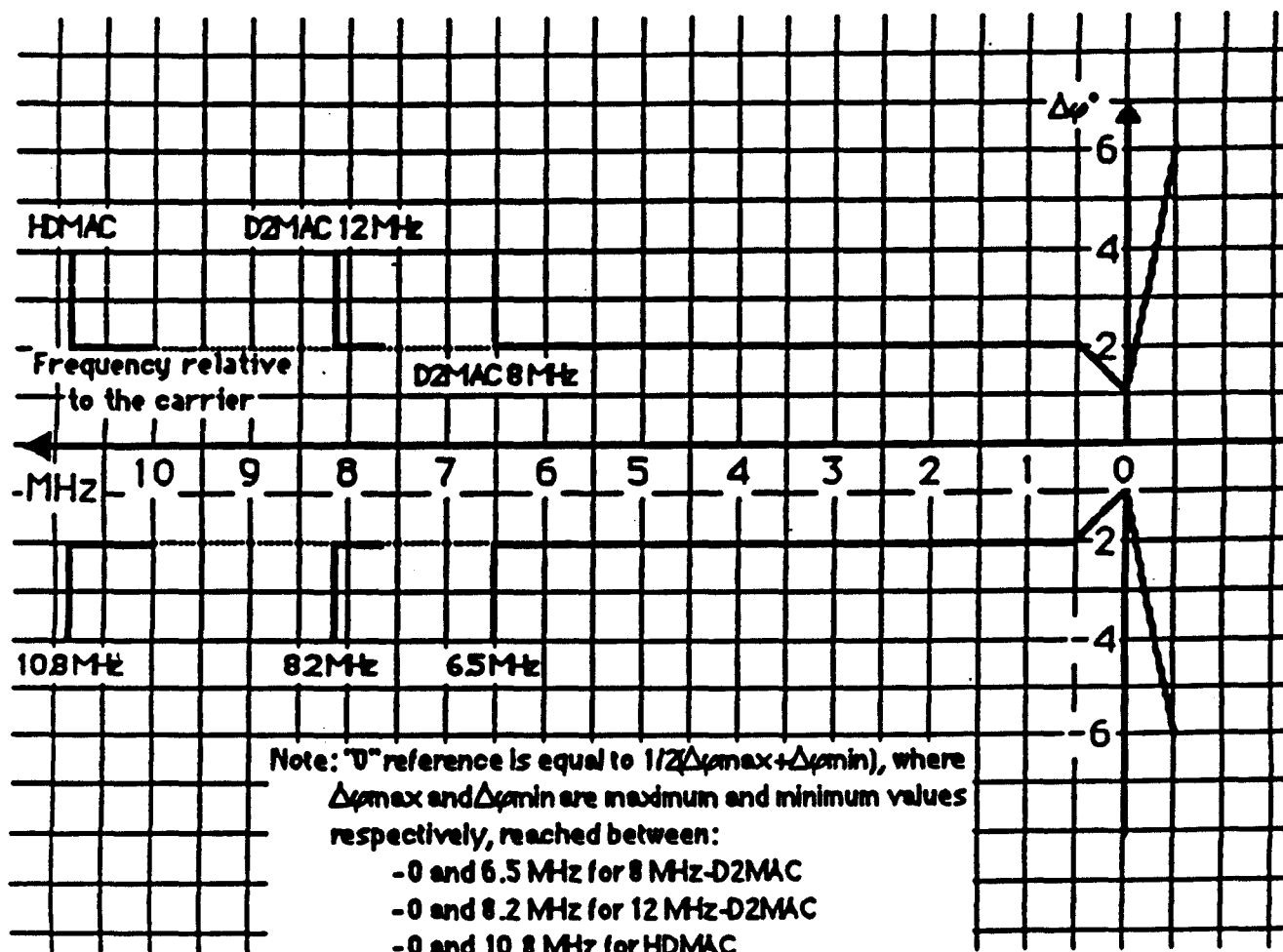
Fig.4: Phase/frequency template for the transmitter filtering
