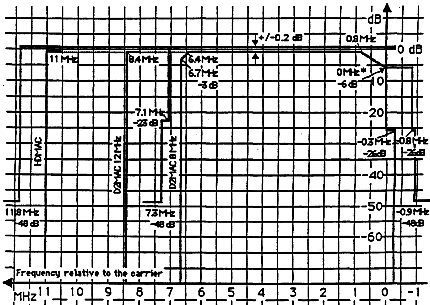
Fig. 3: Amplitude/frequency template for the transmitter filtering
