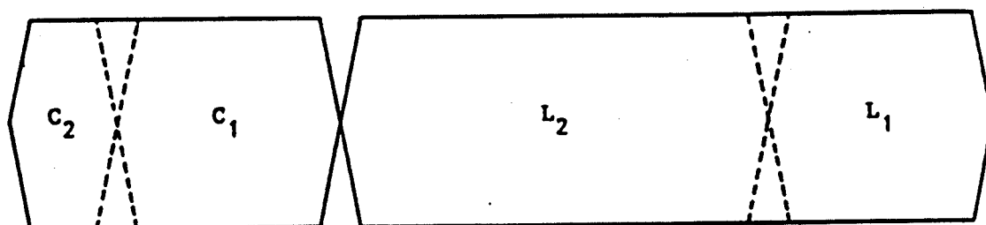
Fig. 4b: Simplified diagram of waveform scrambled by double-cut component rotation
