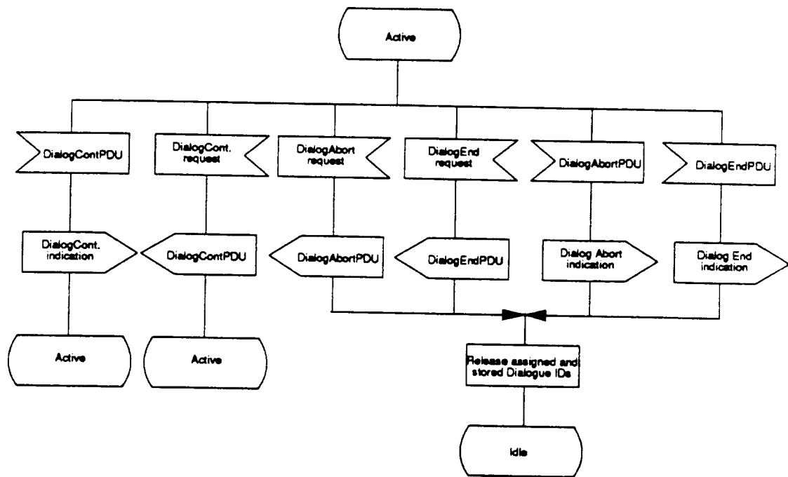
Figure 10 - Dialogue procedures dynamic description (sheet 4 of 4)
