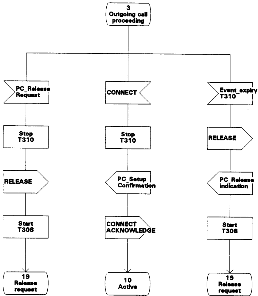
Figure 7 - Connection oriented Protocol Control SDL (sheet 4 of 10)
