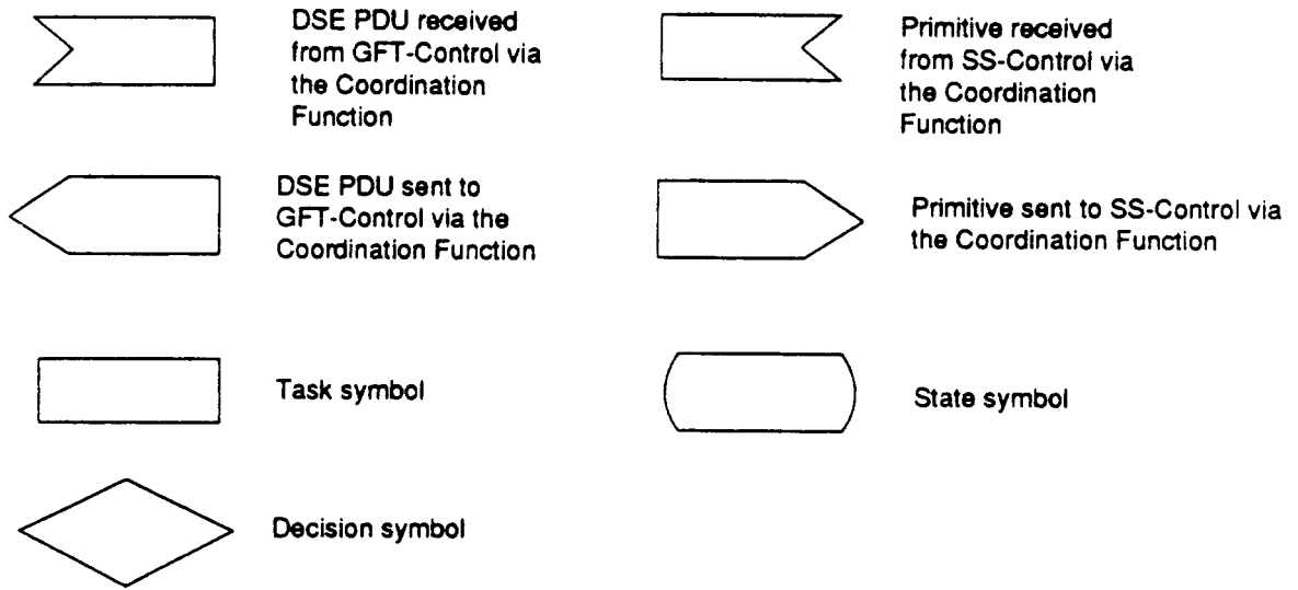
Figure 9 - Key to Dialogue SDL diagram in figure 10
