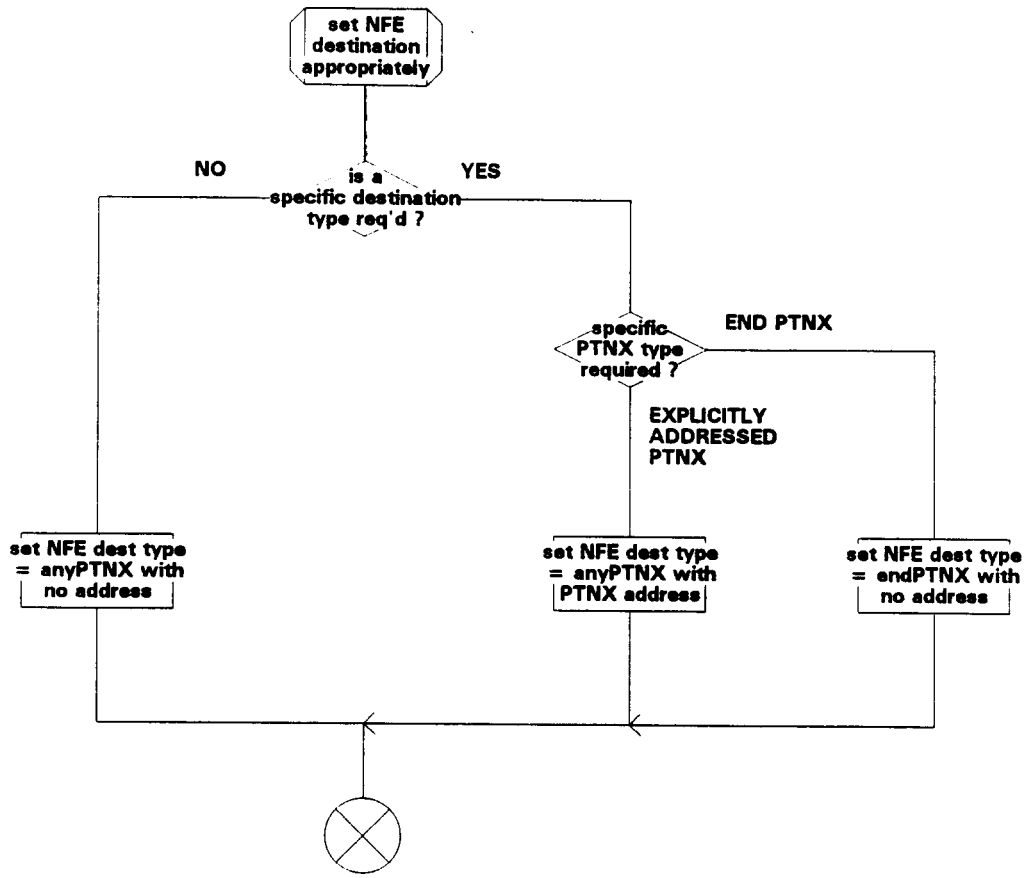
Figure 4 - Actions at a Source PTNX (sheet 2 of 2)
