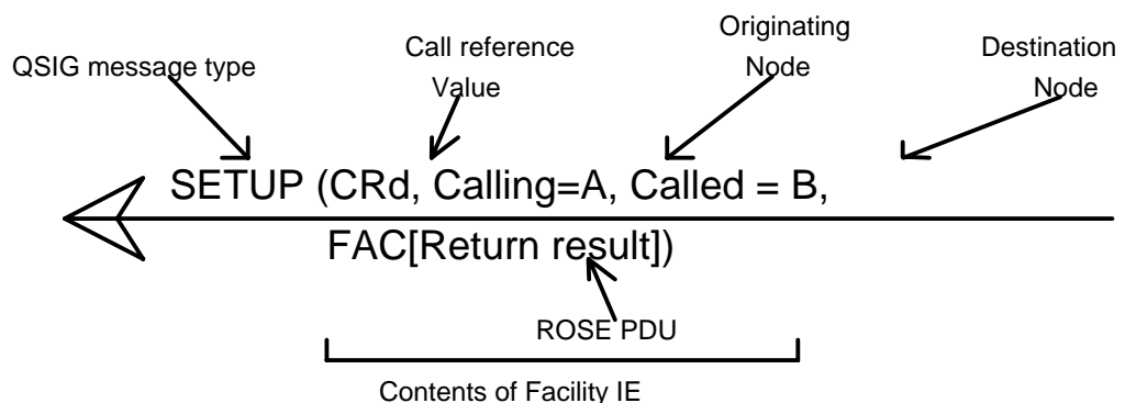
Figure A.11 - Notation for Connection oriented Call independent message sequence examples
