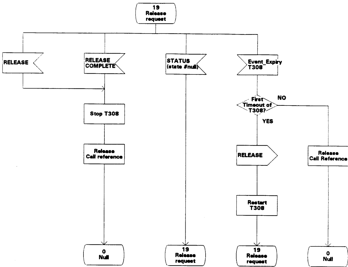
Figure 7 - Connection oriented Protocol Control SDL (sheet 8 of 10)
