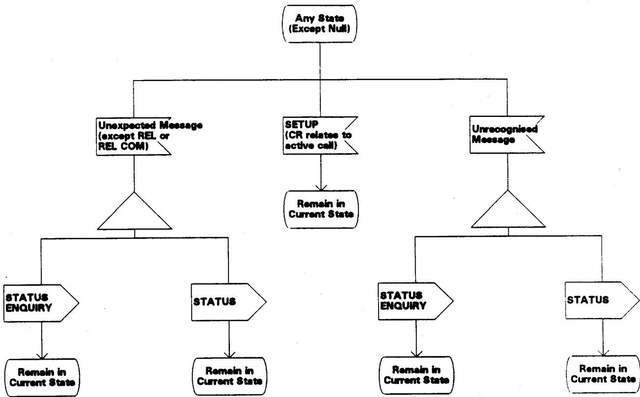
Figure 7 - Connection oriented Protocol Control SDL (sheet 10 of 10)
