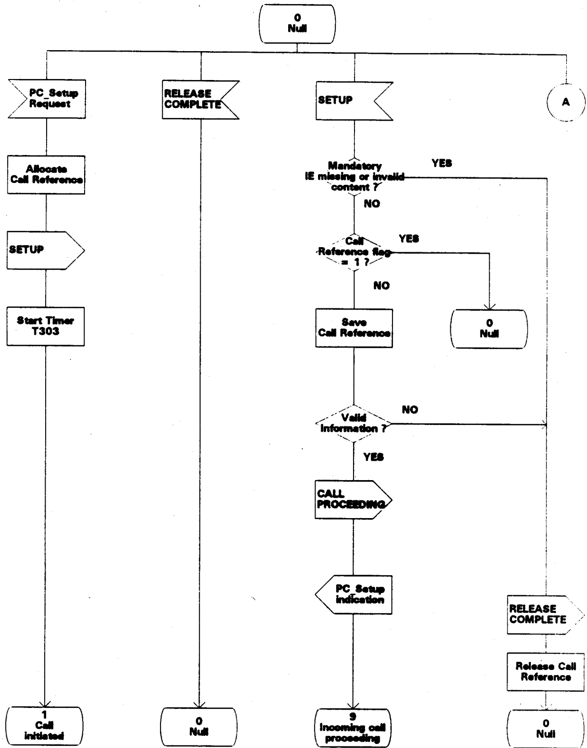
Figure 7 - Connection oriented Protocol Control SDL (sheet 1 of 10)
