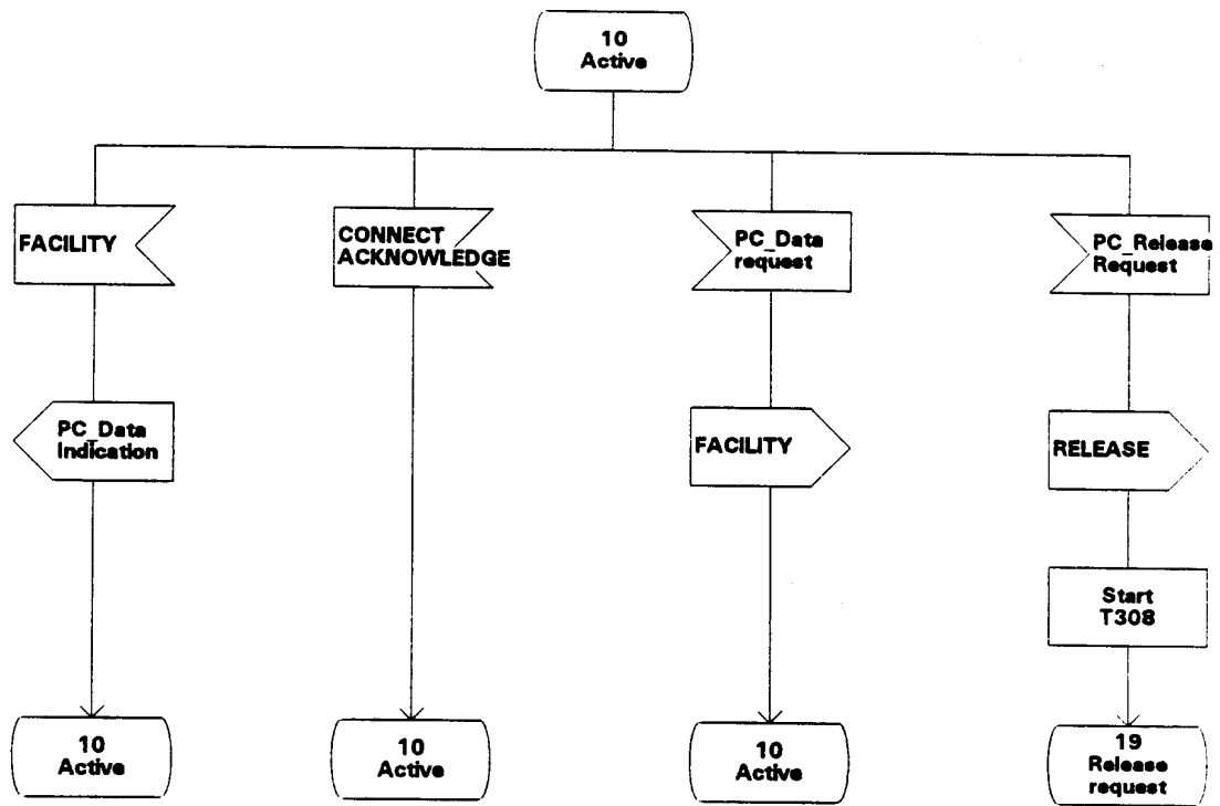
Figure 7 - Connection oriented Protocol Control SDL (sheet 6 of 10)
