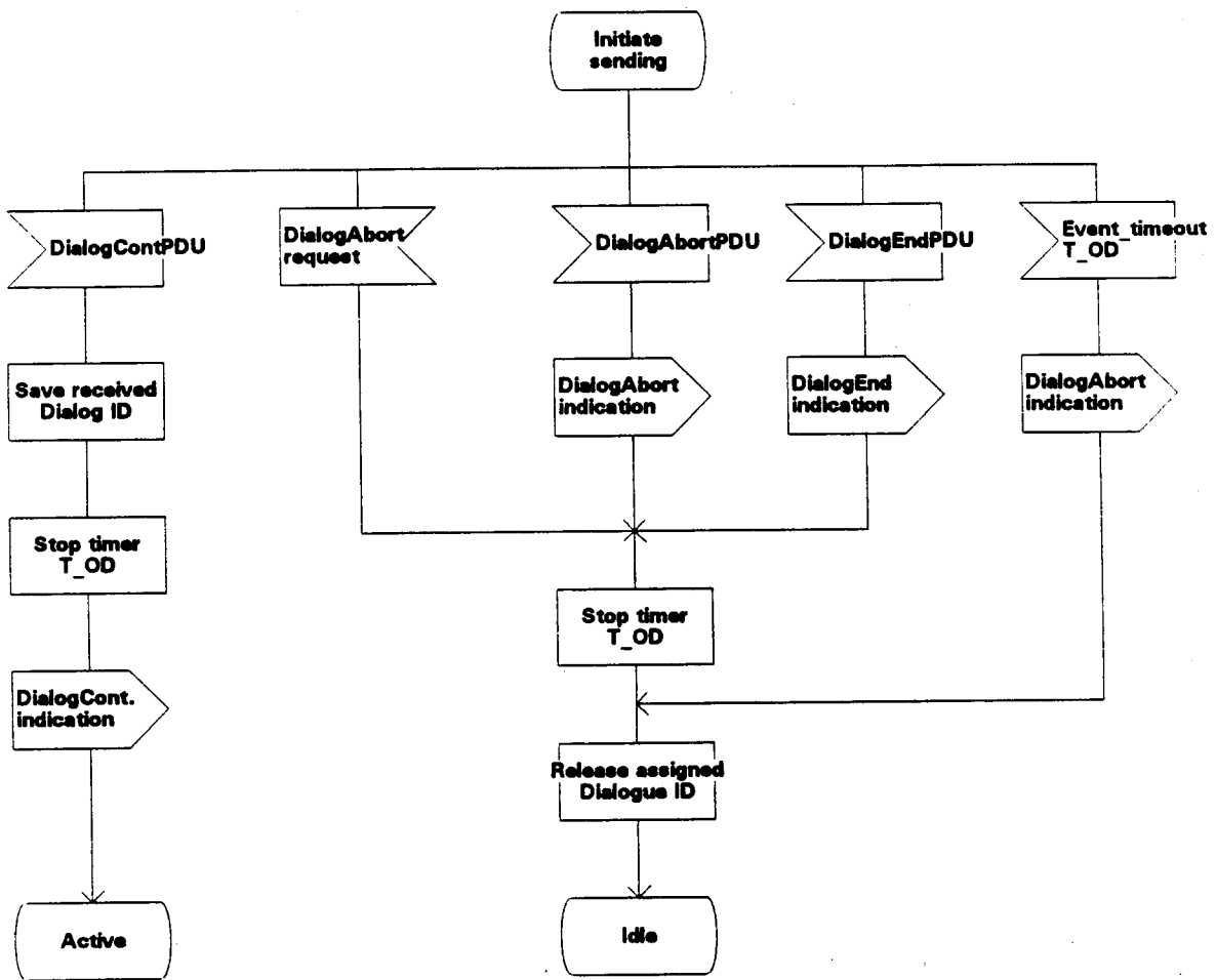
Figure 10 - Dialogue procedures dynamic description (sheet 3 of 4)
