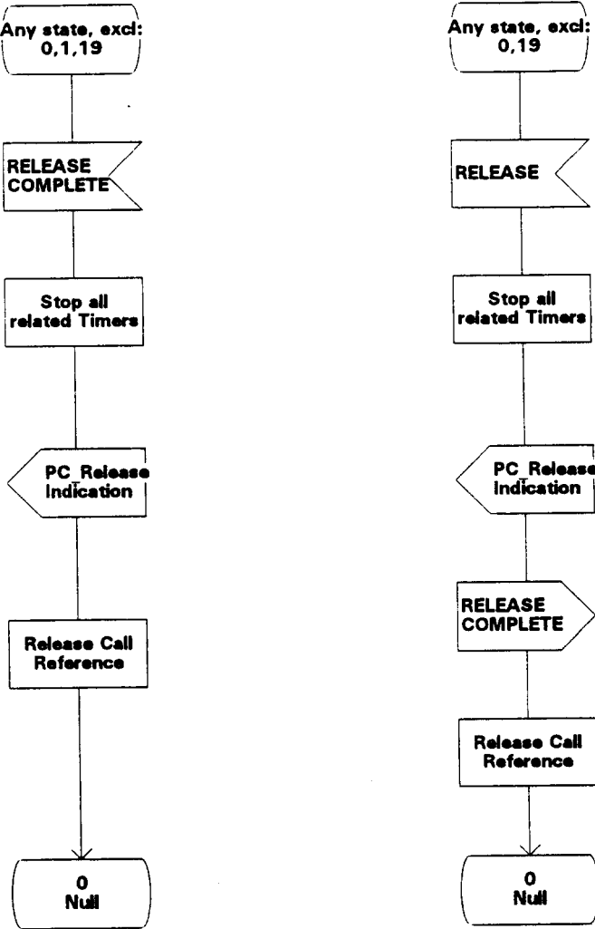
Figure 7 - Connection oriented Protocol Control SDL (sheet 9 of 10)
