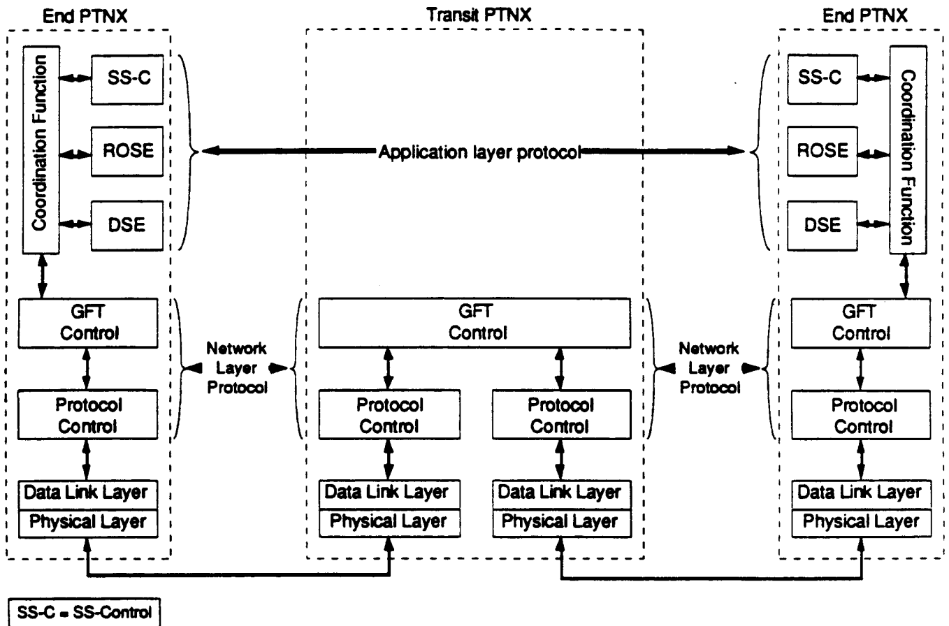
Figure 2 - Application of the protocol model to communication between non-Adjacent PTNXs
