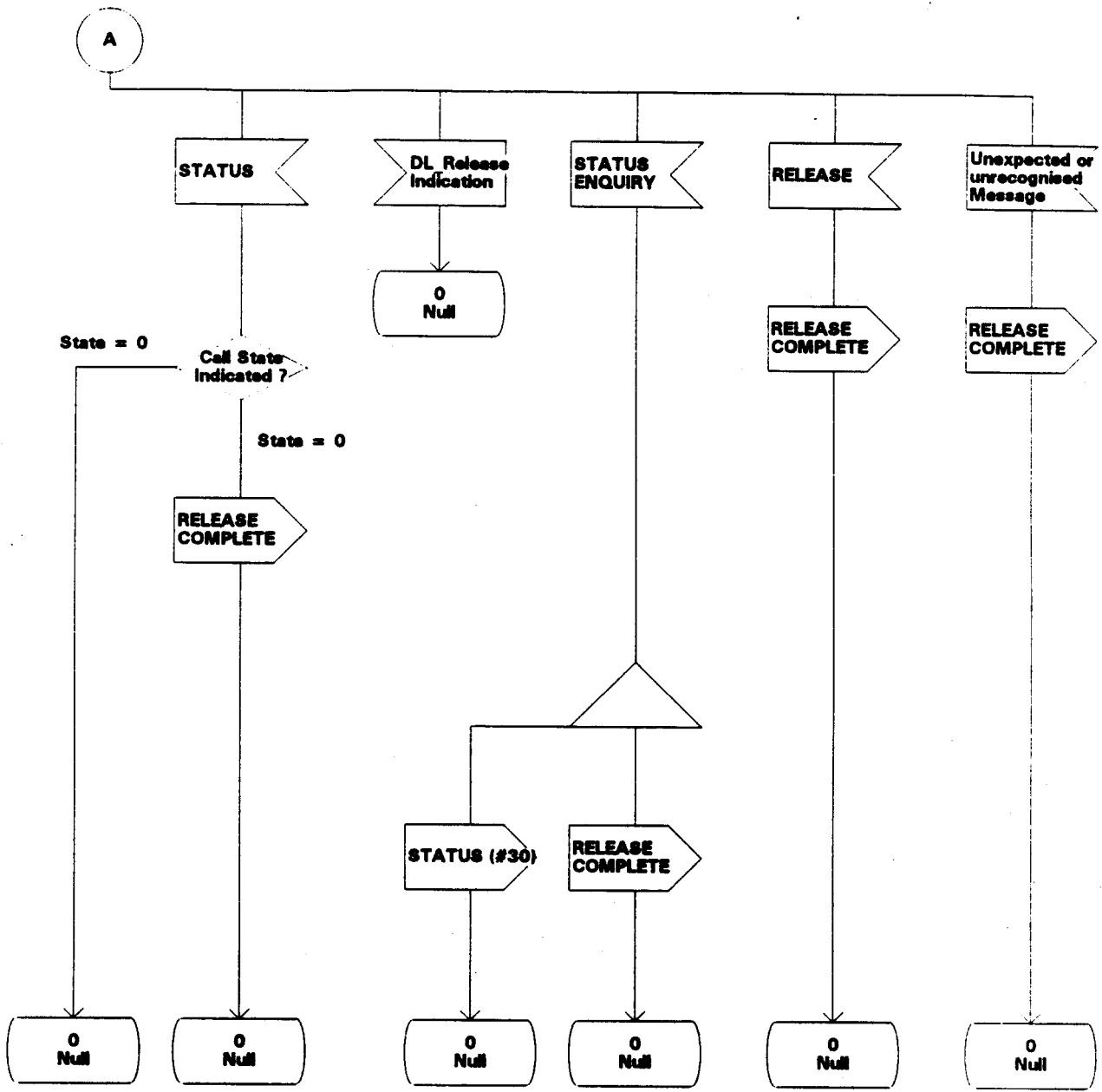
Figure 7 - Connection oriented Protocol Control SDL (sheet 2 of 10)
