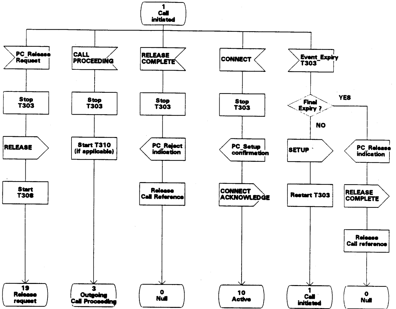
Figure 7 - Connection oriented Protocol Control SDL (sheet 3 of 10)
