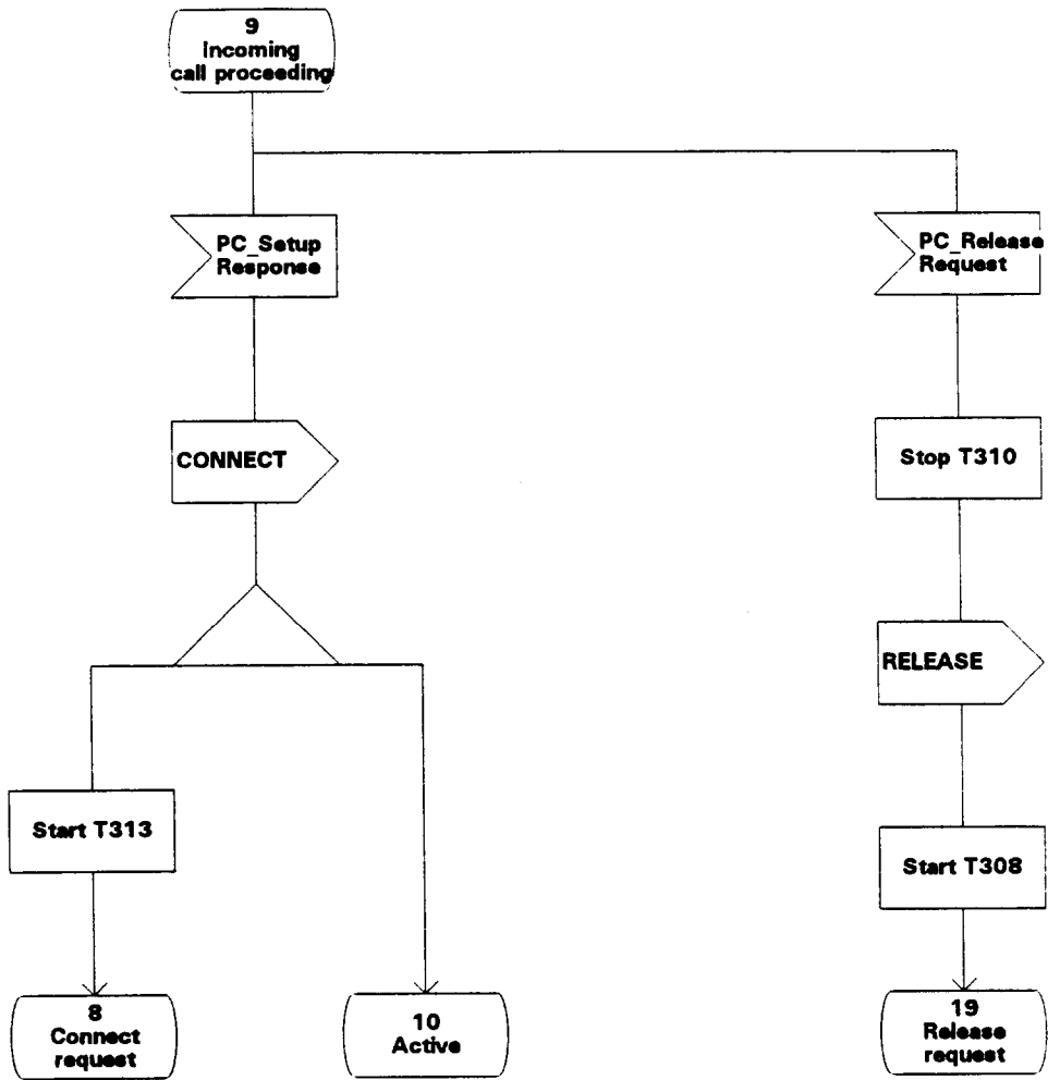
Figure 7 - Connection oriented Protocol Control SDL (sheet 7 of 10)
