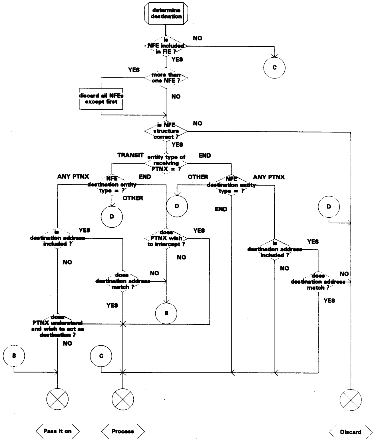
Figure 5 - Actions at a Receiving PTNX (sheet 2 of 2)
