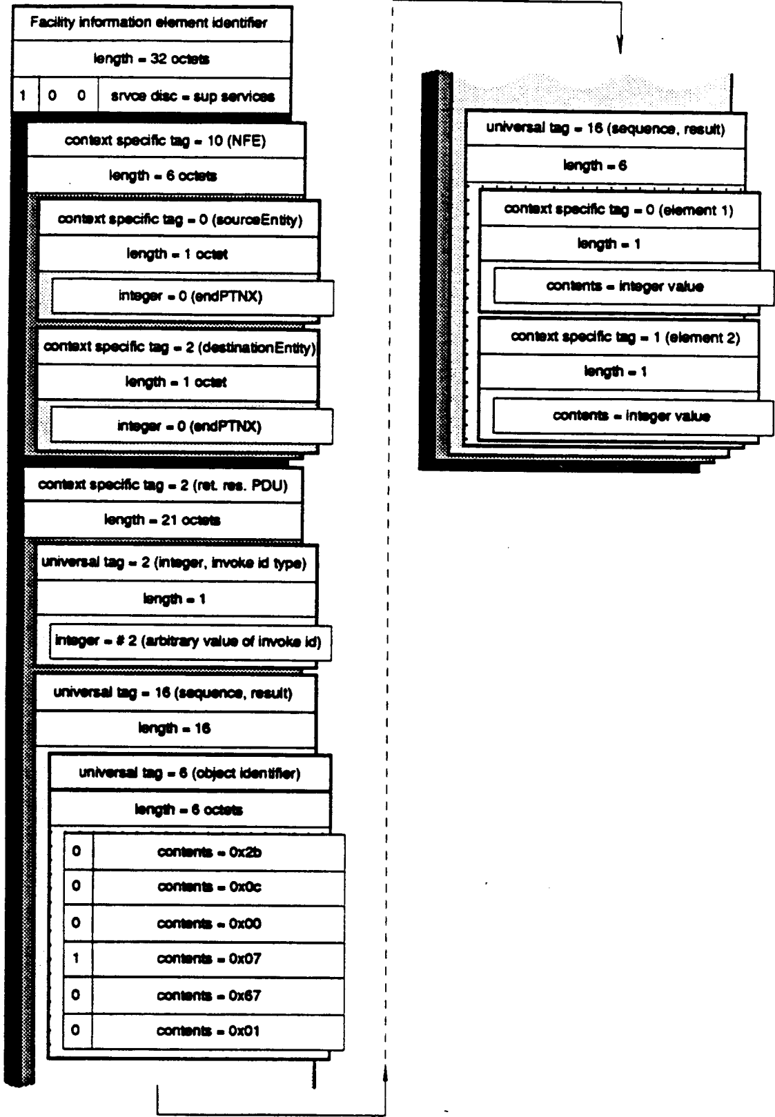
Figure A.5 - Encoding of ReturnResultPDU from ALERTING message of figure A.2
