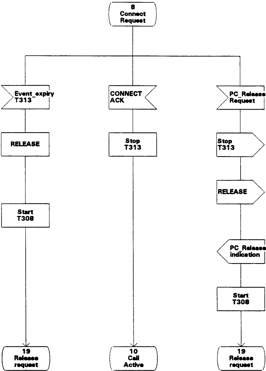
Figure 7 - Connection oriented Protocol Control SDL (sheet 5 of 10)
