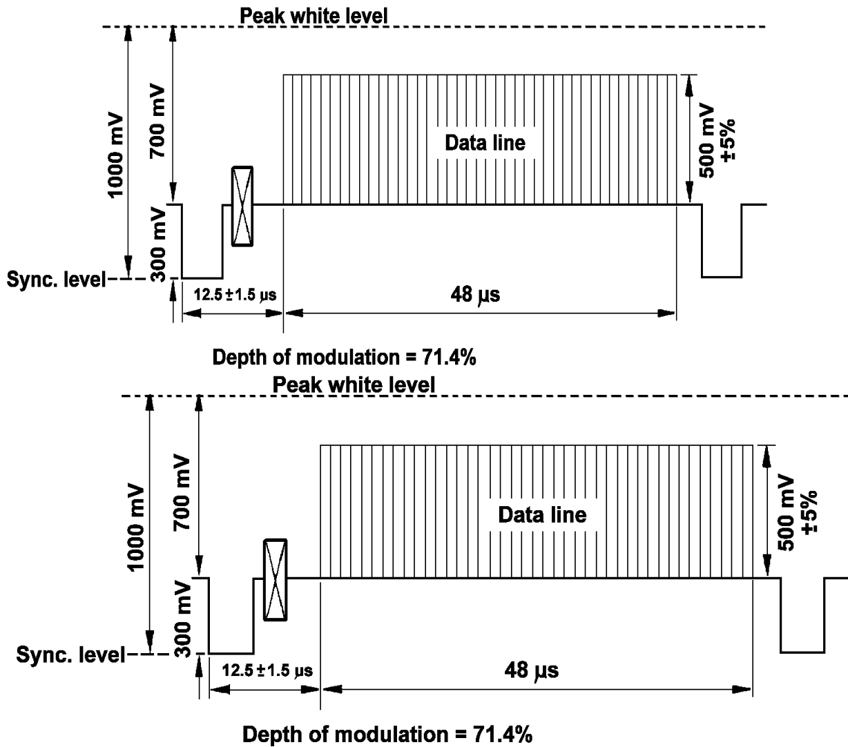
Figure 8: Insertion of the data line into the video signal
